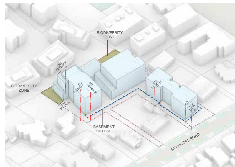
Building Setbacks and Separation
