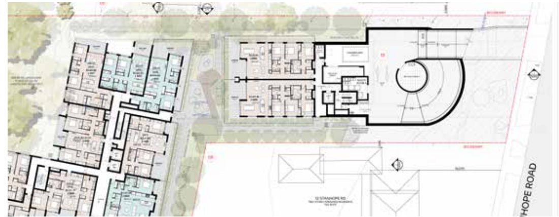
Lower Ground 1 - Loading bay
