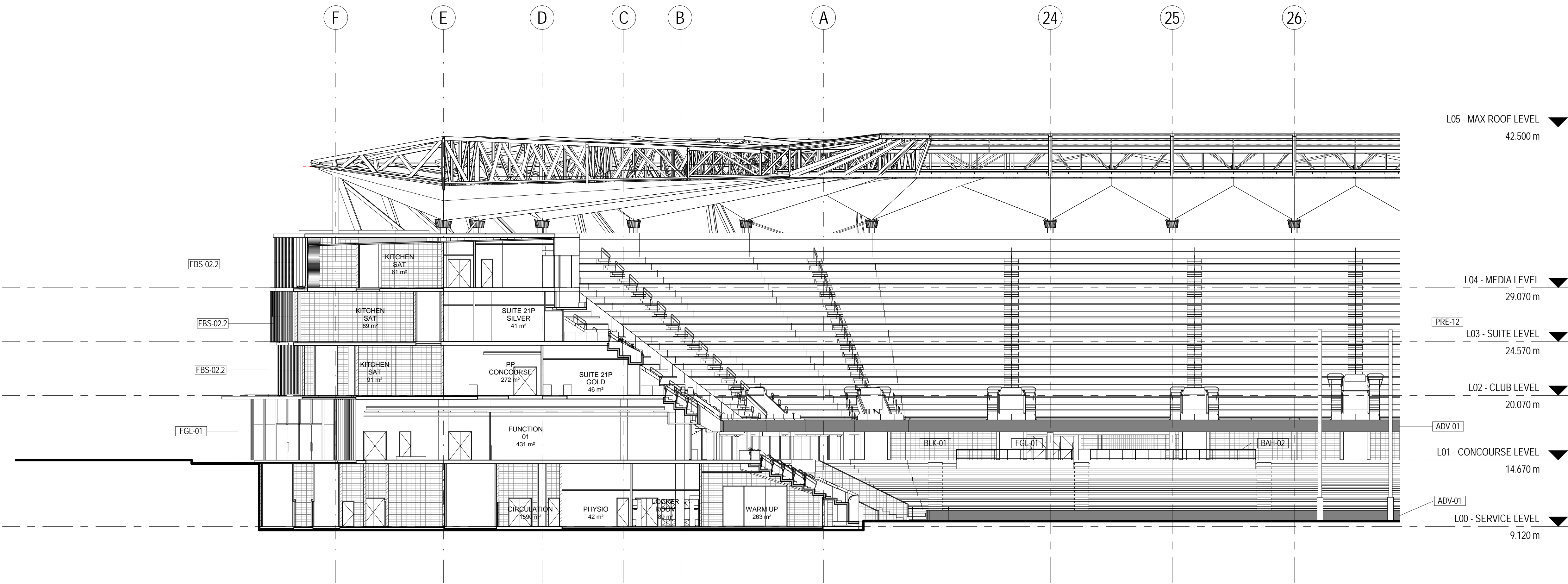
2 GA SECTION - PART WEST 1 : 200
