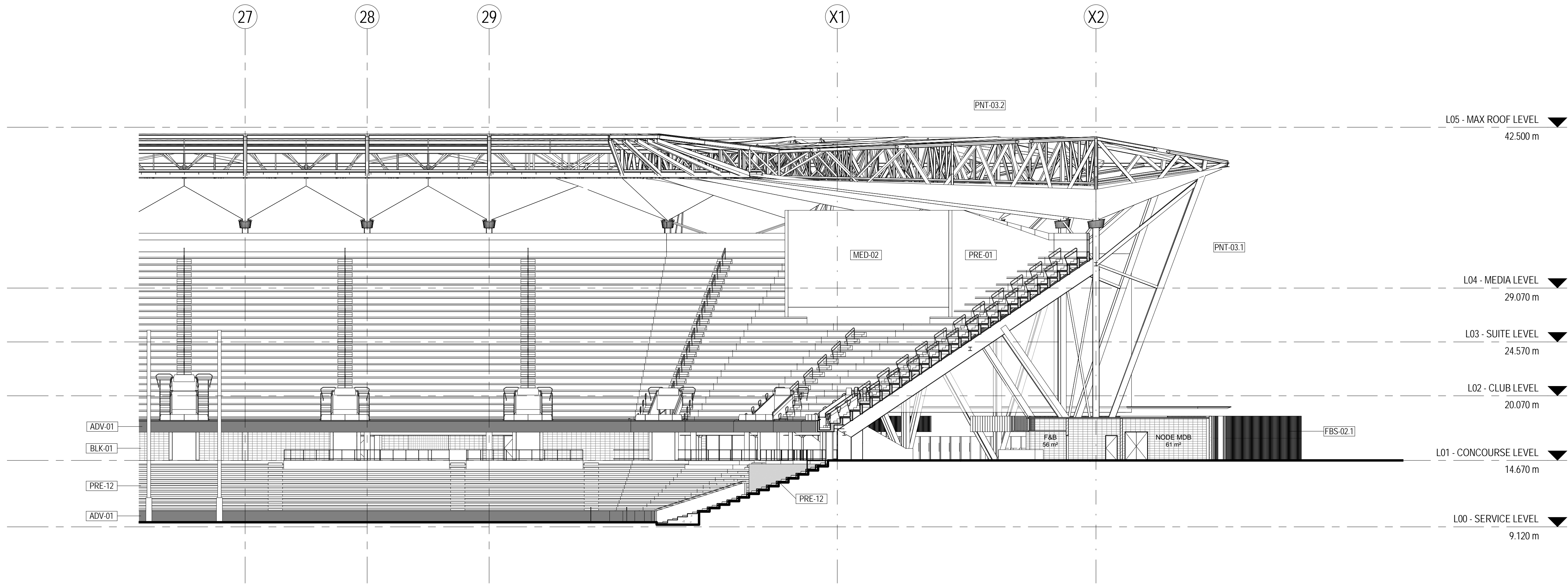
1 GA SECTION - PART EAST 1 : 200
