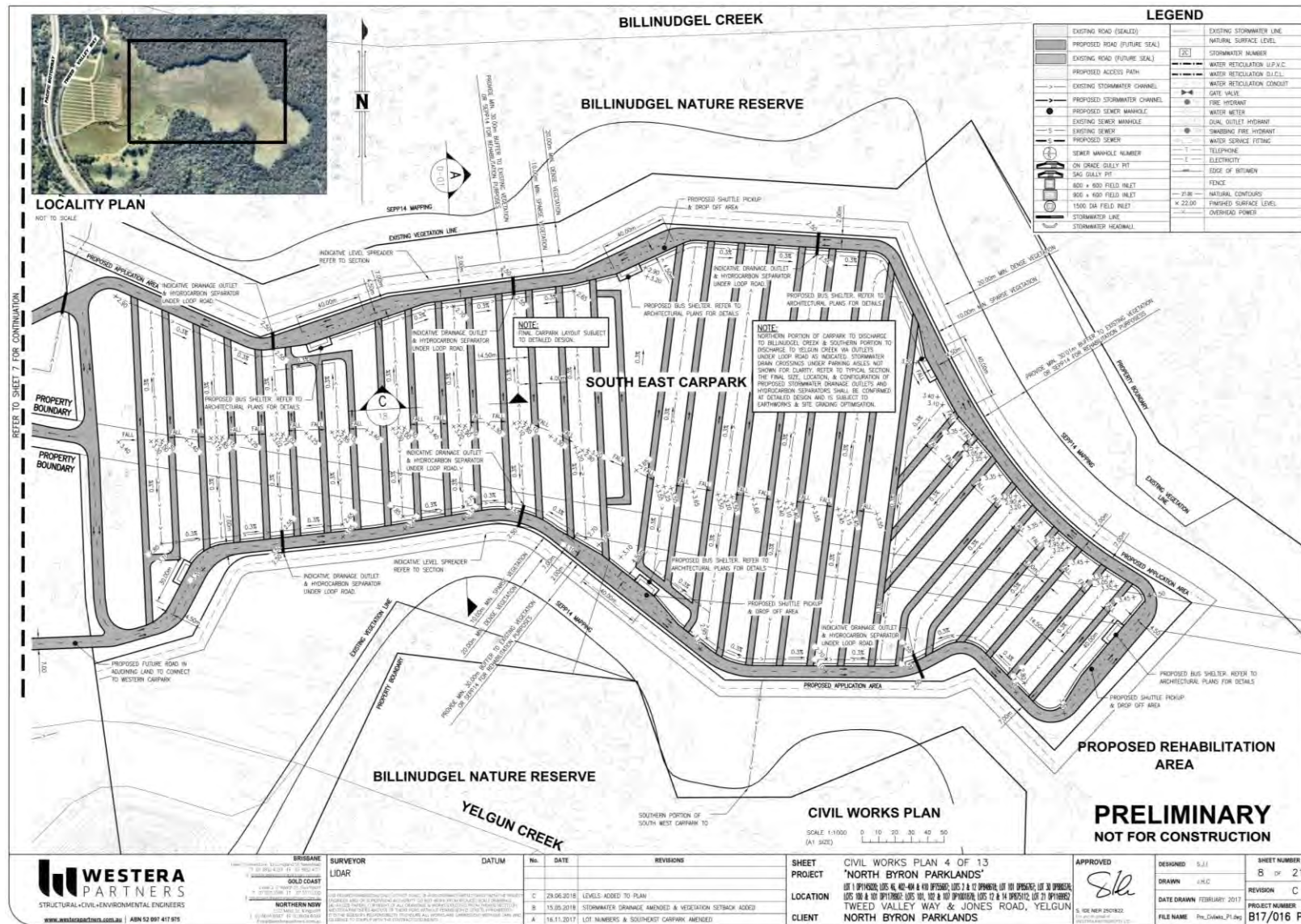
Figure 9: Southern Carpark Civil Works Plan (Preliminary Design)
