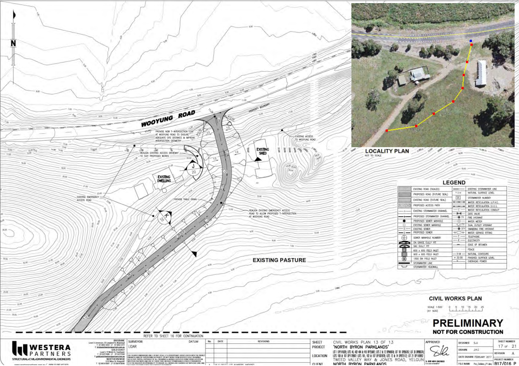
Figure 10: Proposed Northern Access Road Intersection Re-Alignment
