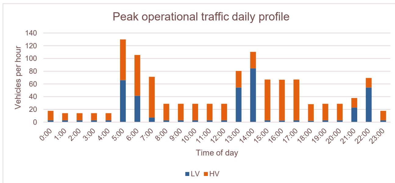
Figure 5-1 Peak operational daily traffic profile - Storage and Distribution warehouse
