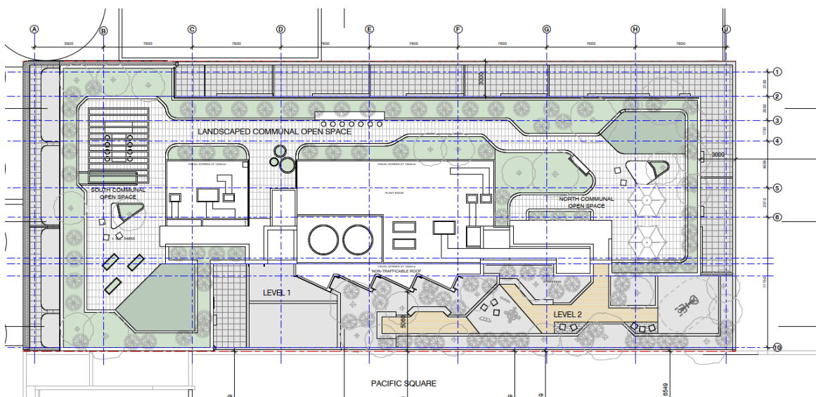
Figure 4 Roof Level Landscaping
