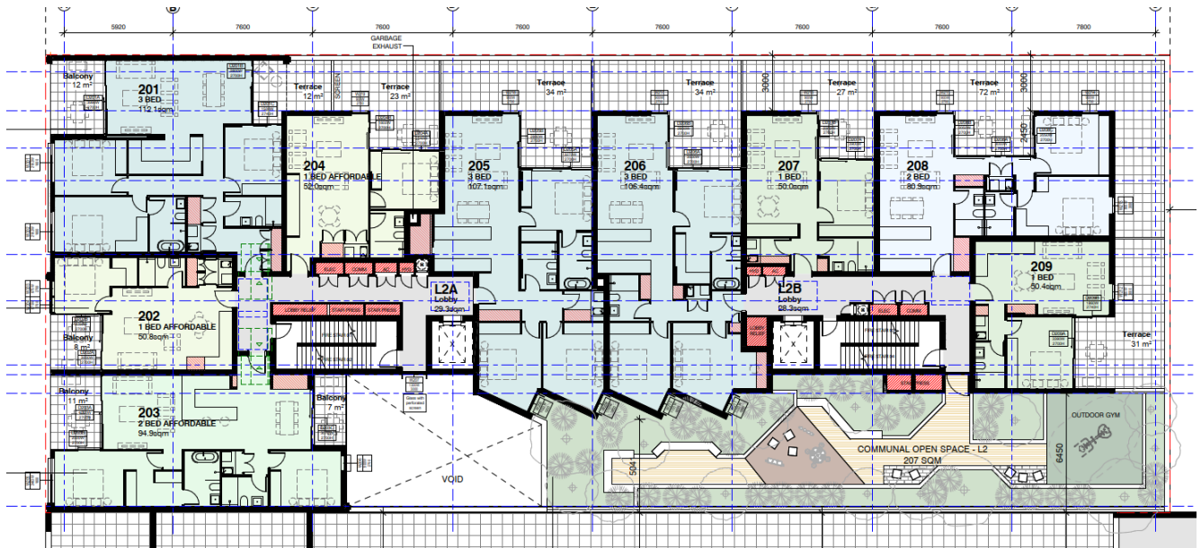
Figure 2 Level 2 Plan
