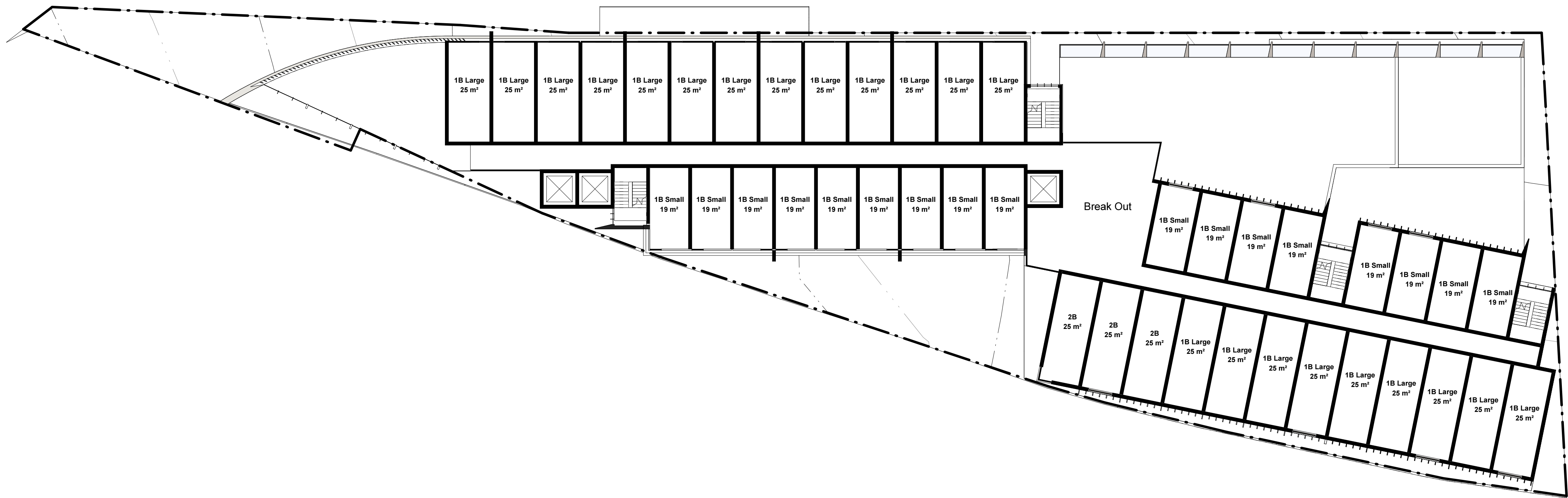
TYPICAL PLAN
