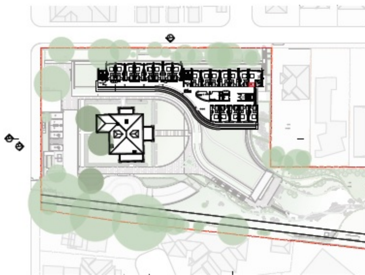
Revised Layout Plans in response to Community Consultation No. 01 Level 2
