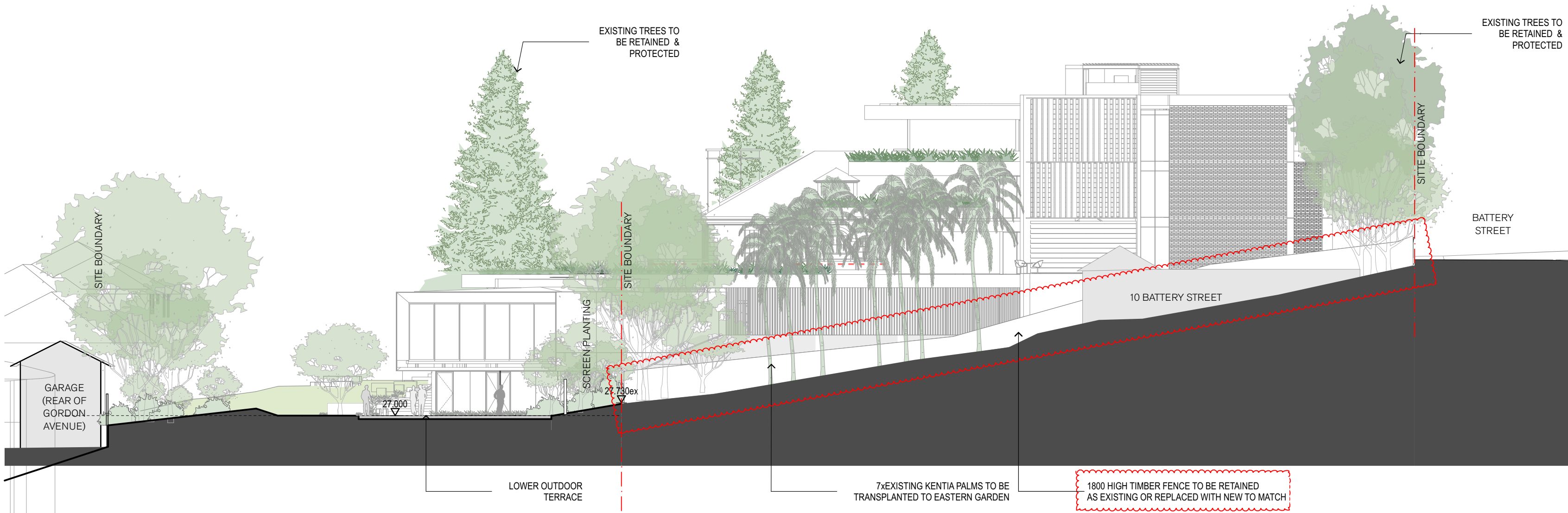
Section L1
