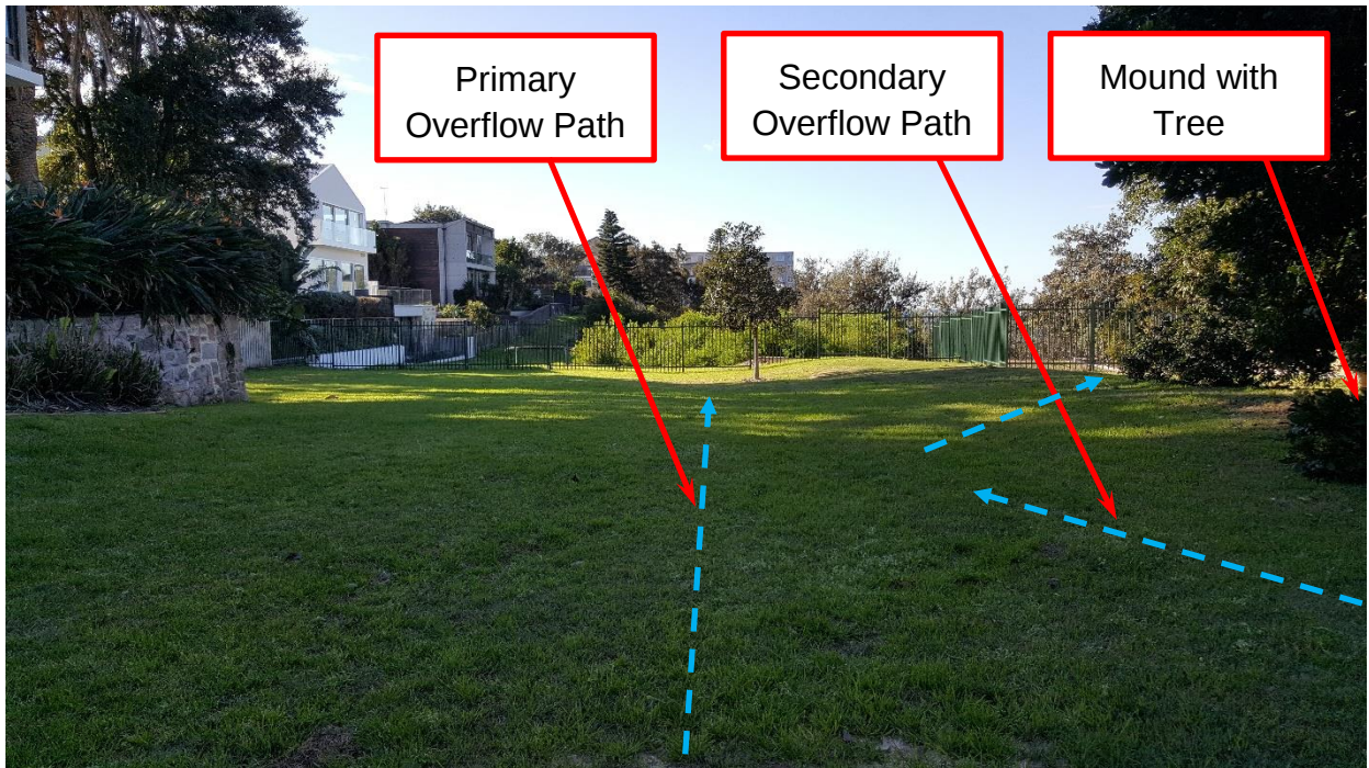
Figure 19 – Eastern view of mound and overflow paths
