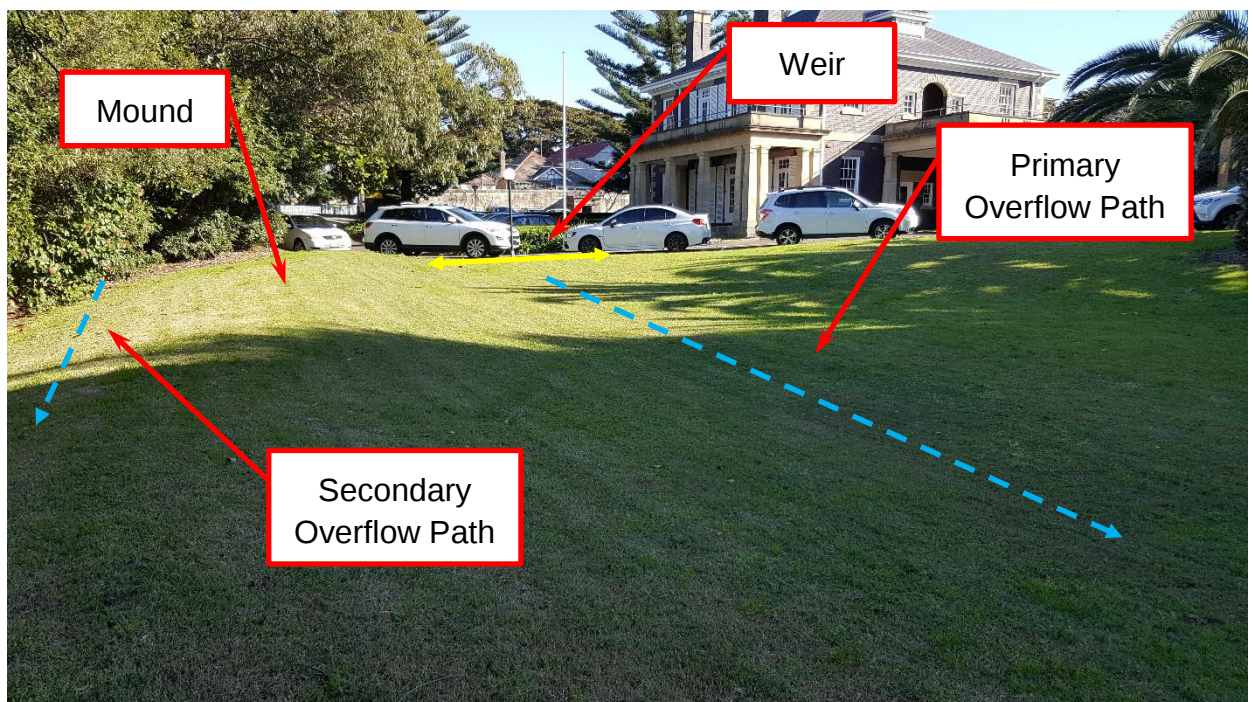
Figure 18 – Western view of overland flow weir, mound and overflow paths
