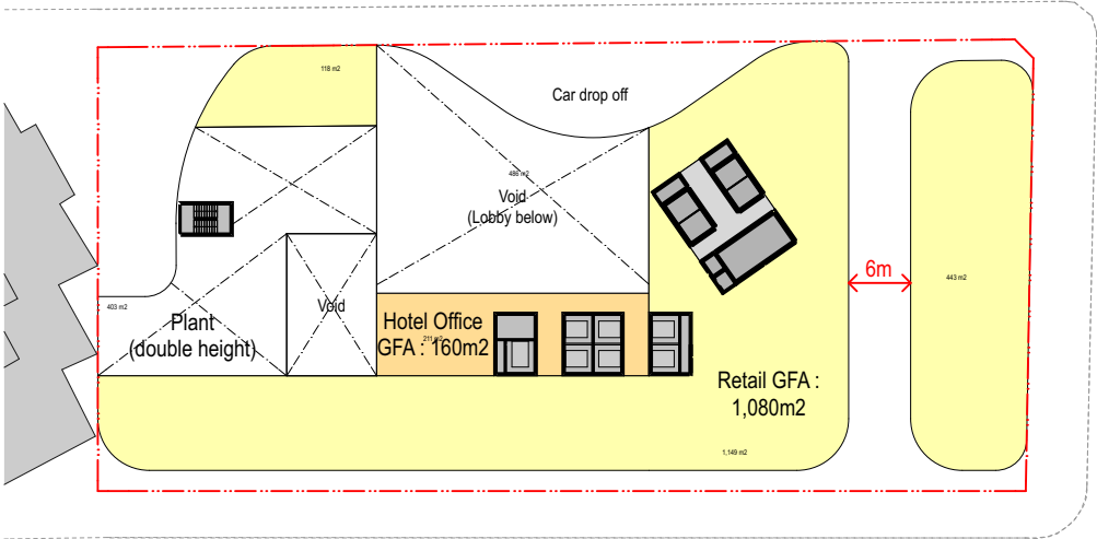
Mezzanine Floor
