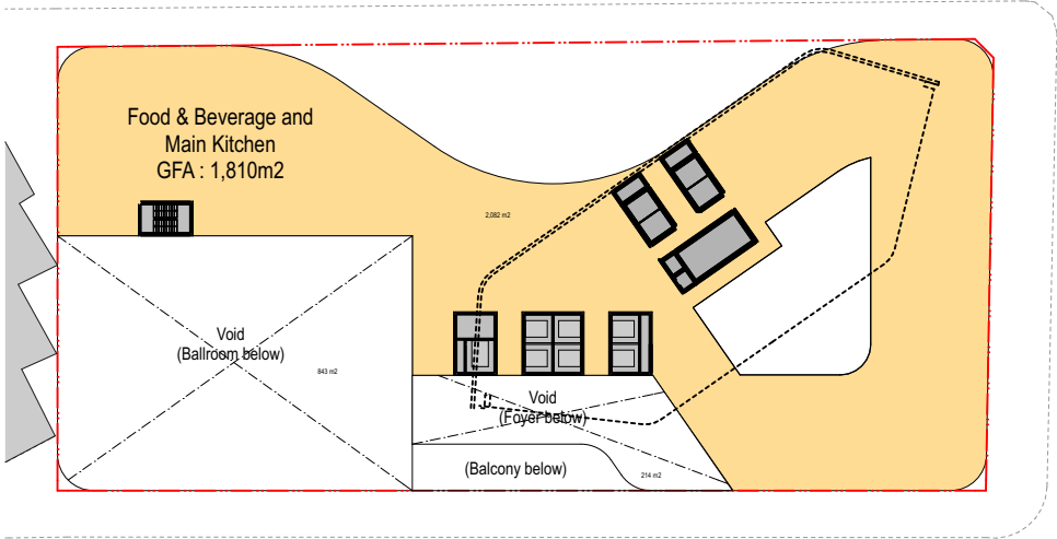
LEVEL 02 Plan
