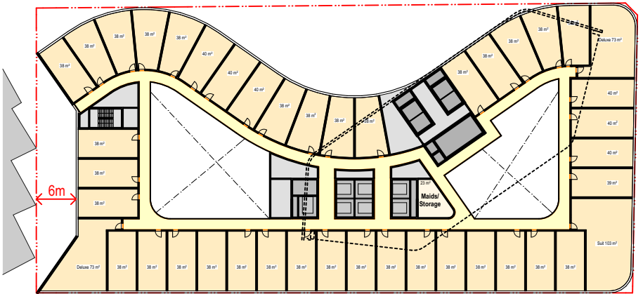
GFA : 2,470m2 (Level 03-05 : 43 rooms)
