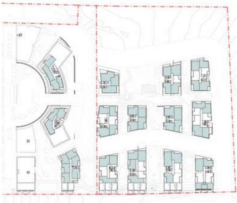
1 CROSS VENTILATION - RL 66.60 1:1200
