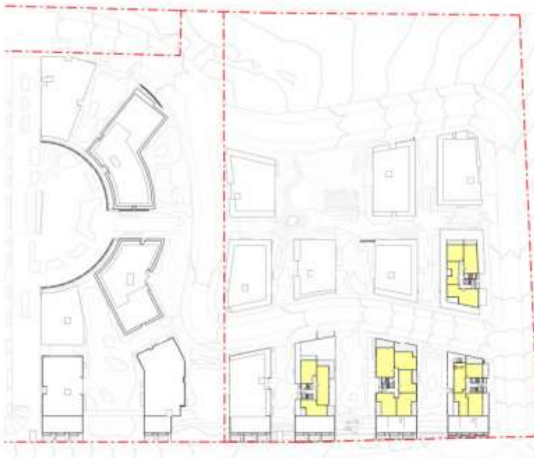
④ SOLAR COMPLIANCE - RL 76.20 1:1200
