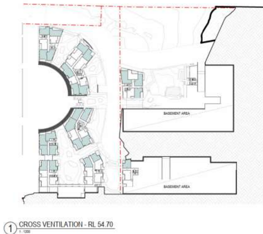
Figure 8 Cross Ventilation Assessment
