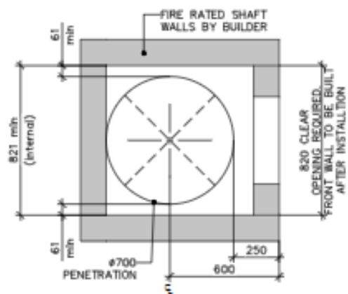
04 SINGLE (610Ø) GALV. STEEL CHUTE WITH CIRCULAR PENETRATION SET-OUT
