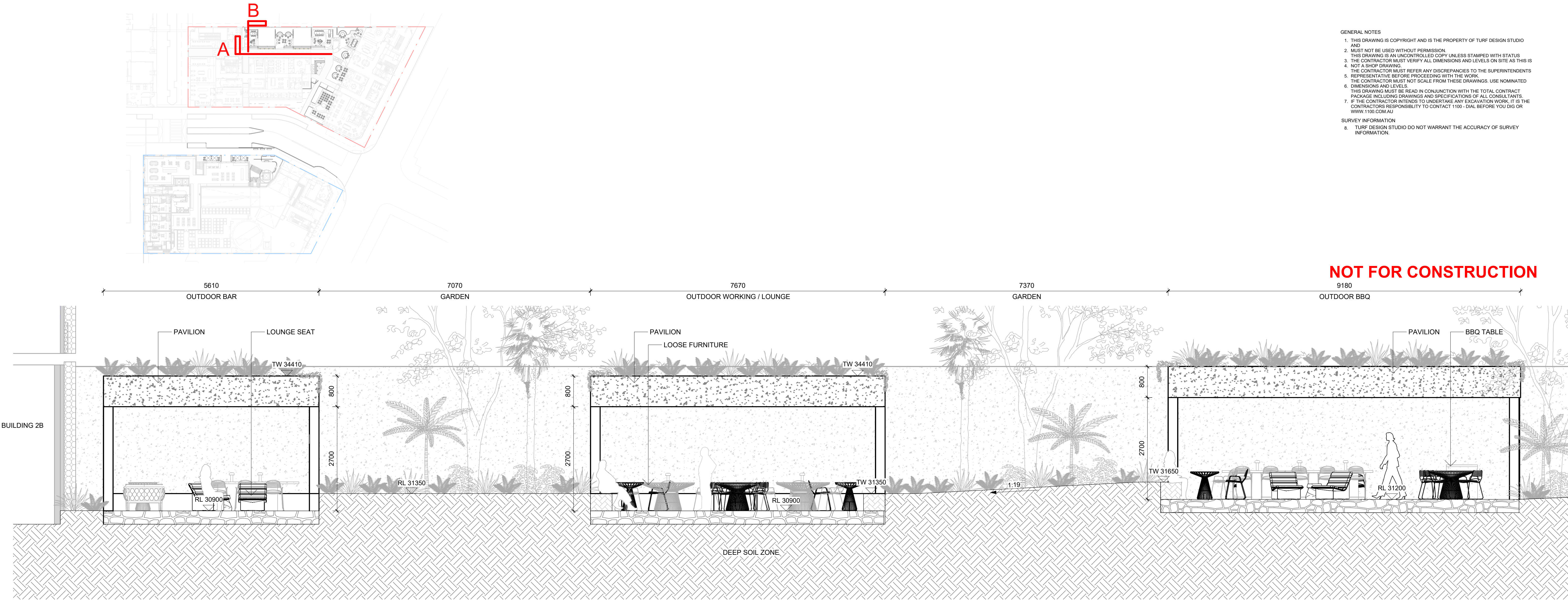
1 SECTION A - GROUND LEVEL PARCEL 2 COMMUNAL SPACE LONG SECTION 1 : 50
