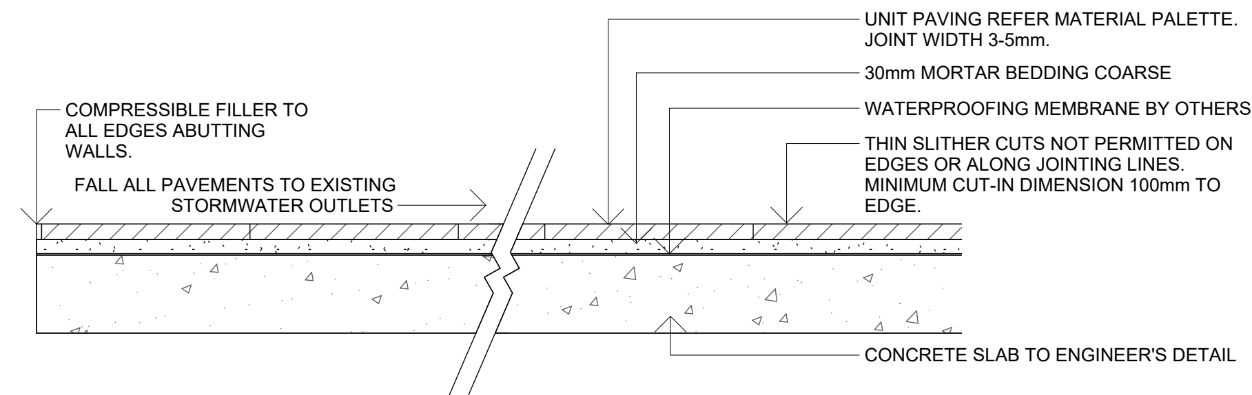
1 P1&P6 - UNIT PAVING ON CONCRETE 1 : 10
