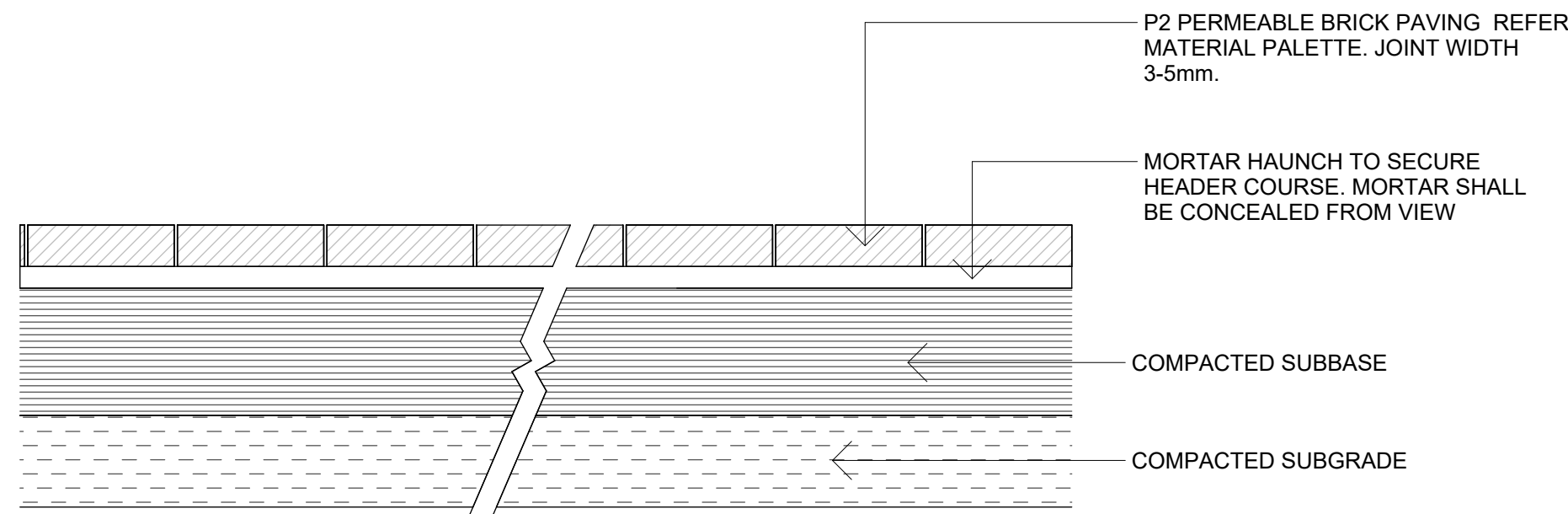
4 P2 - PERMEABLE BRICK PAVING 1 : 10
