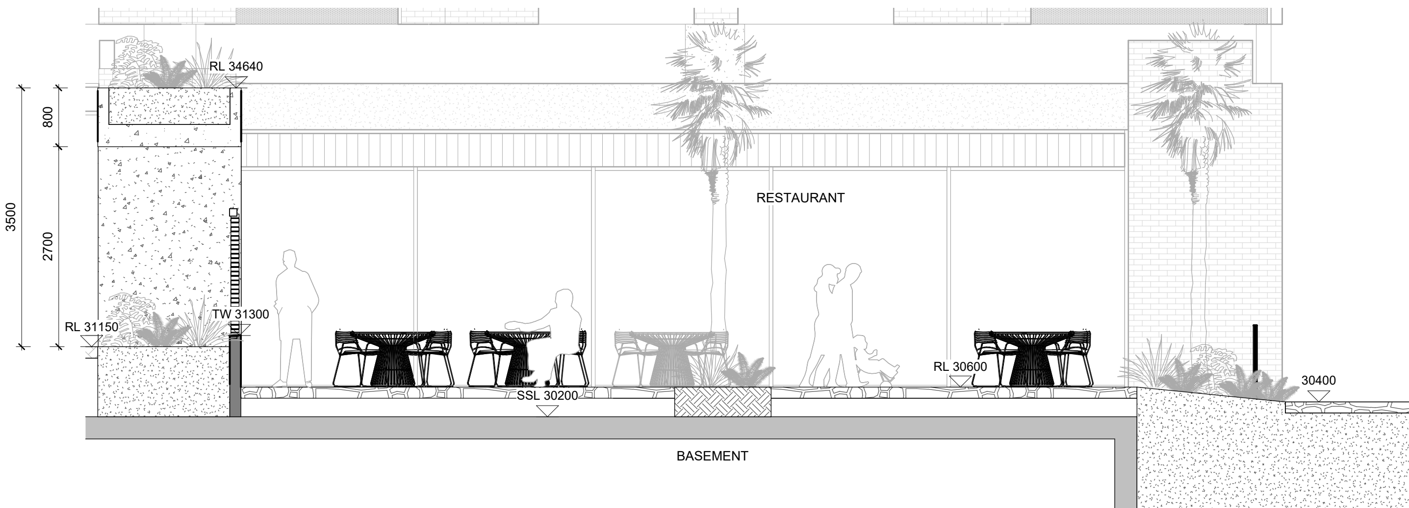
1 SECTION D - GROUND LEVEL PARCEL 2 RESTAURANT OUTDOOR DINING 1 : 50
