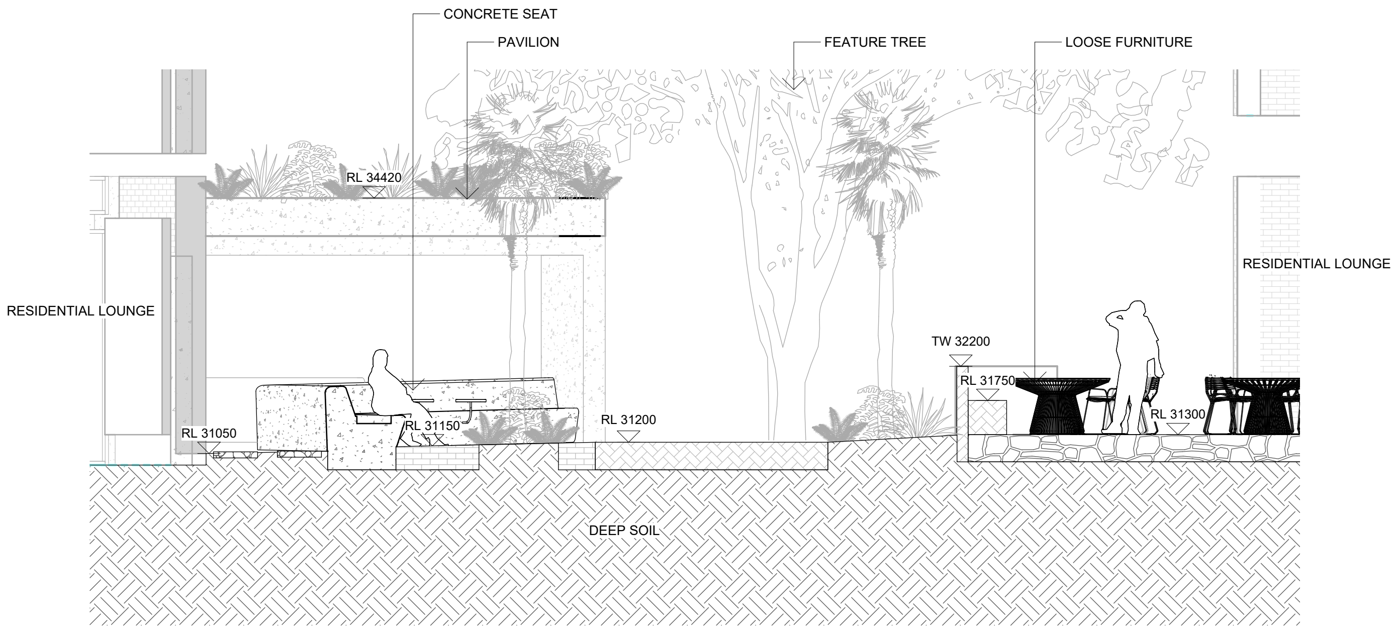
2 SECTION C - GROUND LEVEL PARCEL 2 OUTDOOR LOUNGE 1 : 50
