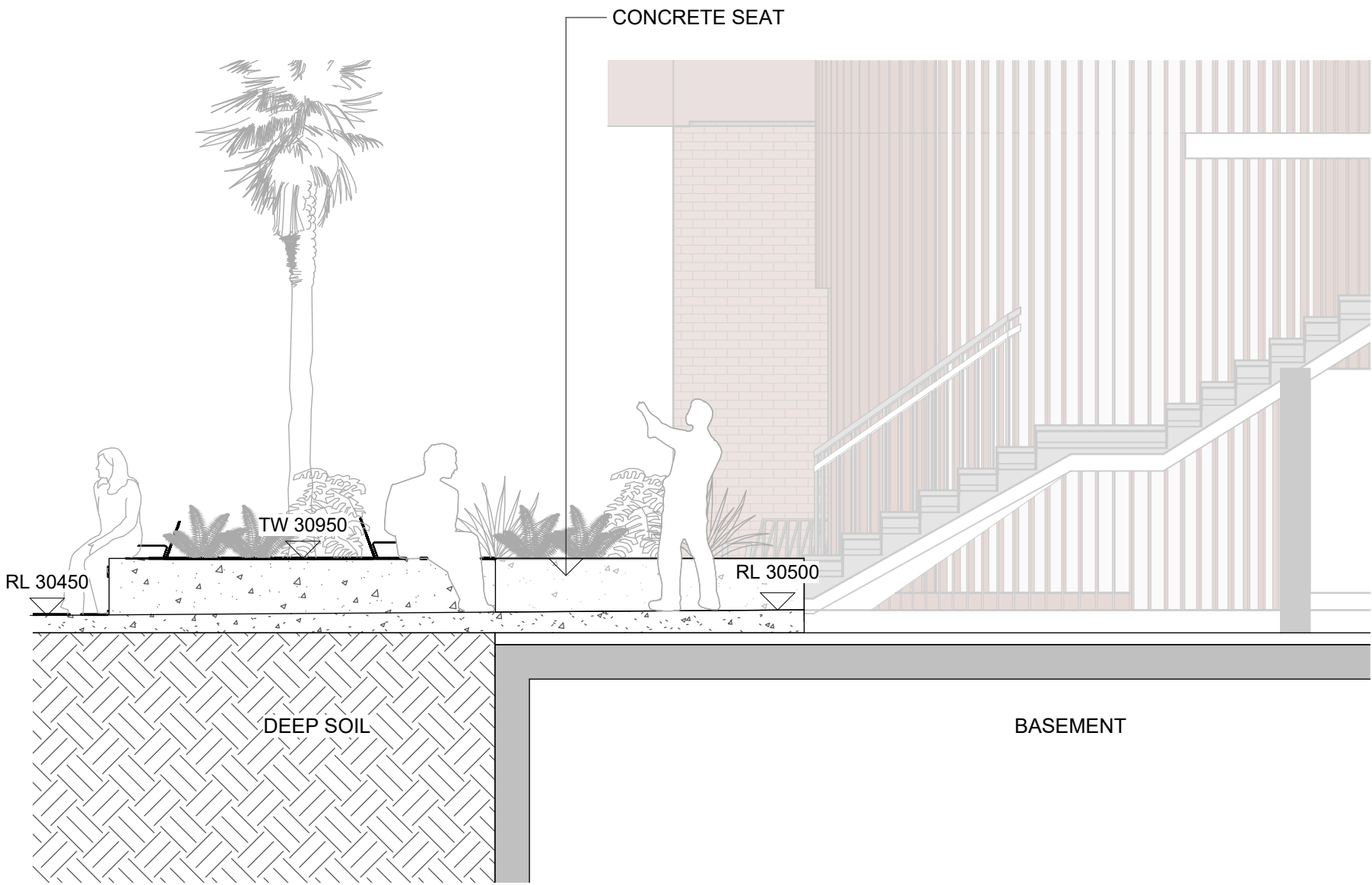
1 SECTION E - GROUND LEVEL PARCEL 3 PLAZA 1 : 50
