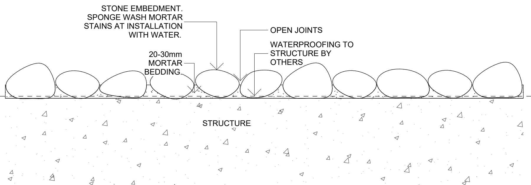
5 P7 - TYPICAL WHITE PEBBLE 1 : 5
