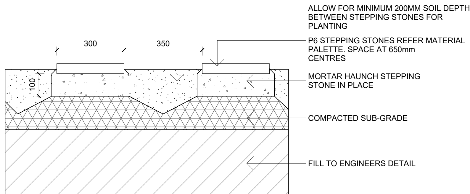
3 P5 - STEPPING STONES IN GARDEN 1 : 10
