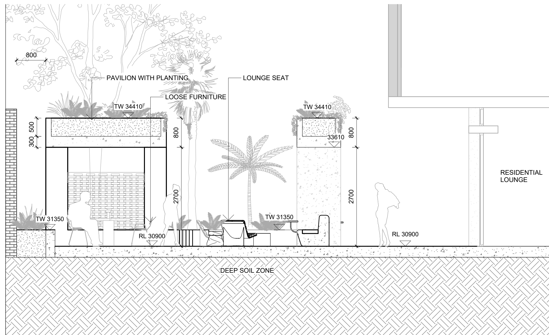
2 SECTION B - GROUND LEVEL PARCEL 2 COMMUNAL SPACE 1 : 50
