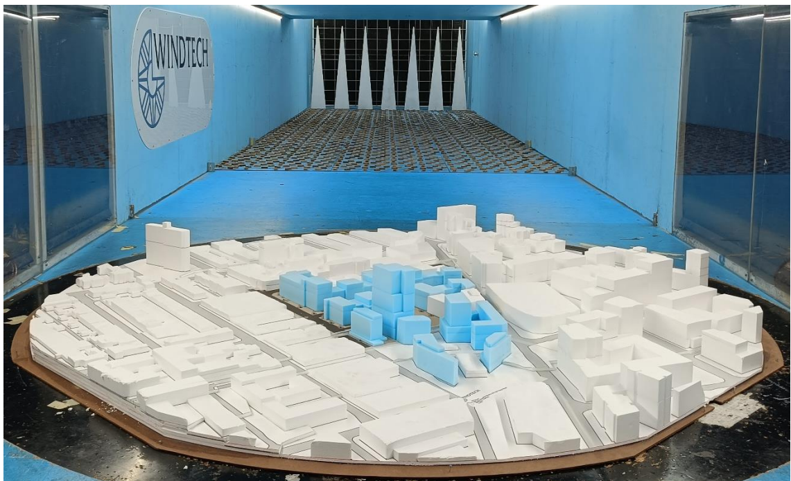
Figure 3d: Photograph of the Wind Tunnel Model (view from the south-west) - Approved Site
