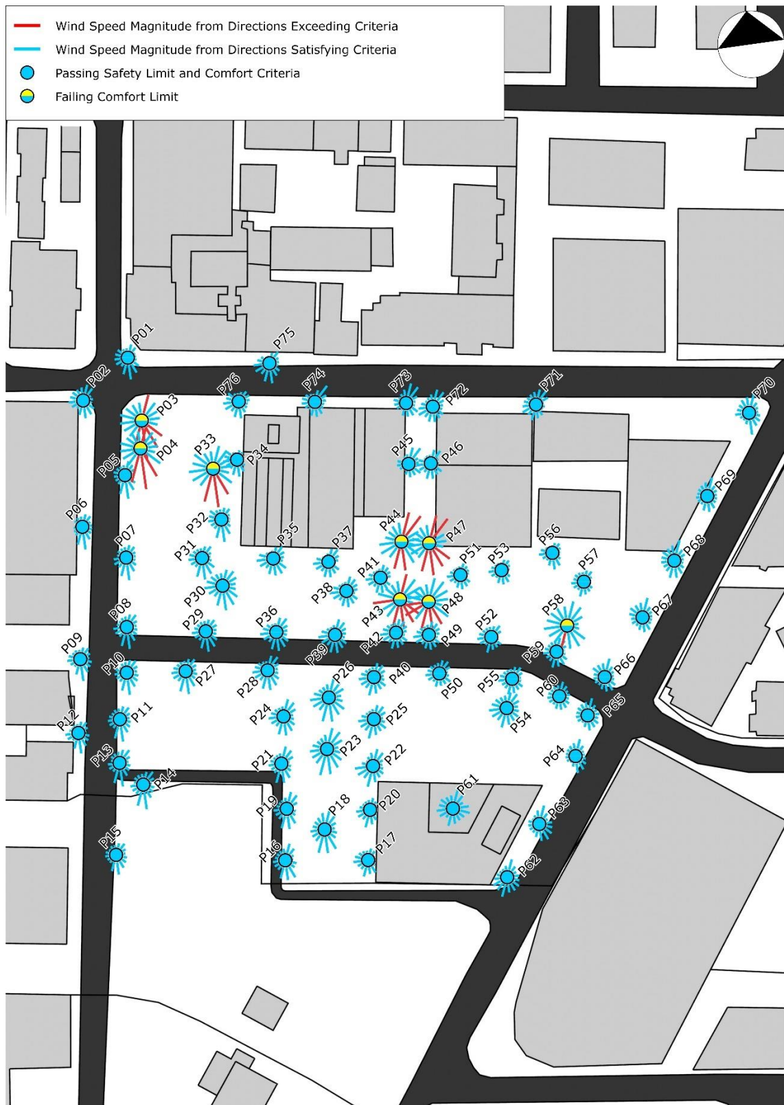
Figure 8c: Wind Tunnel Results – Ground Floor Plan (Existing Scheme) (results shown without treatments applied)
