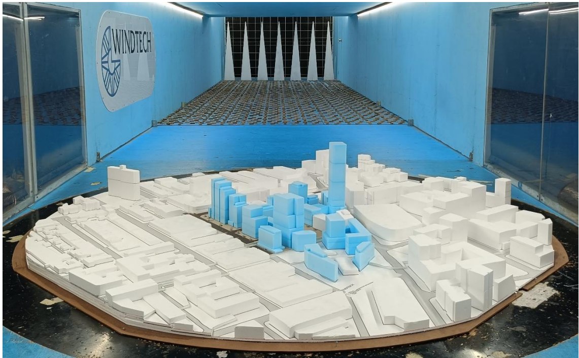
Figure 2d: Photograph of the Wind Tunnel Model (view from the south-west) - Proposed Site
