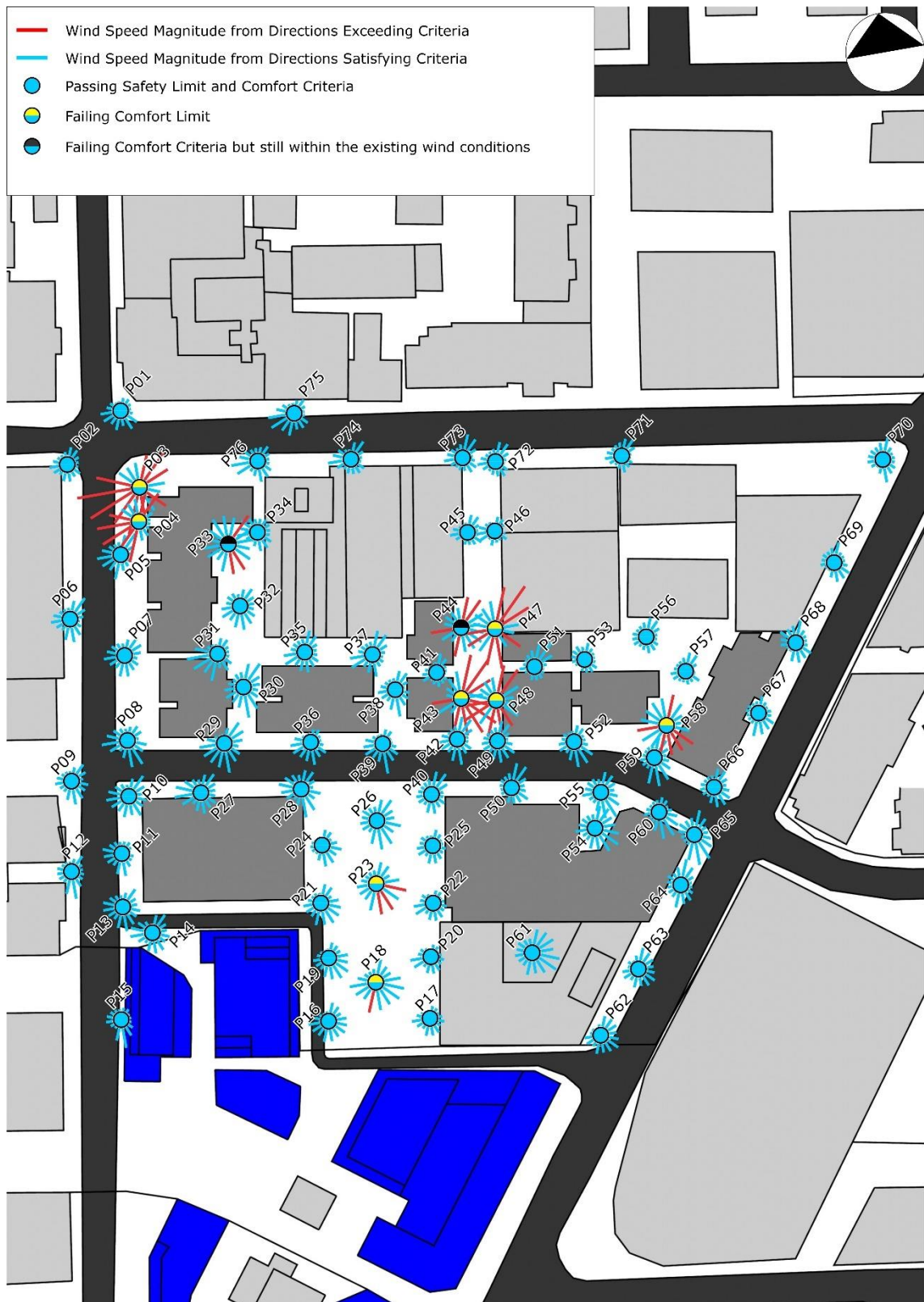
Figure 8a: Wind Tunnel Results – Ground Floor Plan (Proposed Scheme) (results shown without treatments applied)
