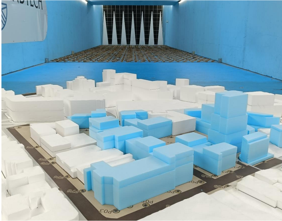
Figure 3a: Photograph of the Wind Tunnel Model (view from the north-west) – Approved Site
