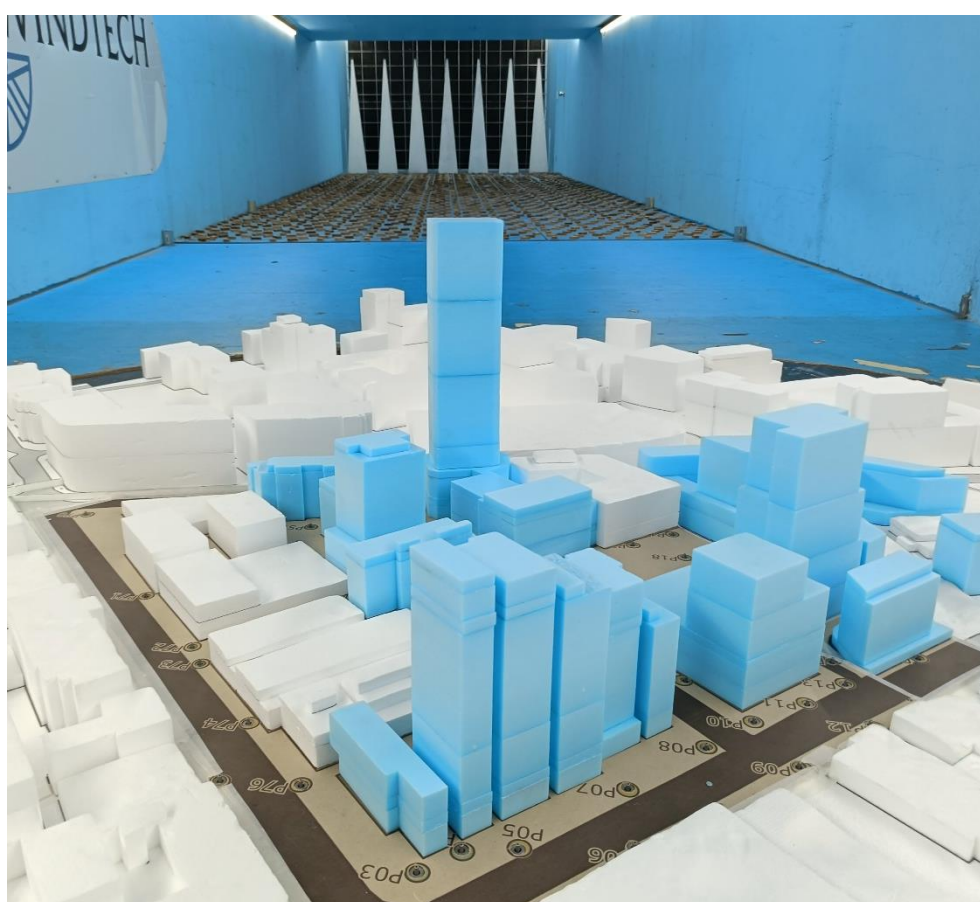
Figure 2a: Photograph of the Wind Tunnel Model (view from the north-west) – Proposed Site
