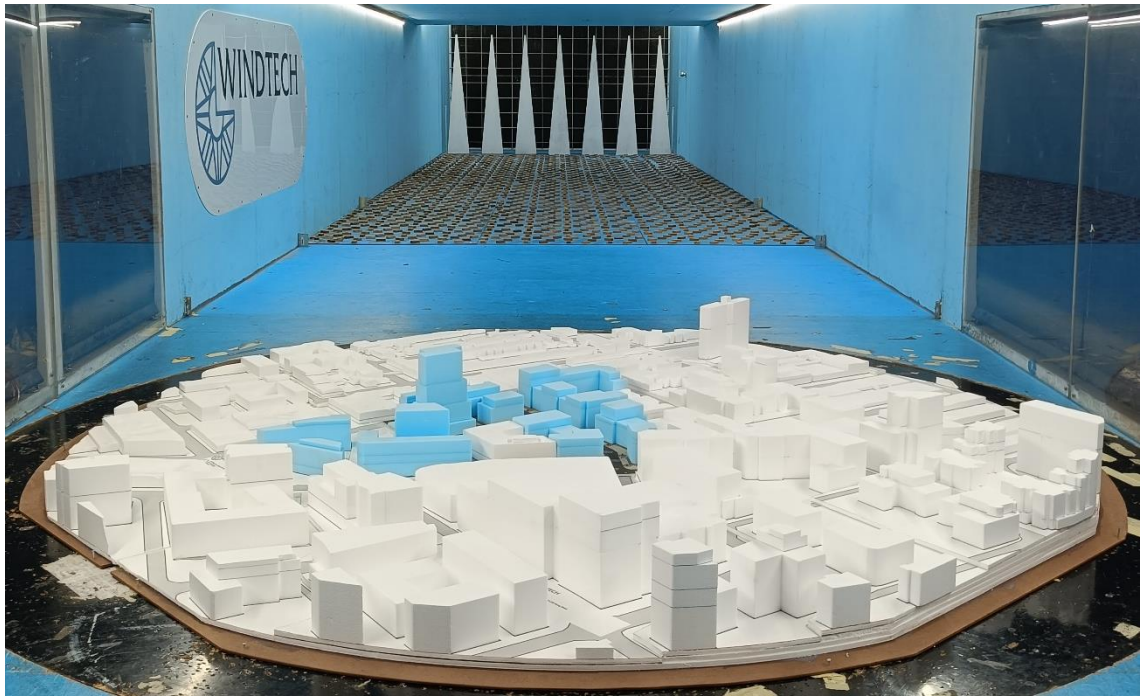
Figure 3c: Photograph of the Wind Tunnel Model (view from the south-east) - Approved Site
