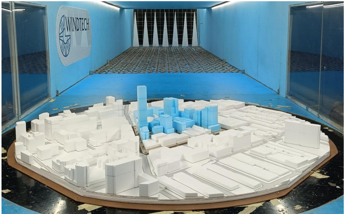
Figure 2b: Photograph of the Wind Tunnel Model (view from the north-east) - Proposed Site
