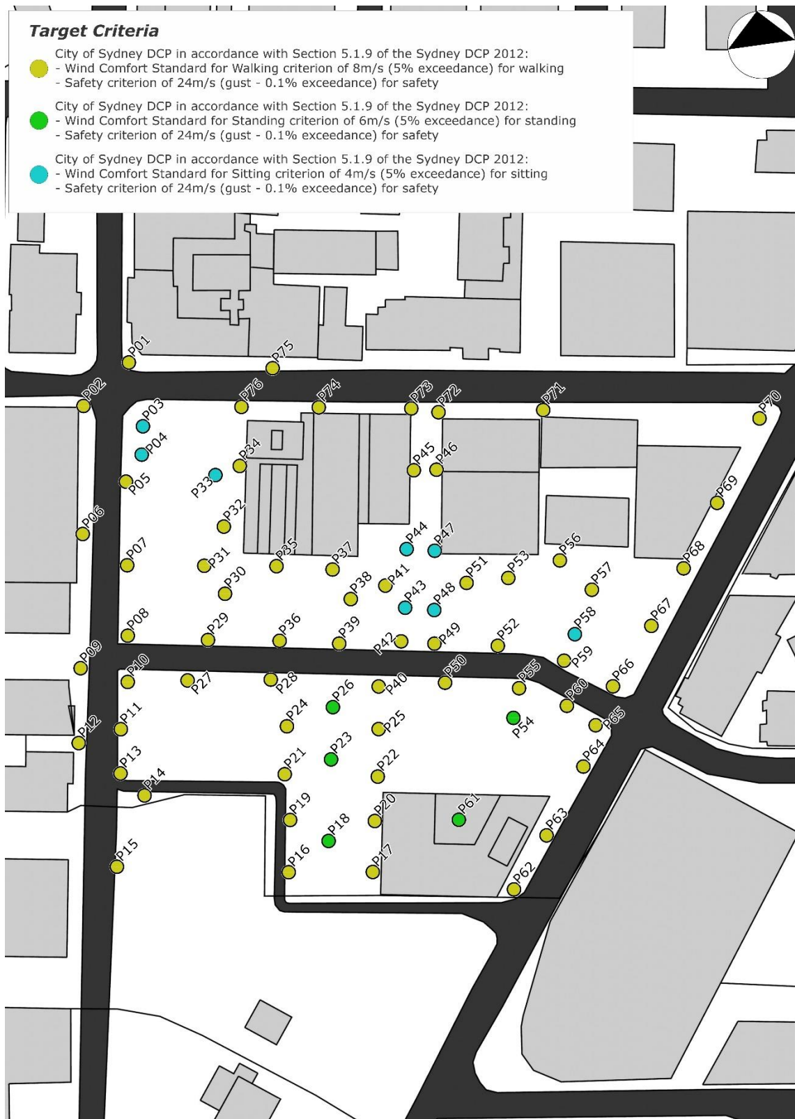
Figure 7c: Study Point Locations and Target Wind Speed Criteria – Ground Floor Plan (Existing Scheme)
