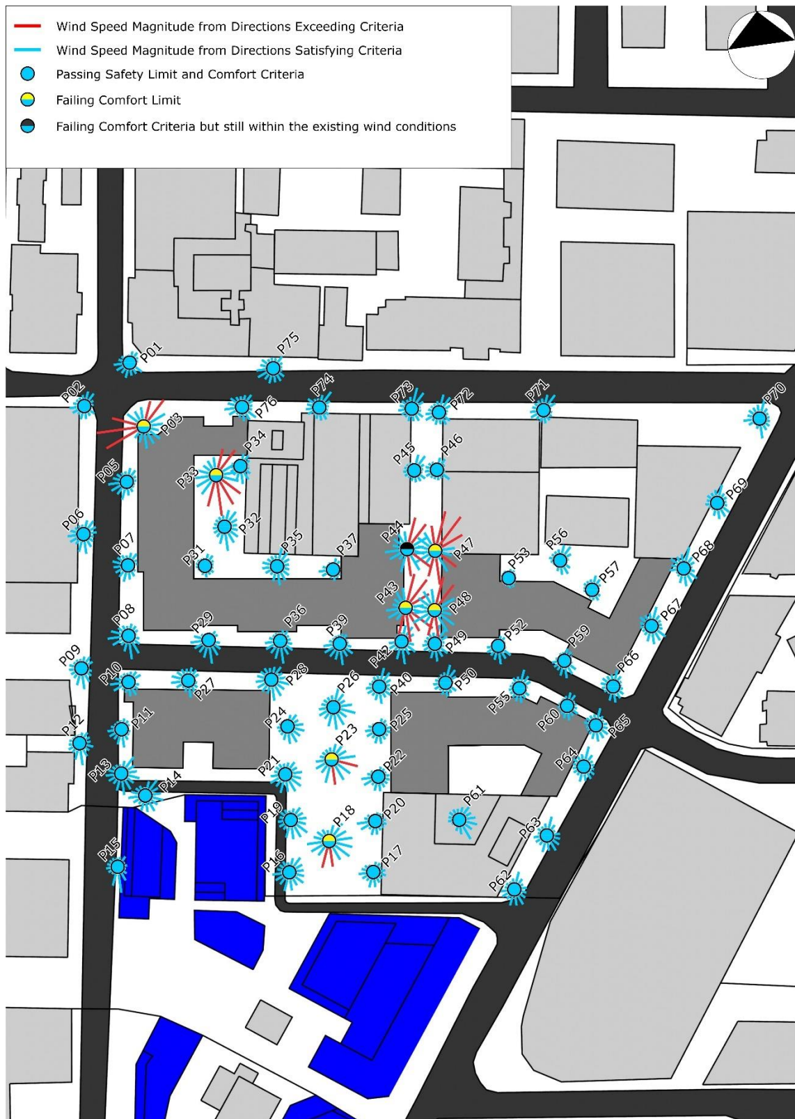
Figure 8b: Wind Tunnel Results – Ground Floor Plan (Approved Scheme) (results shown without treatments applied)
