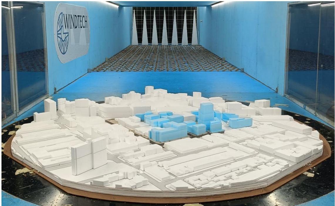
Figure 3e: Photograph of the Wind Tunnel Model (view from the north-west) - Approved Site
