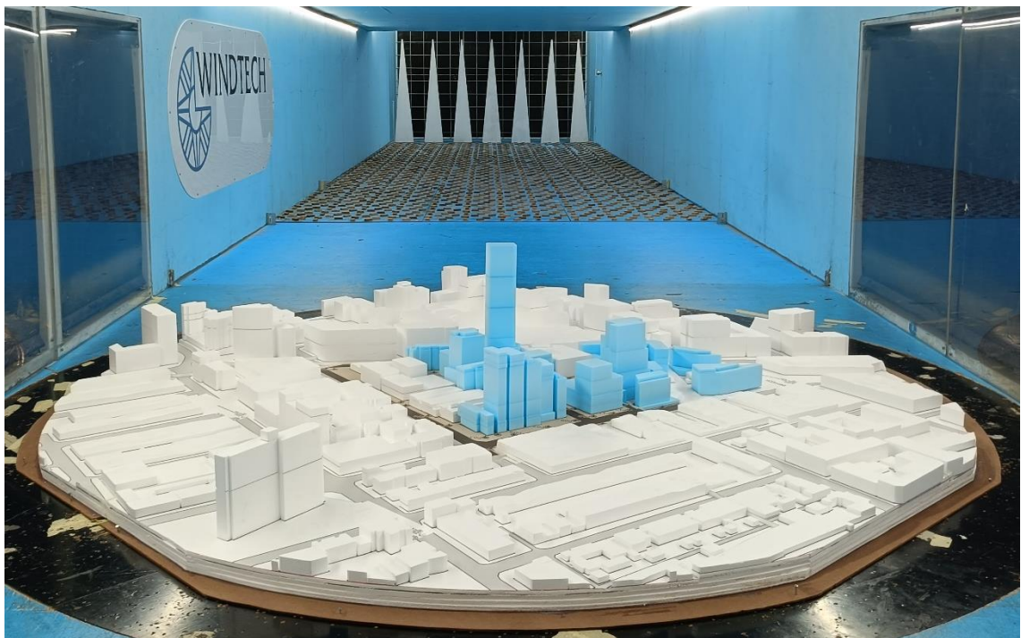
Figure 2e: Photograph of the Wind Tunnel Model (view from the north-west) - Proposed Site
