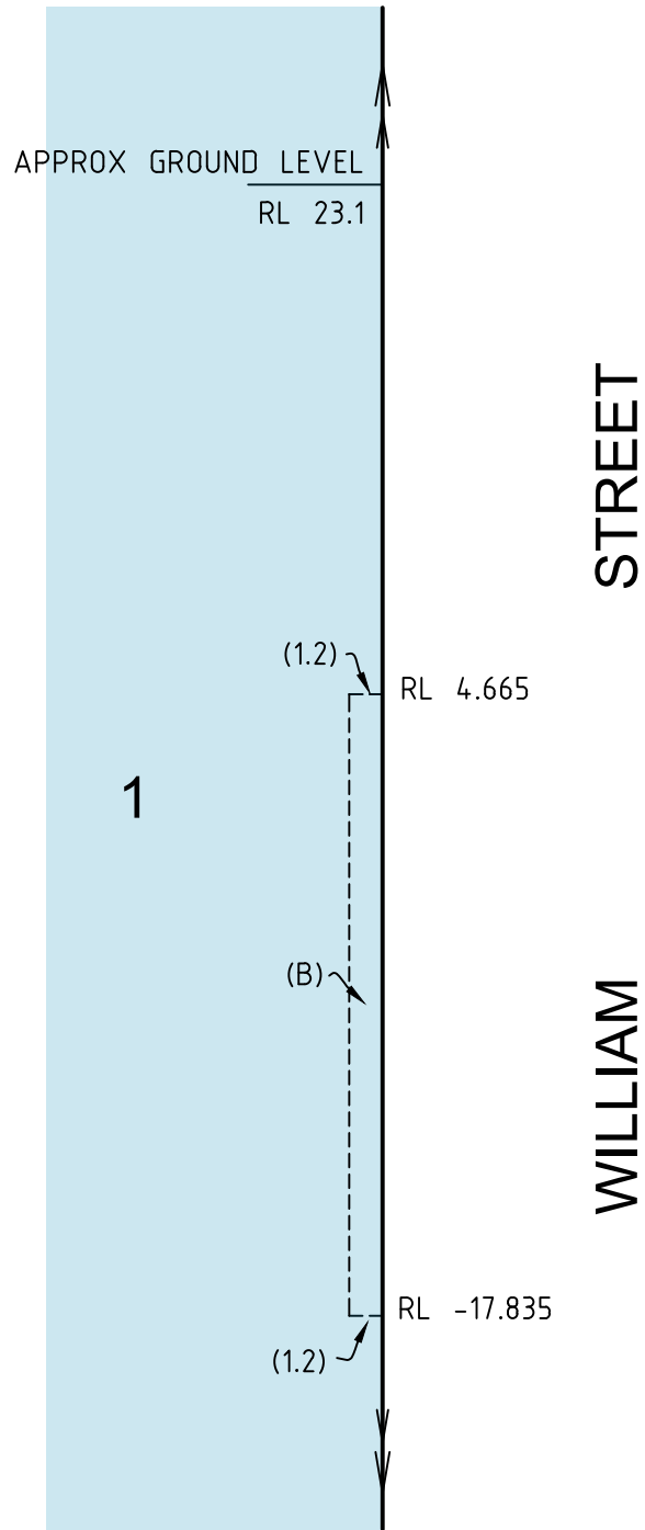
SECTION C-C 1:300
