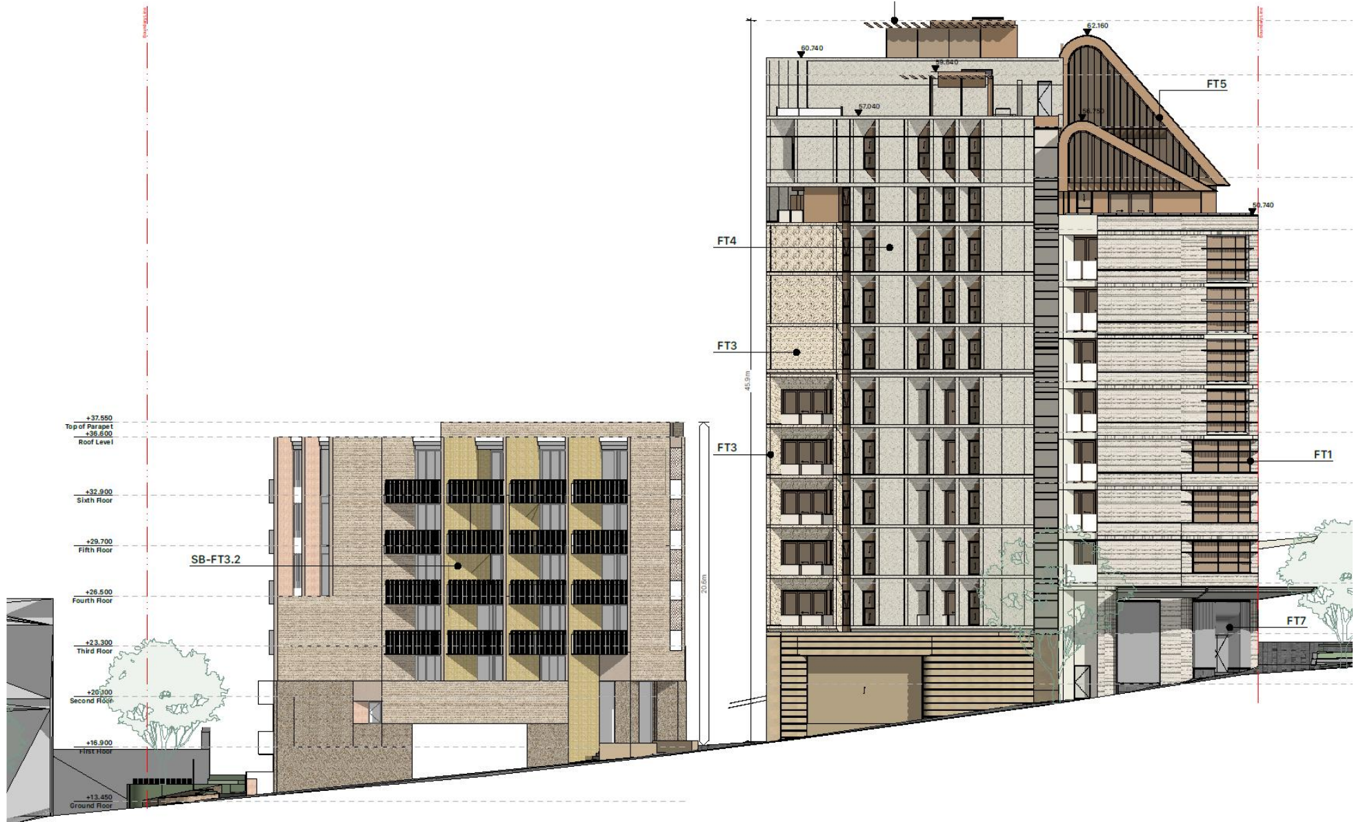
ELEVATION 4 WEST - 164-194 William St, Woolloomooloo 2011
