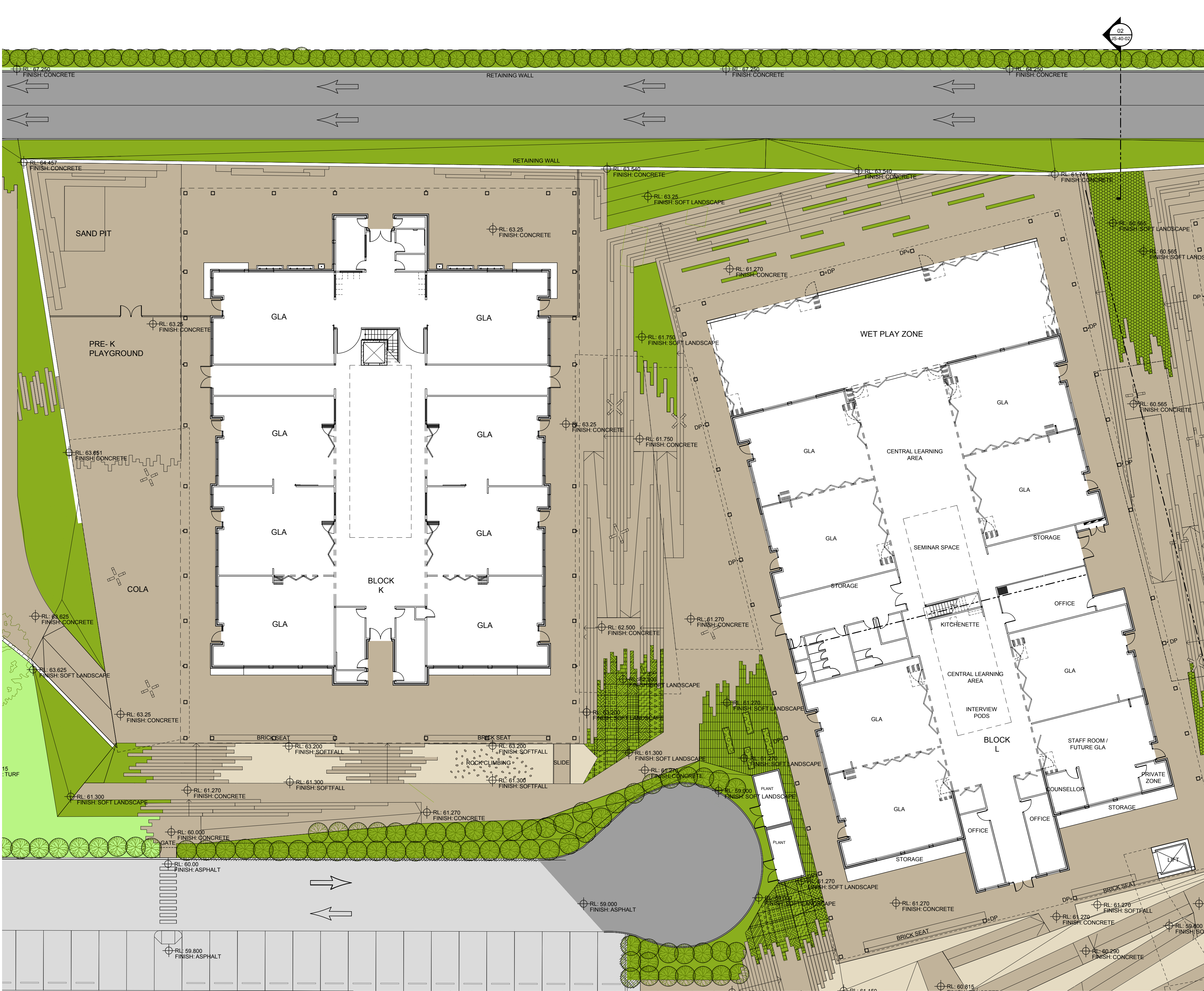
01 MAINTENANCE SHED AND CARPARK LANDSCAPE PLAN 1:200 @ A1
