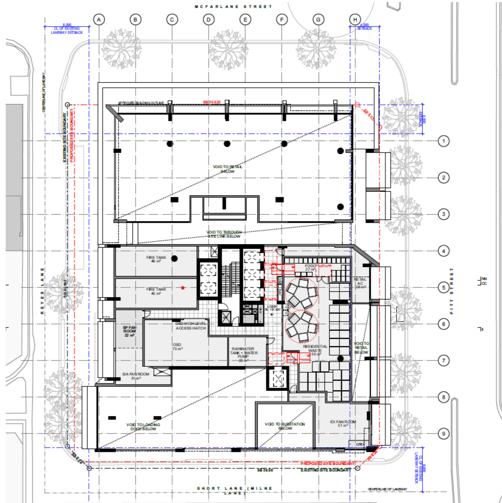
Source Fuse Architects, SSDA 107, Rev A, Oct2025 - Ground Level Plan - Mezzanine:
