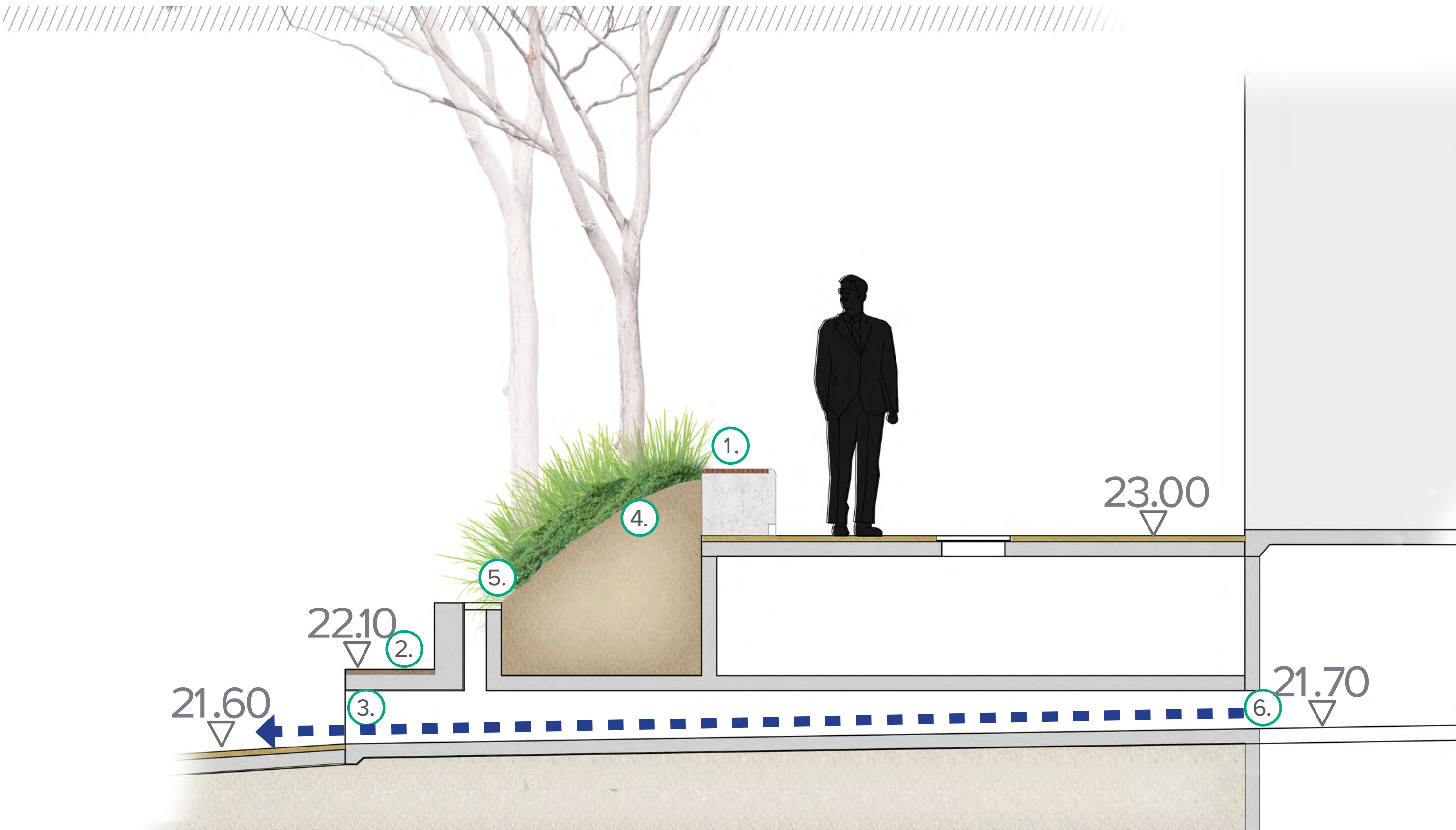
Section DD SCALE 1:25 @ A1
