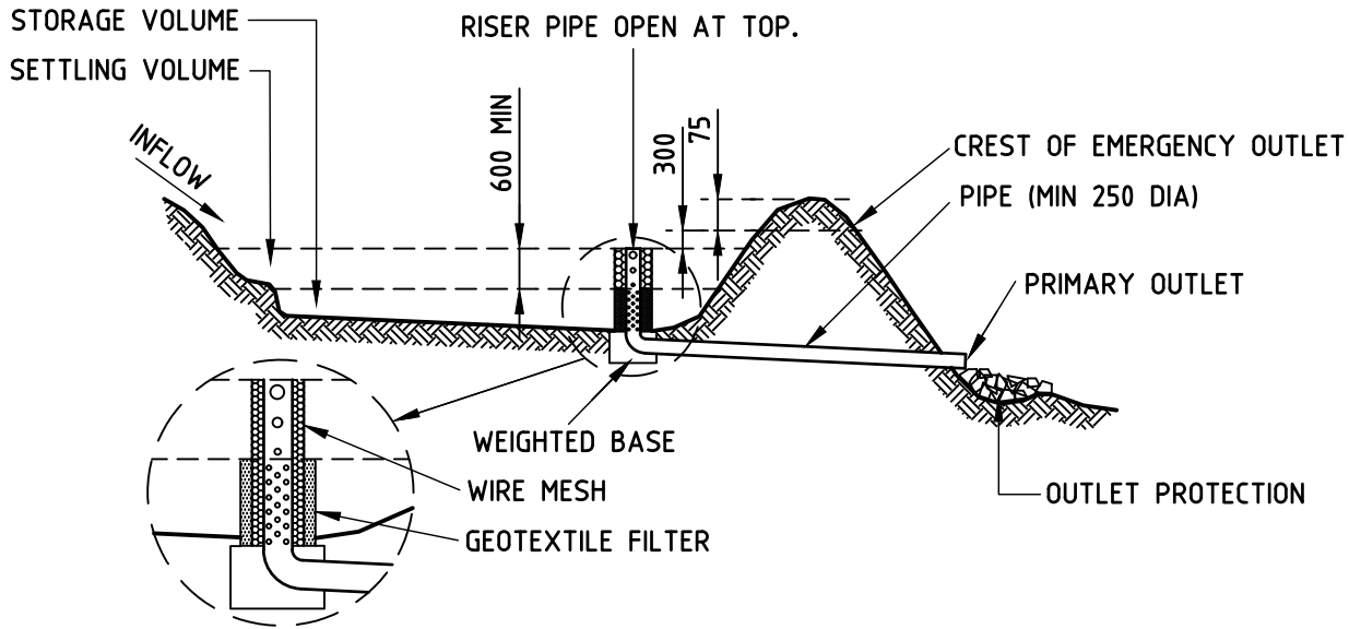
CROSS SECTION OF TYPICAL SEDIMENT BASIN.
