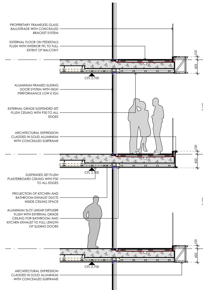
03 Recessed Facade Aluminium facade cladding and louvred blades in dark champagne finish.
