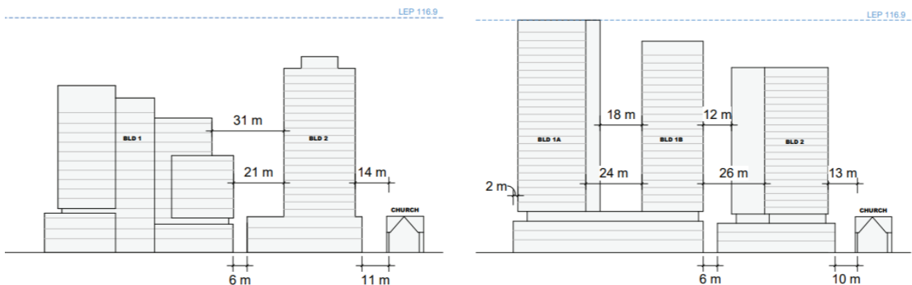
Figure 3 Approved (left) and Proposed (right) massing
