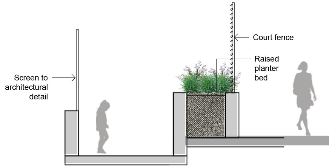
02 LG2 Court Planter Section 601 1:50
