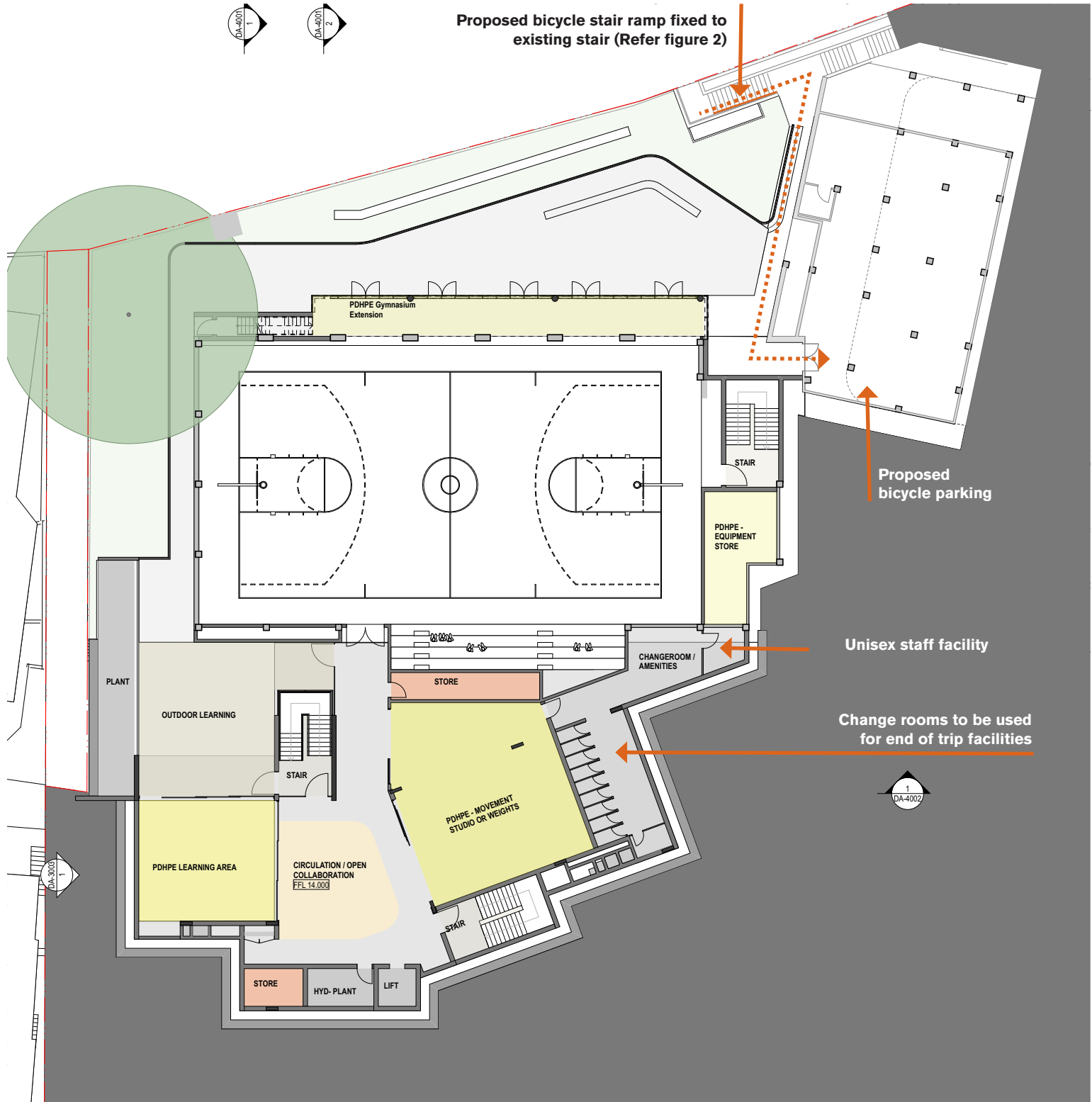
Figure 3 - Proposed Lower Ground Level 4 Plan
