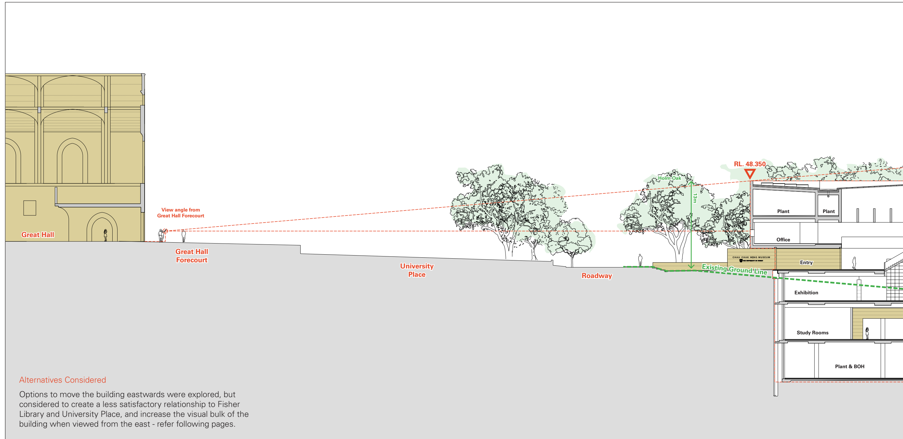
Proposed Cross Section, Looking North NTS
