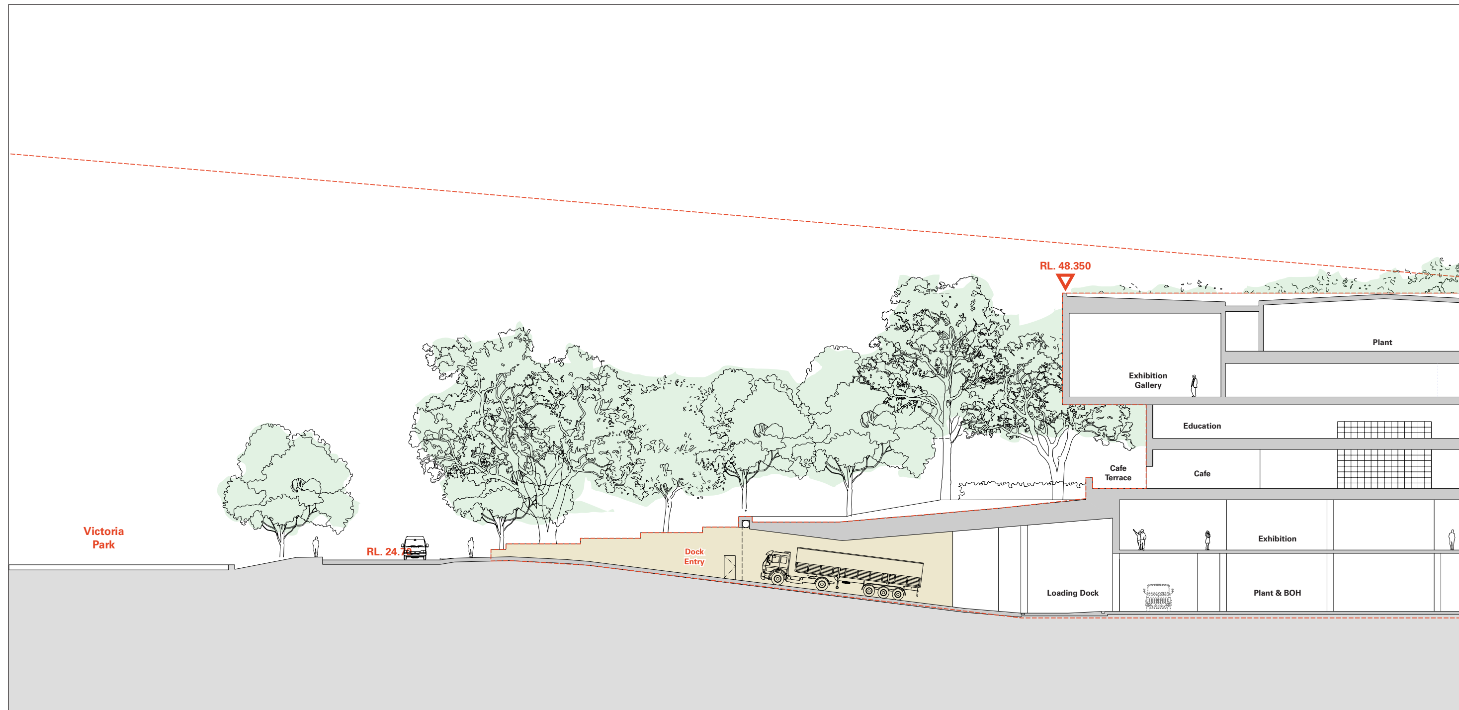
Proposed Cross Section, Looking South NTS
