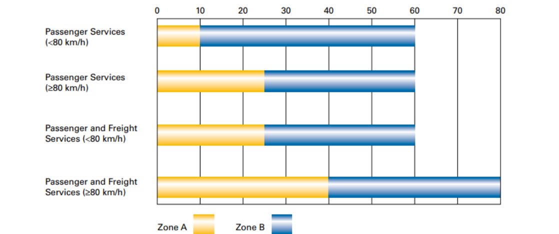
Figure 2 Noise Assessment Zones based on Distance (m) of Noise – Sensitive Development from Operational Track (Not Corridor)
