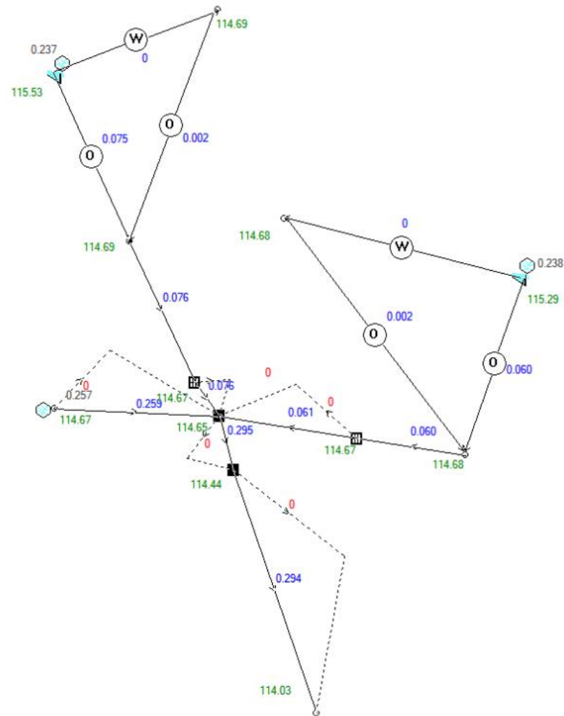
Figure 10 - DRAINS model results, 10% AEP event
