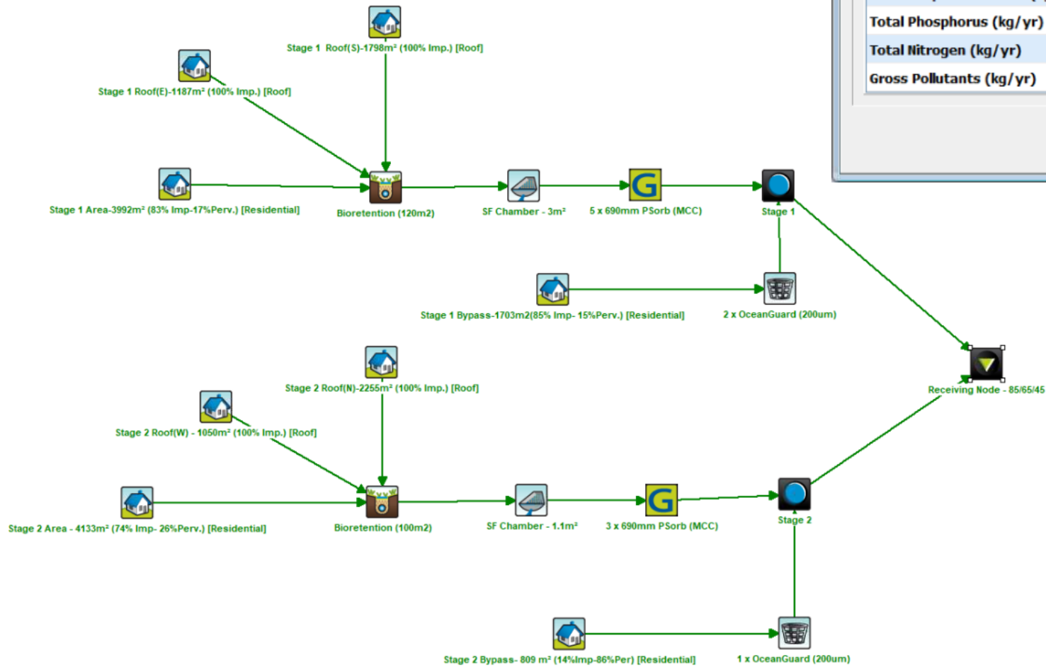
Figure 15 - Water Quality Management Strategy MUSIC Model Configuration
