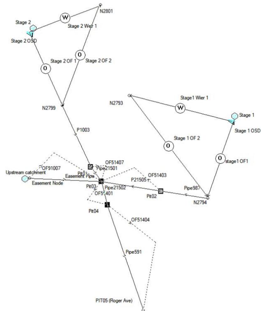
Figure 9 - DRAINS model setup
