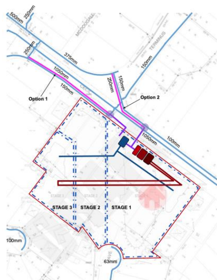
Figure 8. Two options for water main upgrade
