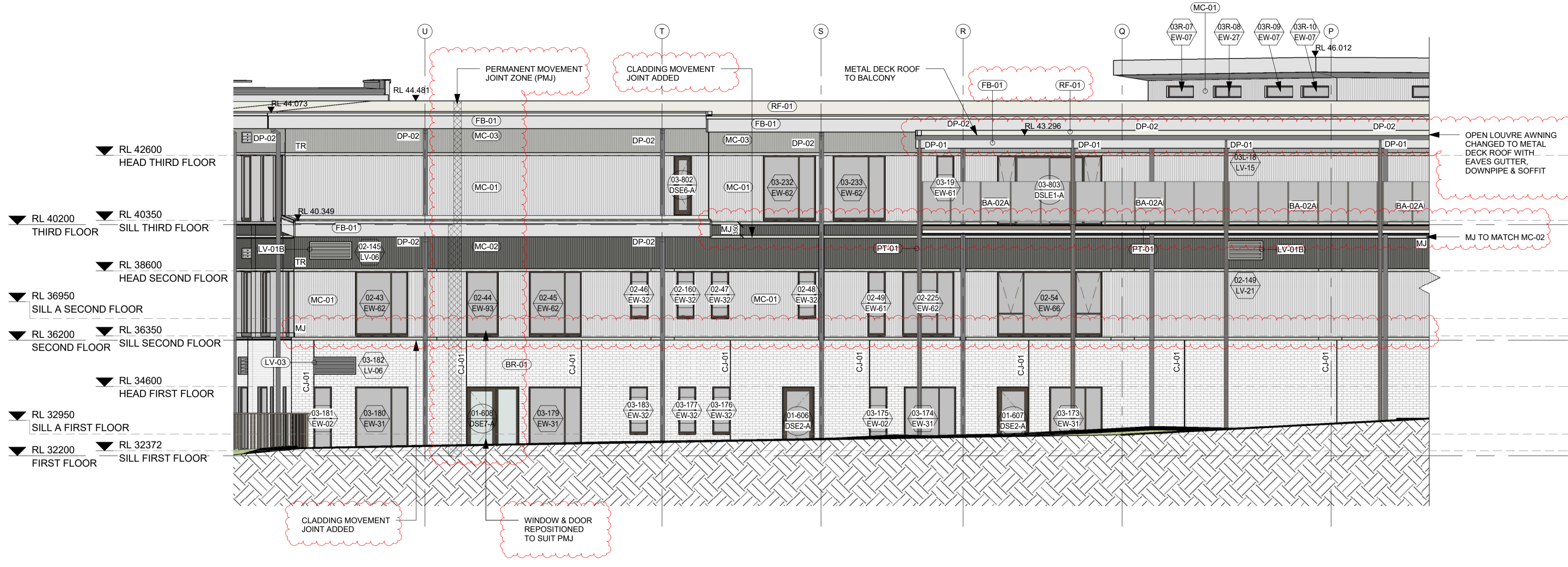
1 ELEVATION 6 - IRT NORTH PART 01 1:100
