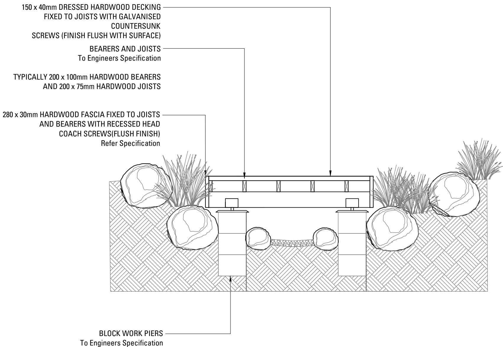
08 P8 - TIMBER BRIDGE SCALE 1:20
