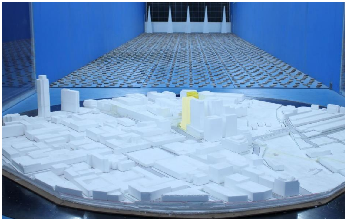
Figure 1a: Photograph of the Wind Tunnel Model – Proposed Scenario (View from the north-east)
