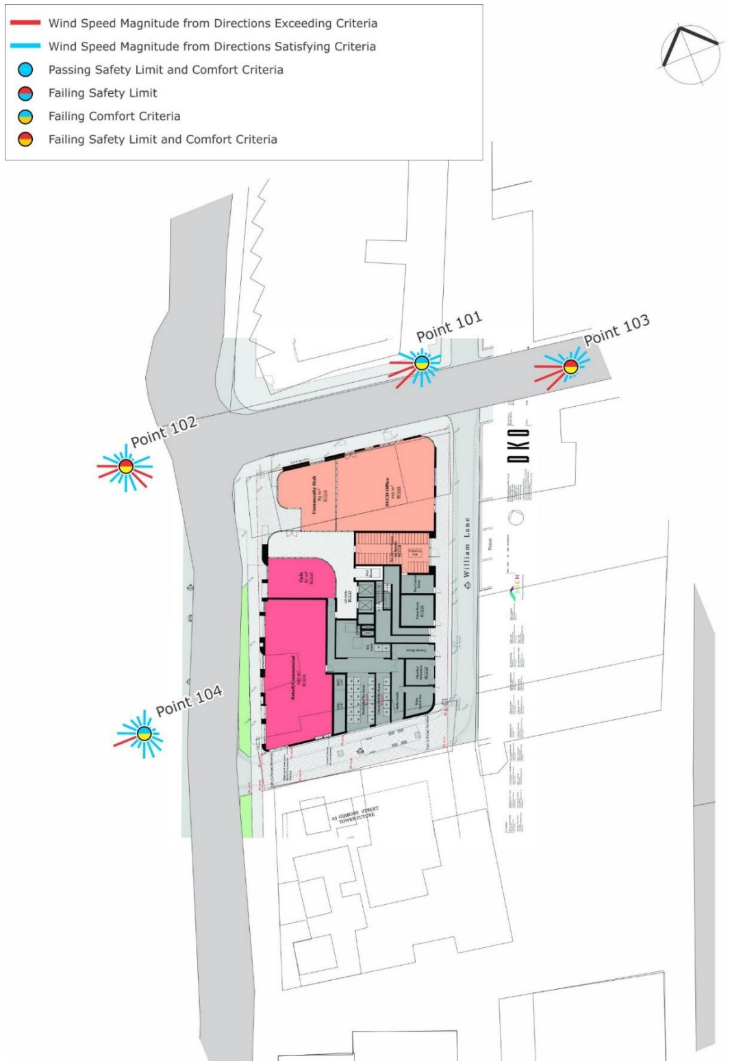
Figure 6d: Wind Tunnel Results – Surrounding Points
