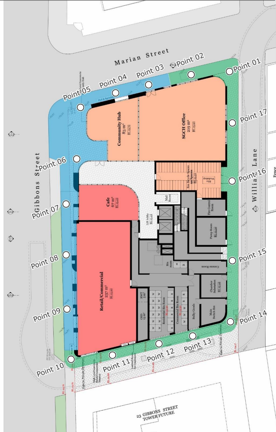
Figure 5a: Study Point Locations and Target Wind Speed Criteria - Ground Floor
