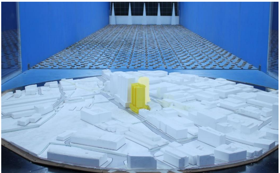
Figure 1c: Photograph of the Wind Tunnel Model – Proposed Scenario (View from the south-west)
