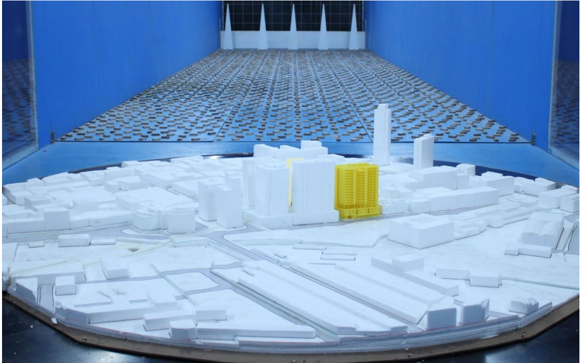
Figure 1d: Close up photograph of the Wind Tunnel Model – Proposed Scenario (View from the north-west)
