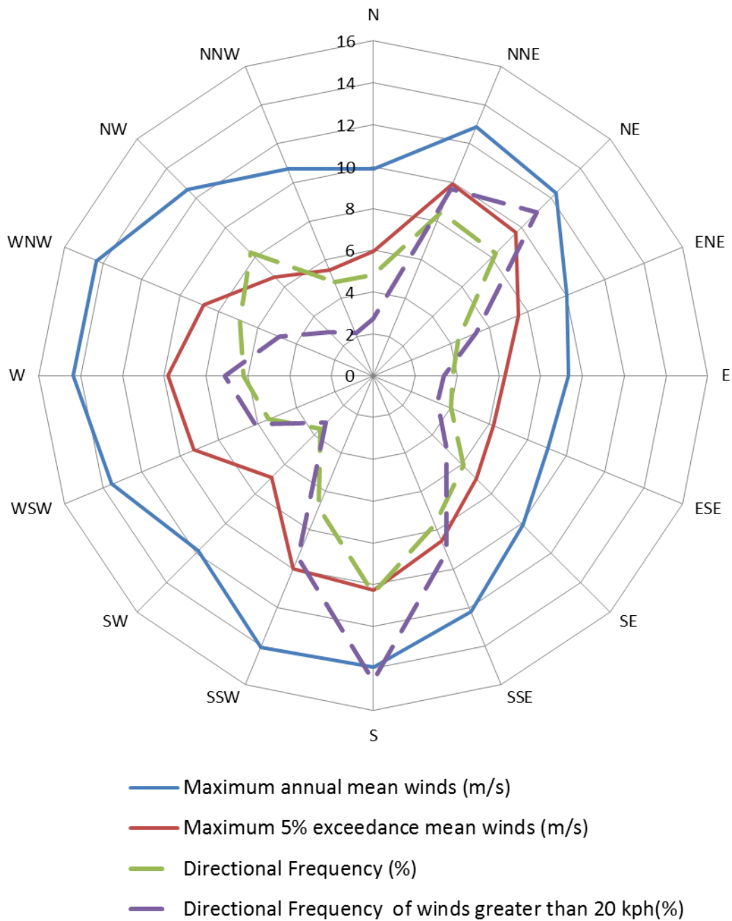
Figure 4: Annual and 5% Exceedance Hourly Mean Wind Speeds, and Frequencies of Occurrence, for the Sydney Region (referenced to 10m above ground in standard open terrain)
