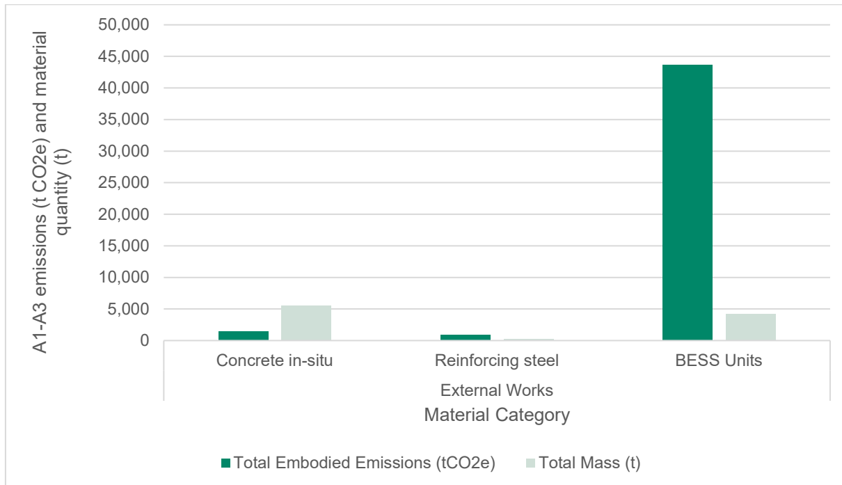
Figure 1: Breakdown of material quantities and embodied emissions
