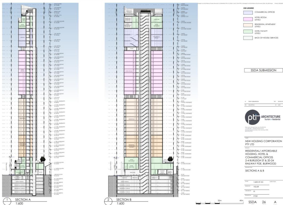
Figure 14. Vertical cross section of proposed building. (Source: PTI Architecture, 3/02/25)
