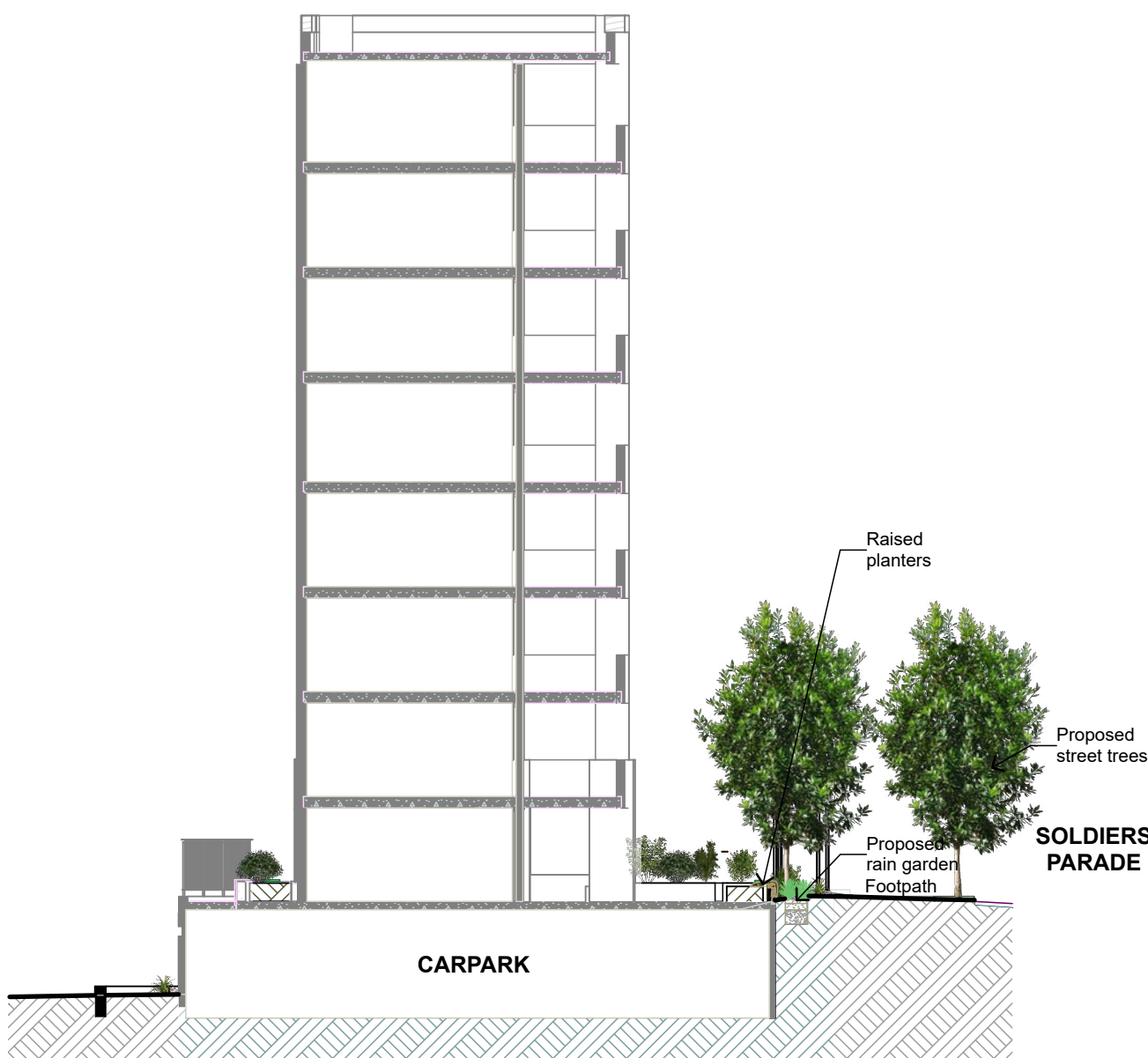
2 Section 1:200
