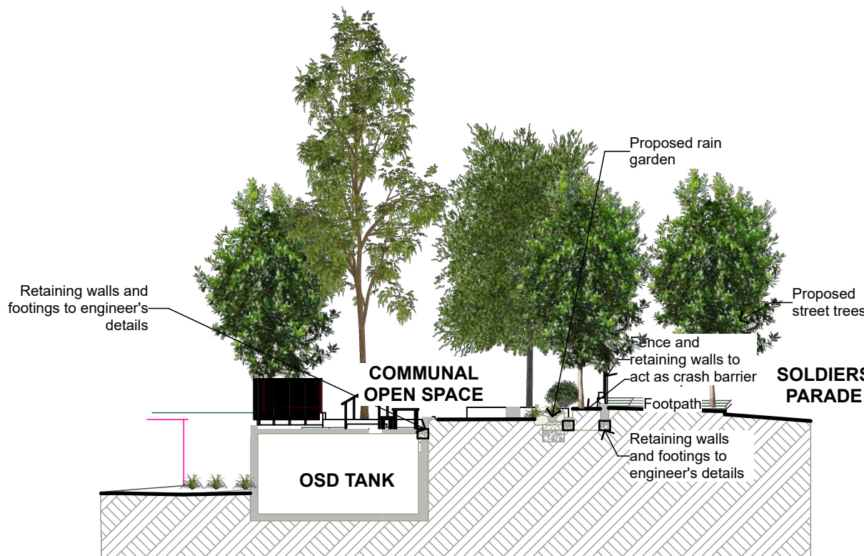
3 Section 1:200
