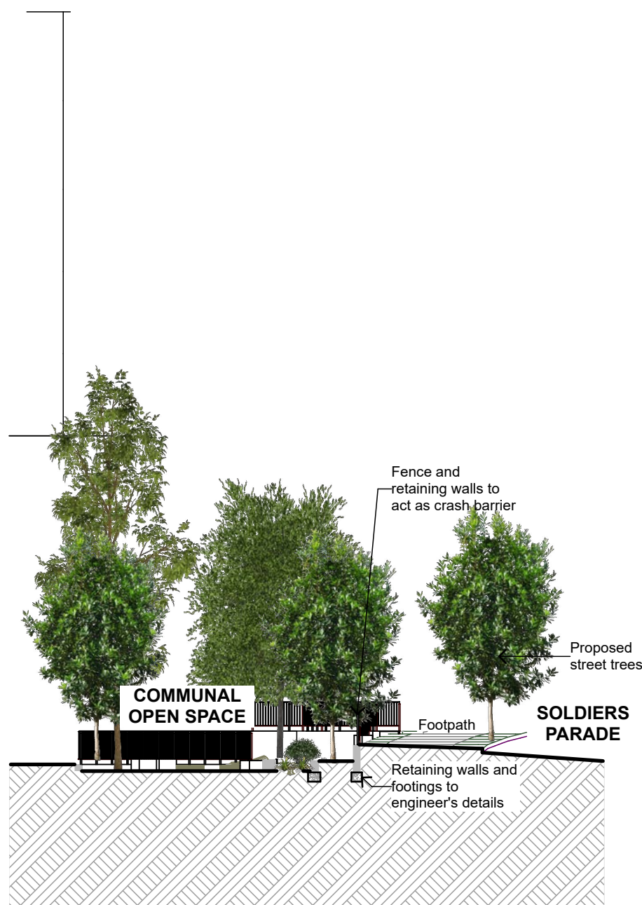
4 Section 1:200
