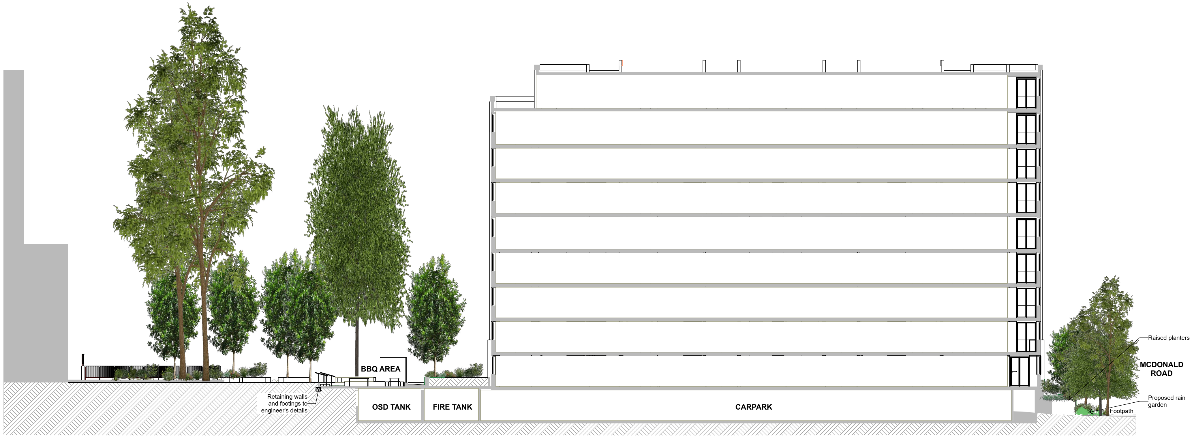
6 Section 1:200
