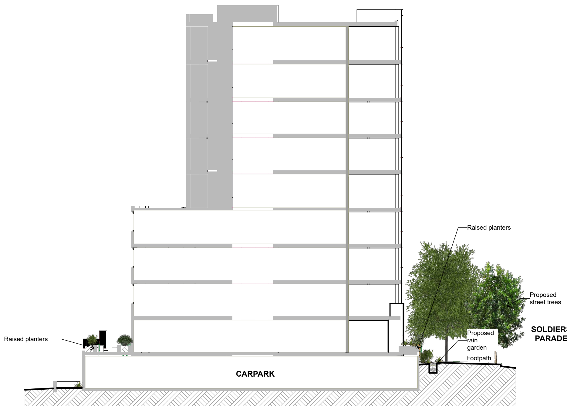
1 Section 1:200
