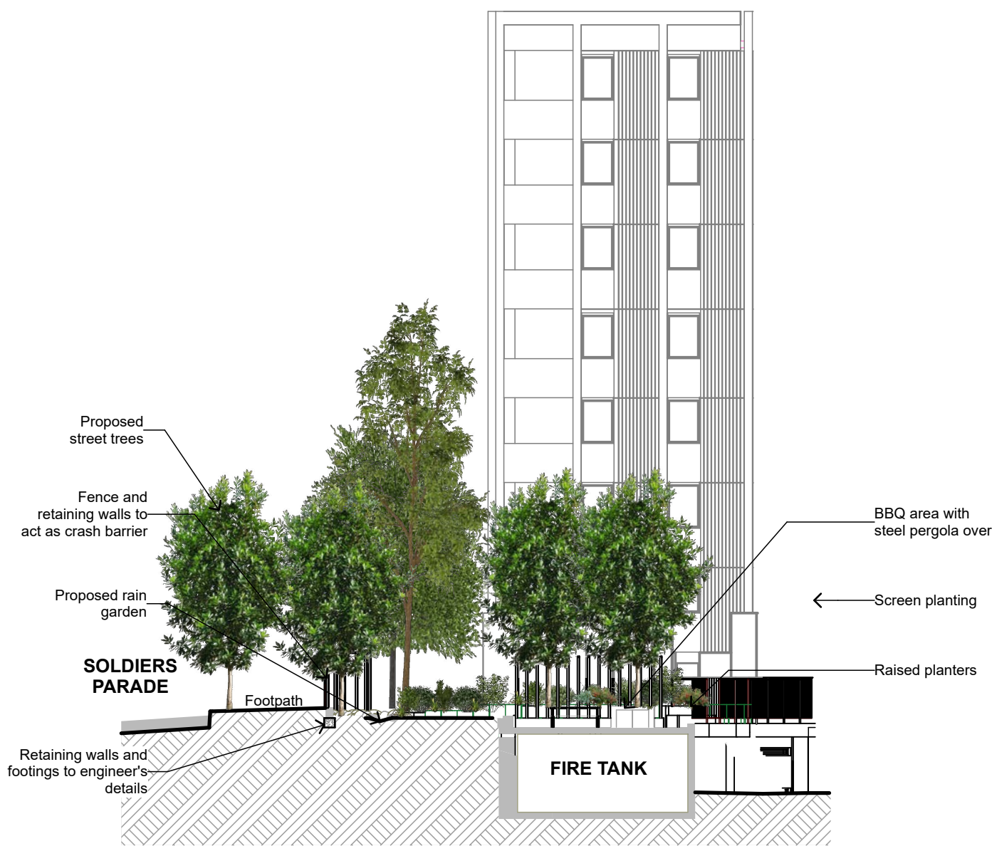
5 Section 1:200
