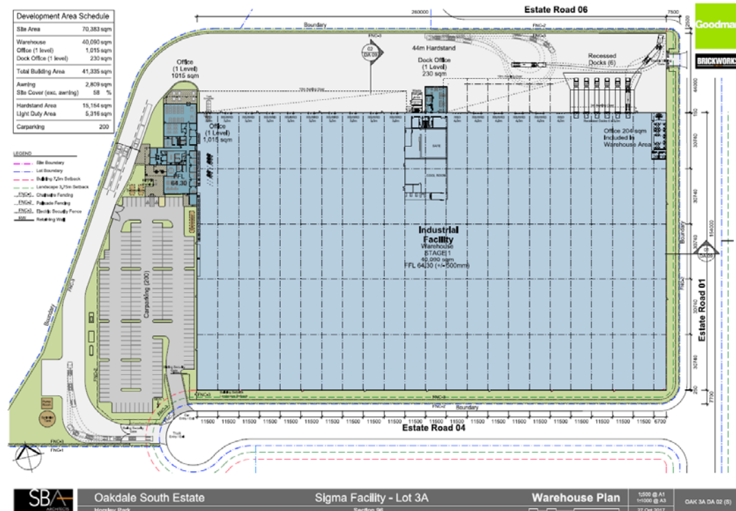
Figure 2: Proposed Lot 3A Development Layout
