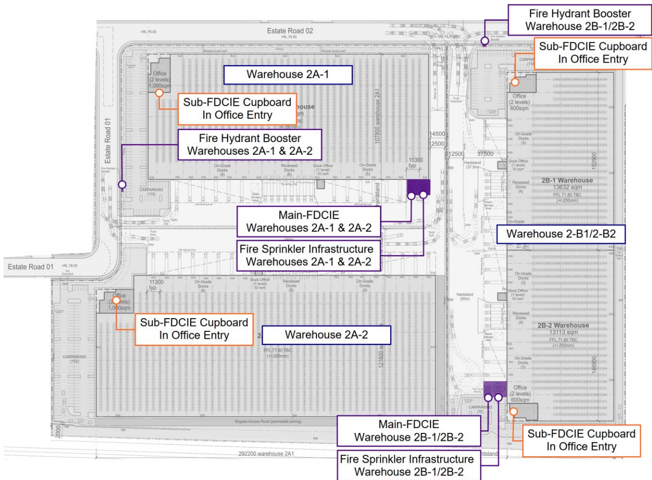
Figure 7-1: Site Fire Services Overview
