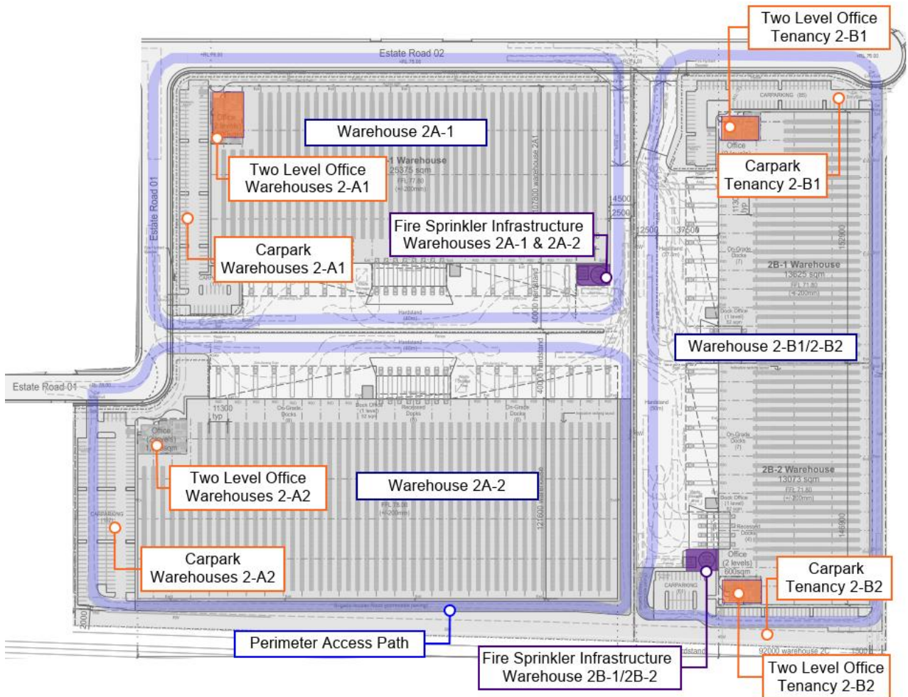
Figure 3-2: Precinct 2 Site Plan - Key Building Features
