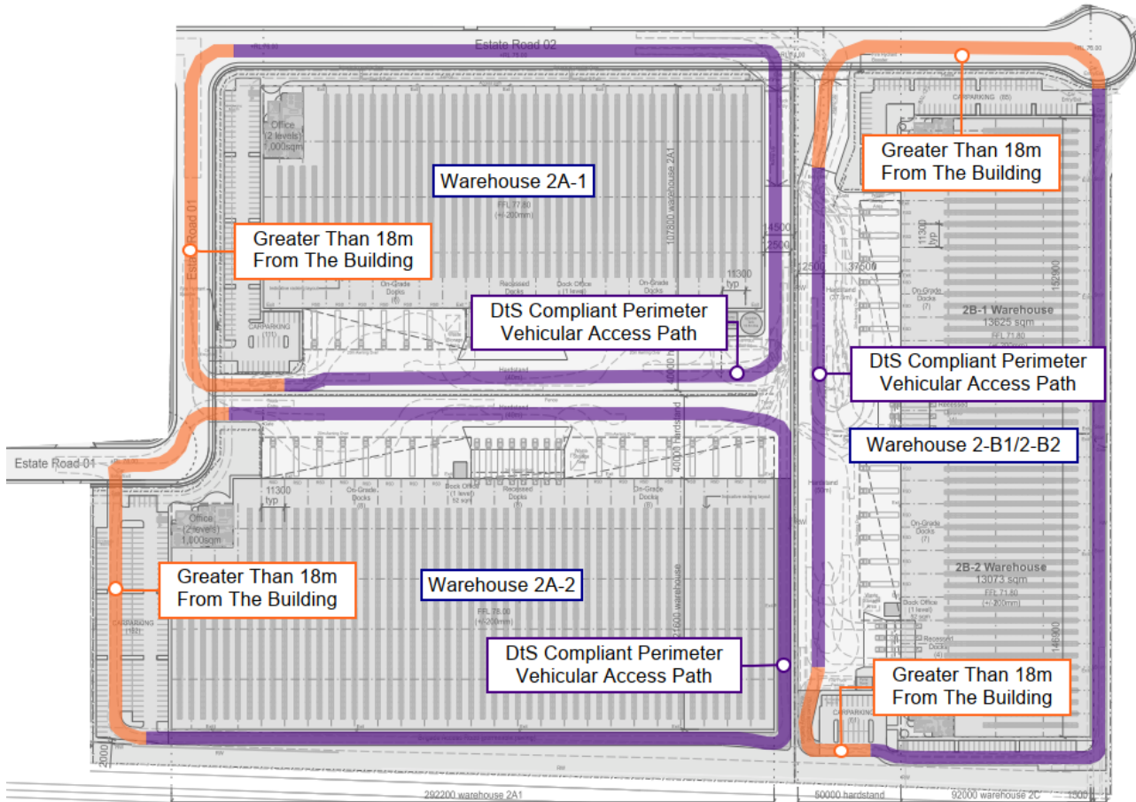
Figure 7-5: Vehicular Perimeter Access Roadway around each Building – Areas of Non-Compliance Highlighted
