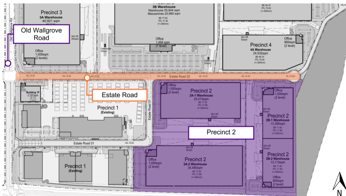
Figure 3-1: Allotment Location relative to Existing Local Setting
