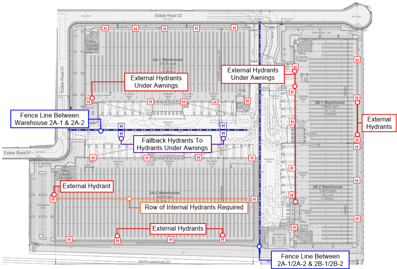
Figure 7-4: Indicative Locations of Fire Hydrants to Serve each Building (example only)
