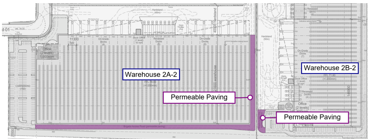
Figure 7-6: Proposed Section of Permeable Paving
