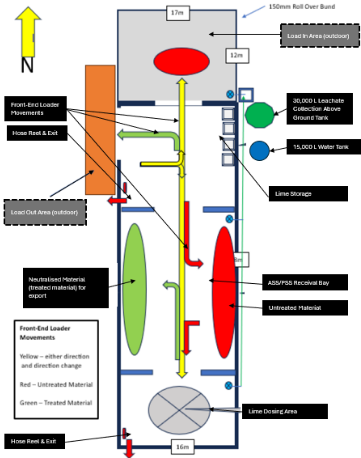
Figure 2 Mag Shed building layout and alterations for AASS/PASS processing activities (outdoor areas are labelled in grey)
