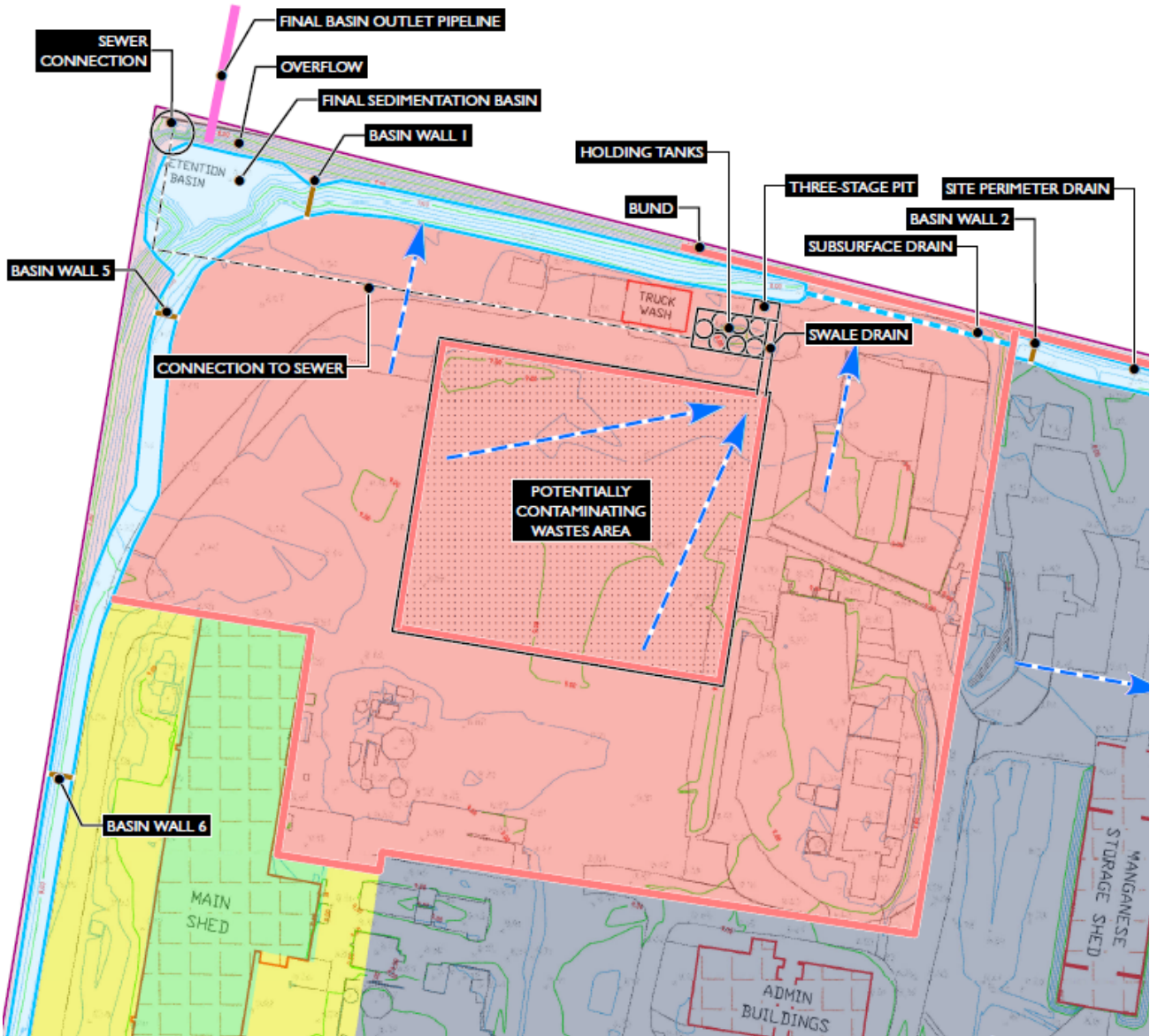
Figure 4 Location of Surface Water Management Infrastructure
