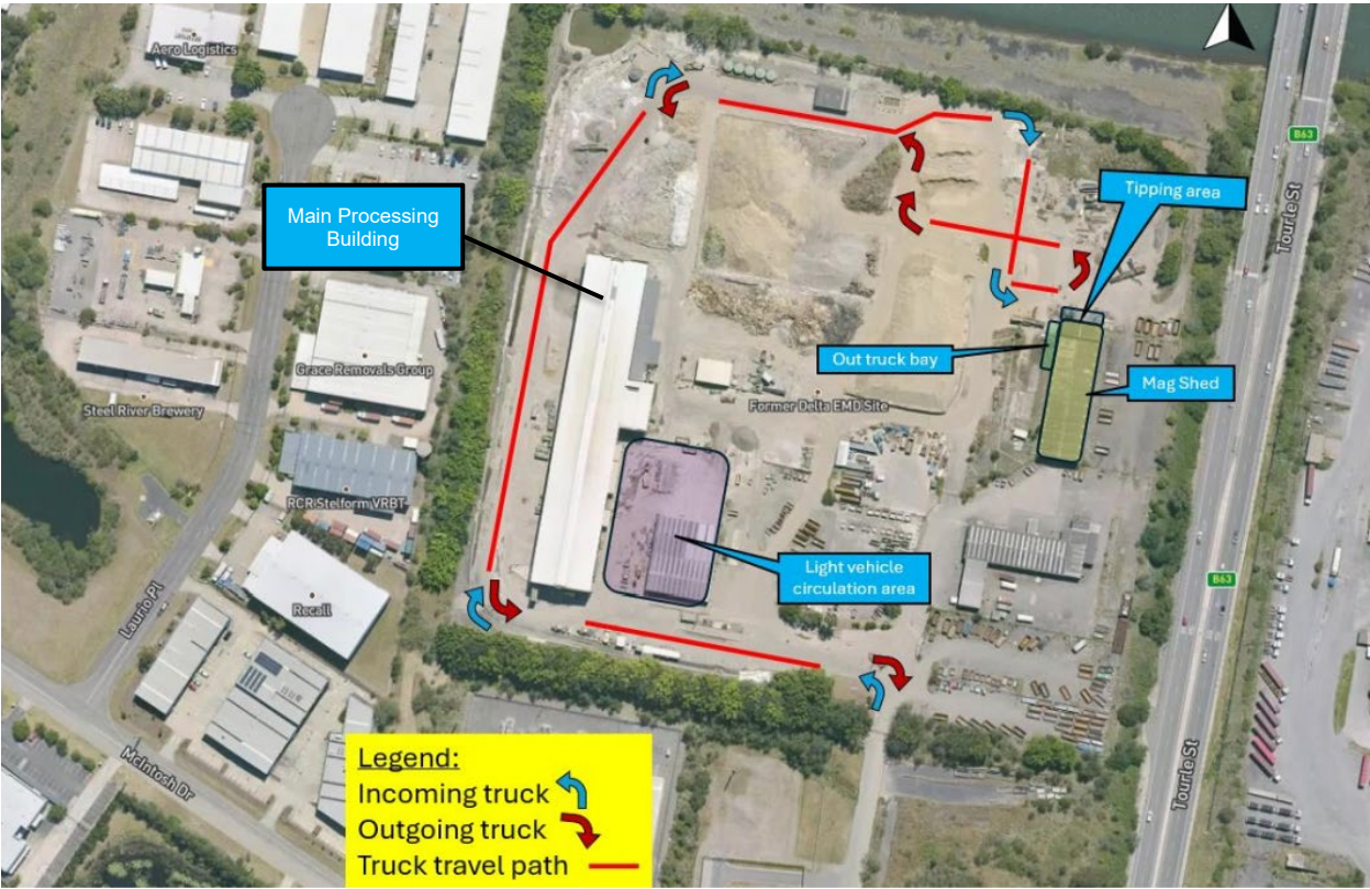
Figure 3 Truck Circulation Plan
