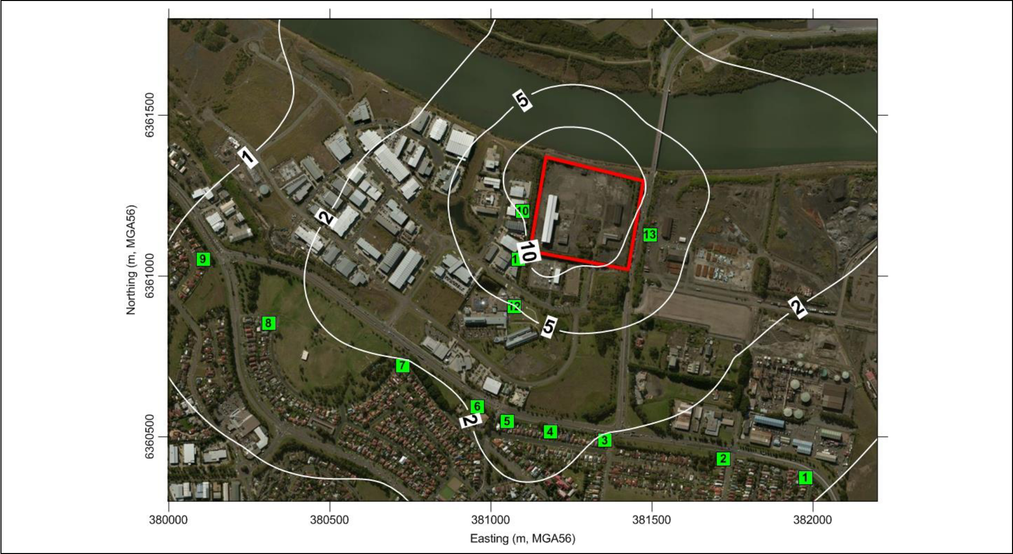
Figure A3.2 Predicted Incremental Maximum 24-hour Average PM 10 Concentrations (µg/m 3 )
