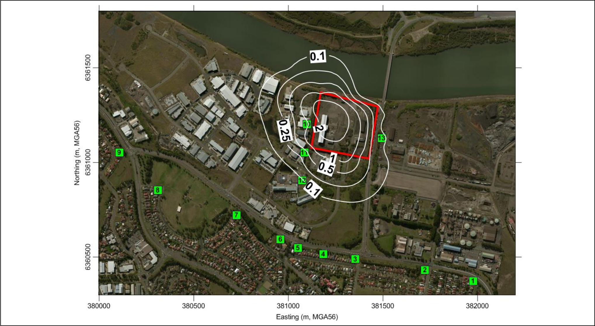
Figure A3.6 Predicted Incremental Annual Average Dust Deposition Levels (g/m²/month)
