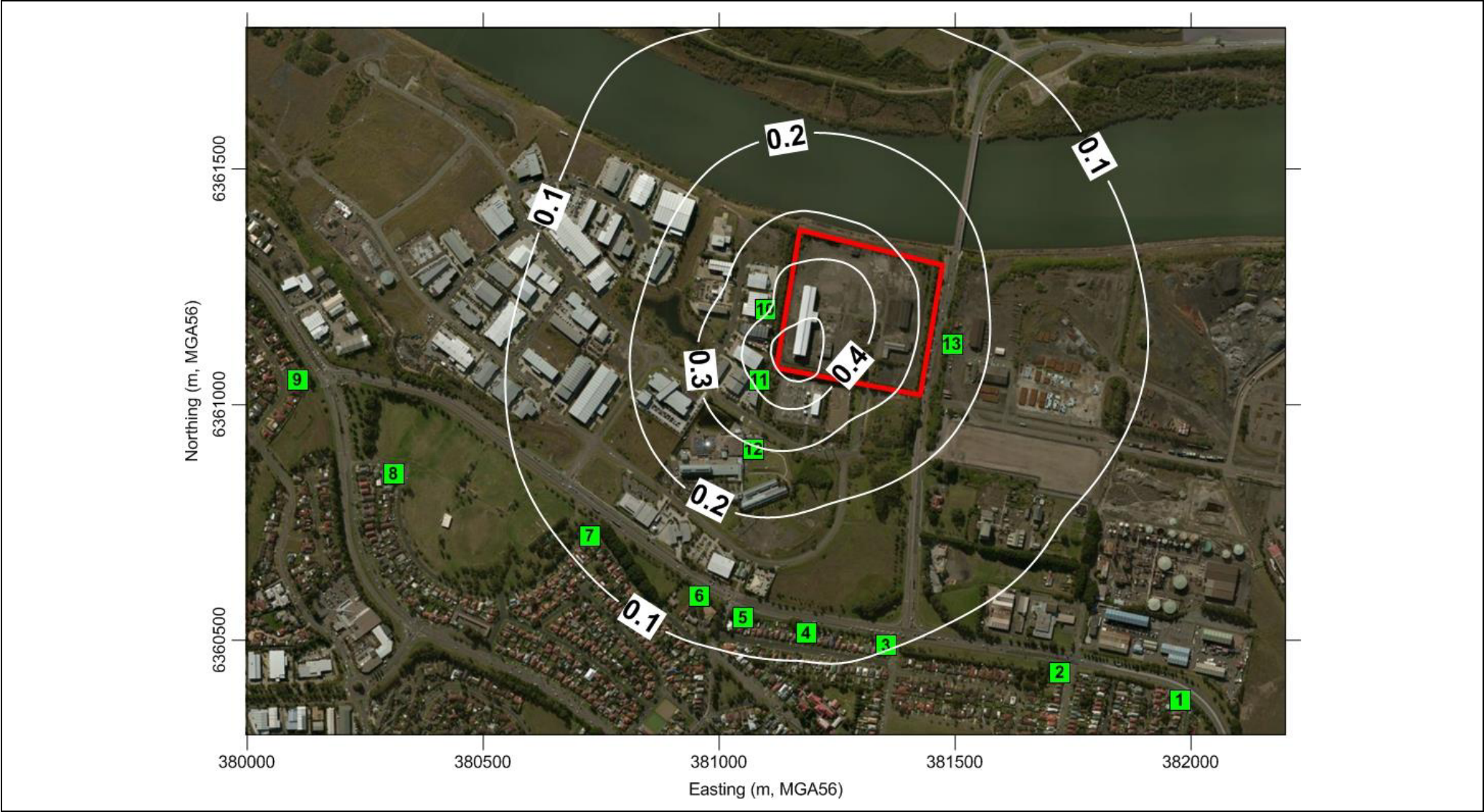
Figure A3.7 Predicted Incremental 99 th Percentile 1-second Average Odour Concentrations (OU)
