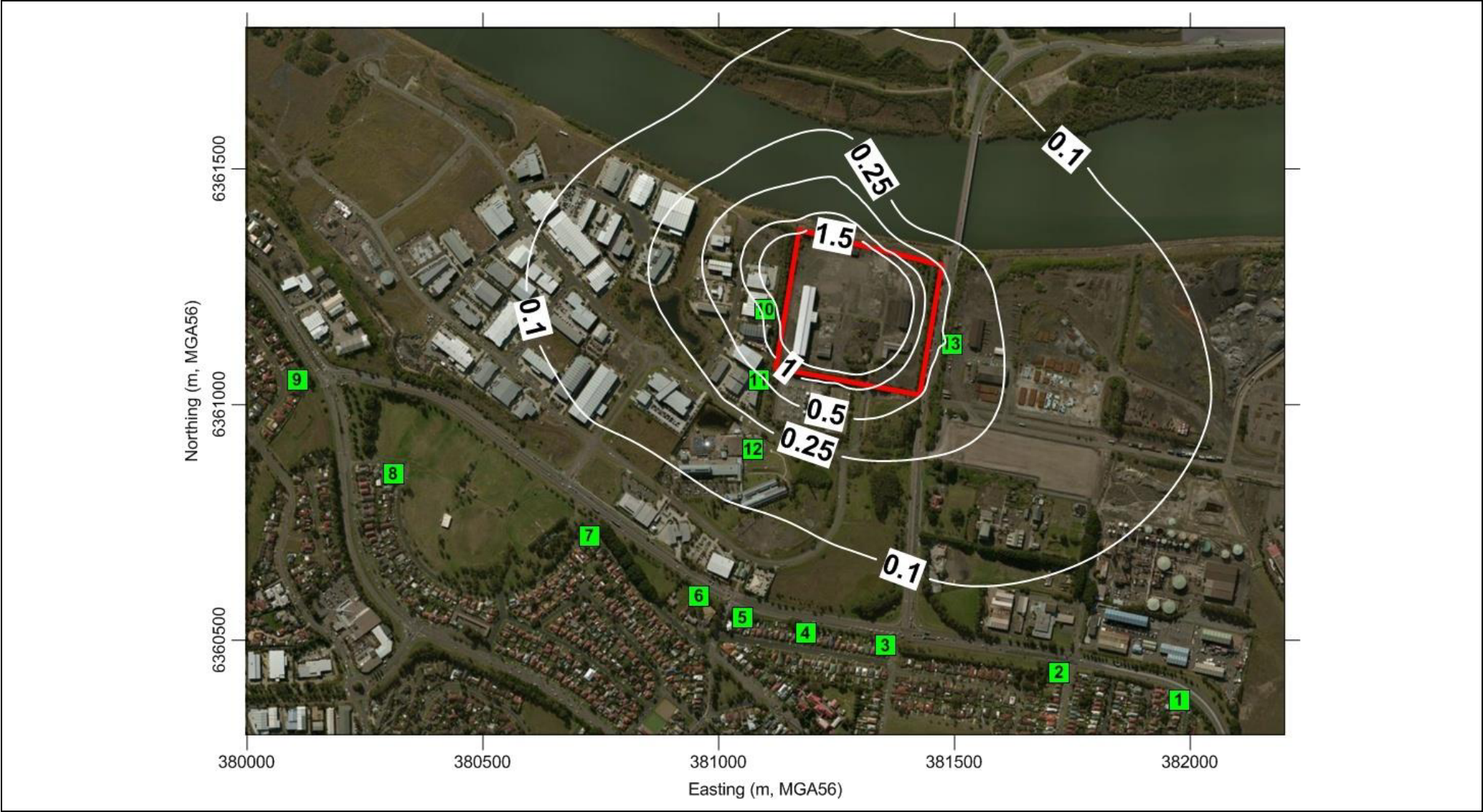
Figure A3.5 Predicted Incremental Annual Average PM 2.5 Concentrations (µg/m 3 )
