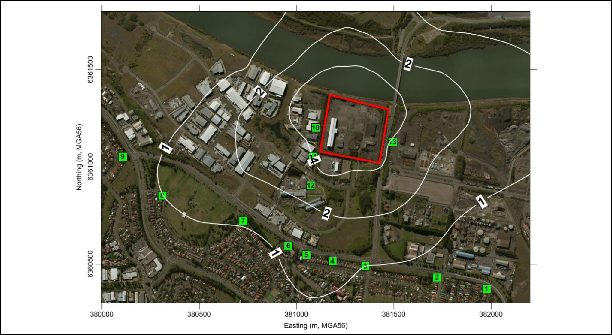
Figure A3.4 Predicted Incremental Maximum 24-hour Average PM 2.5 Concentrations (µg/m 3 )
