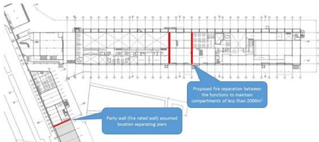
Figure 13: Wharf 4/5 Level 1
