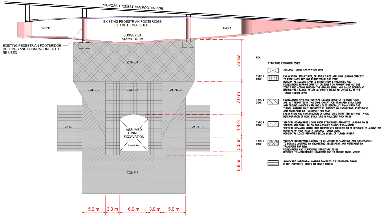
Pedestrian Footbridge over CBDRL Sussex Street Corridor
