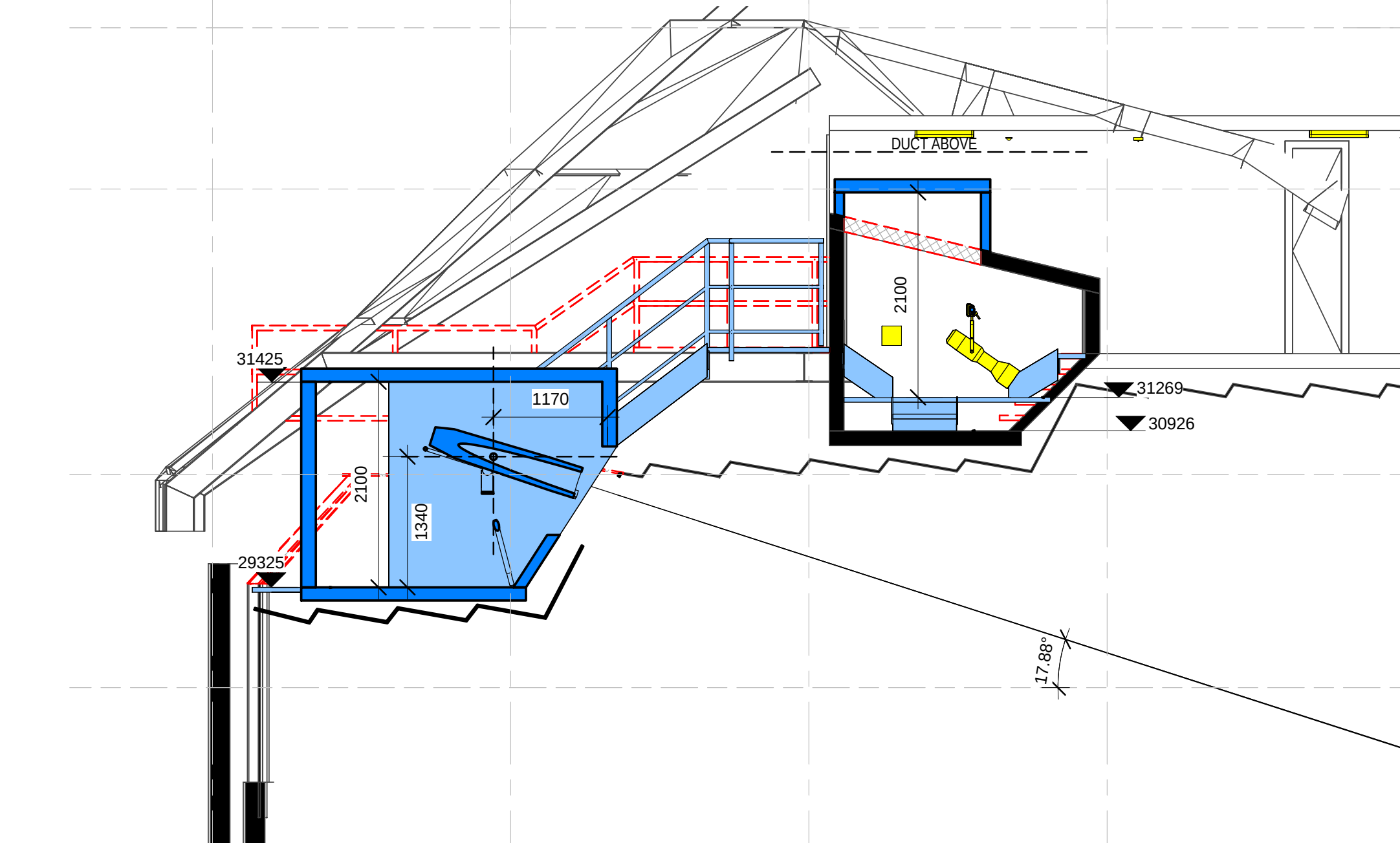
2 SECTION - EXISTING FOLLOW SPOT ROOM 01 -DA 1 : 50
