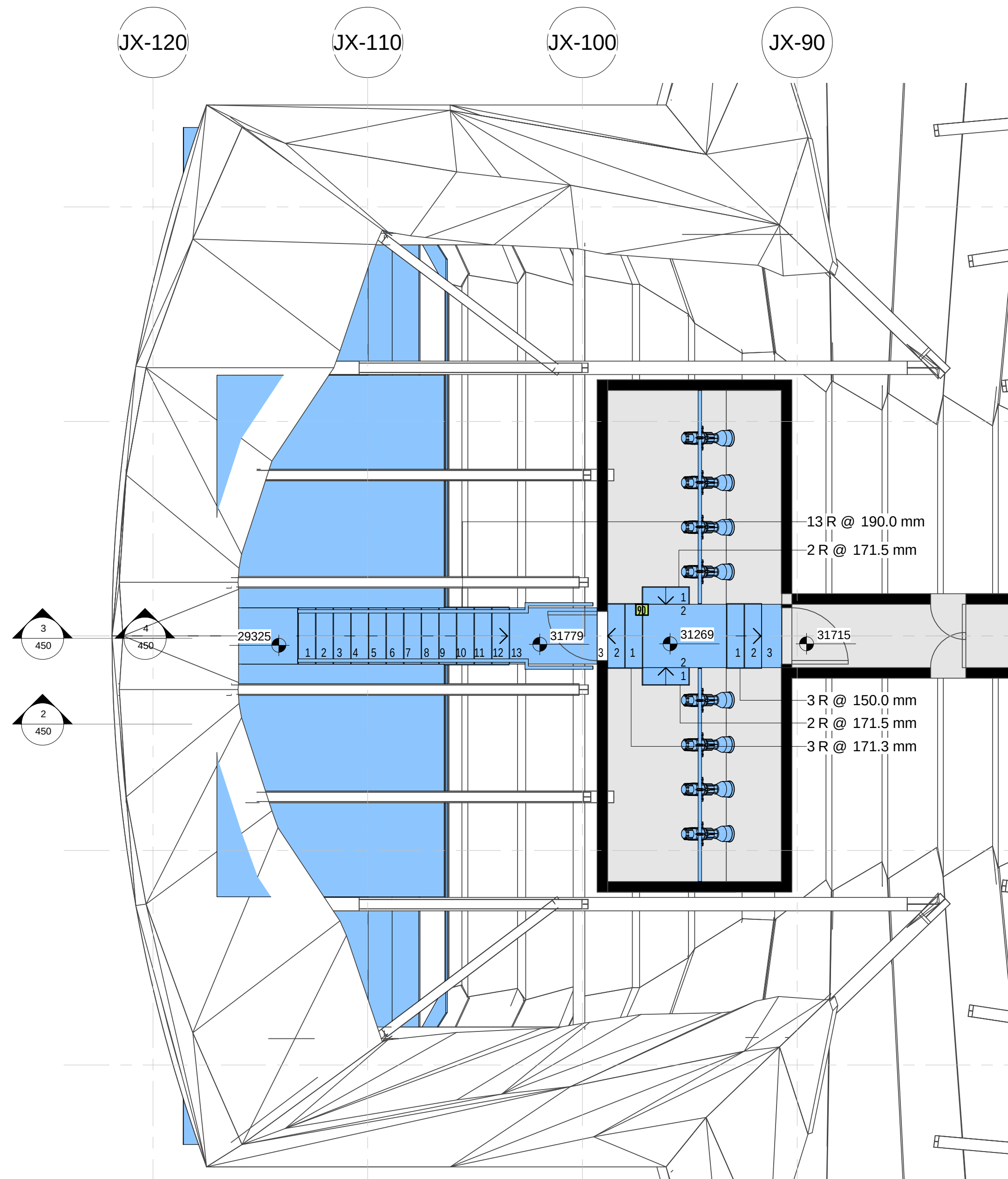
1 PLAN - EXISTING FOLLOW SPOT ROOM - DA 1 : 50
