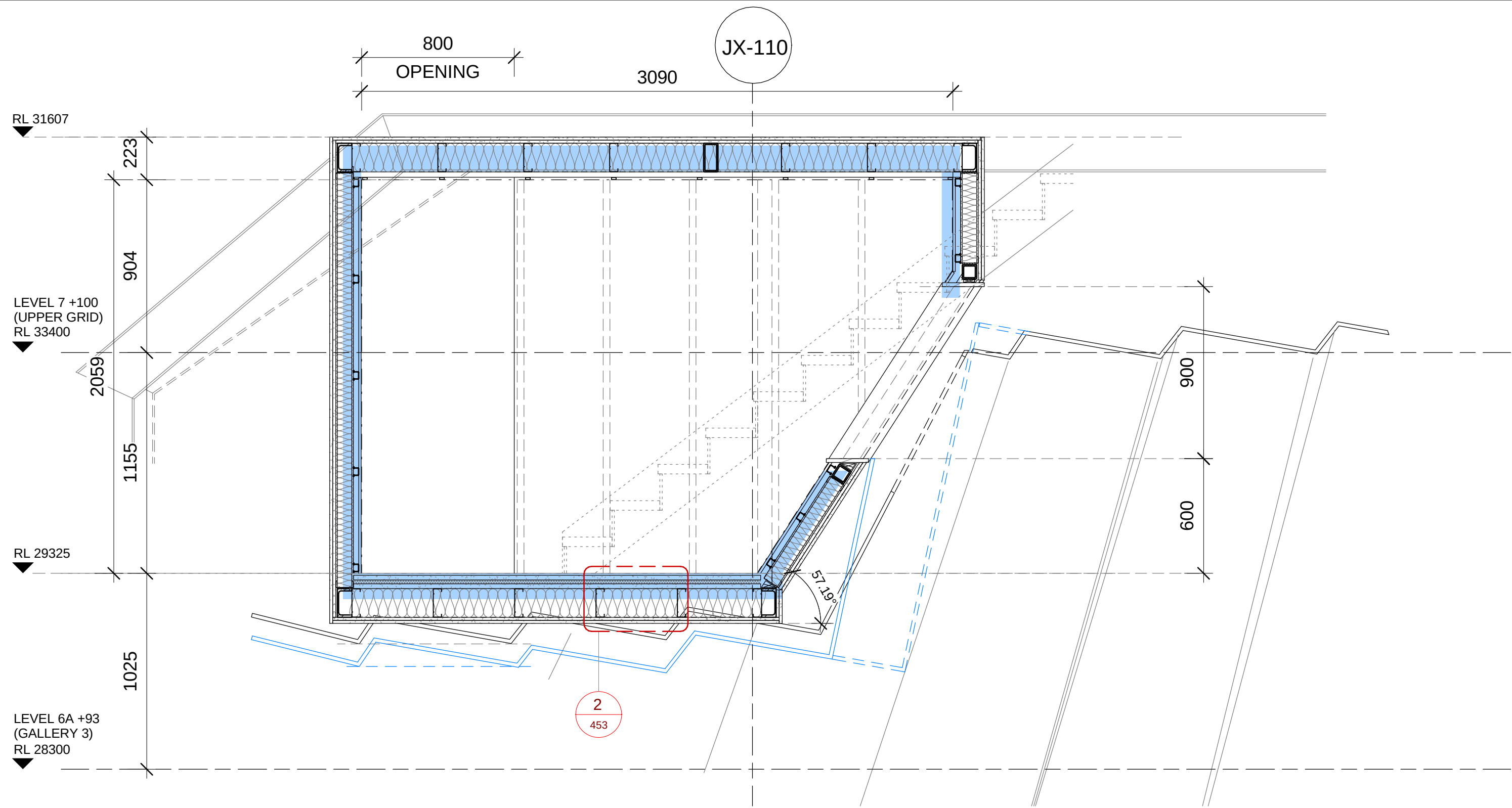
3 SECTION - FSP INTERIOR ELEVATION 2 - DA 1 : 20
