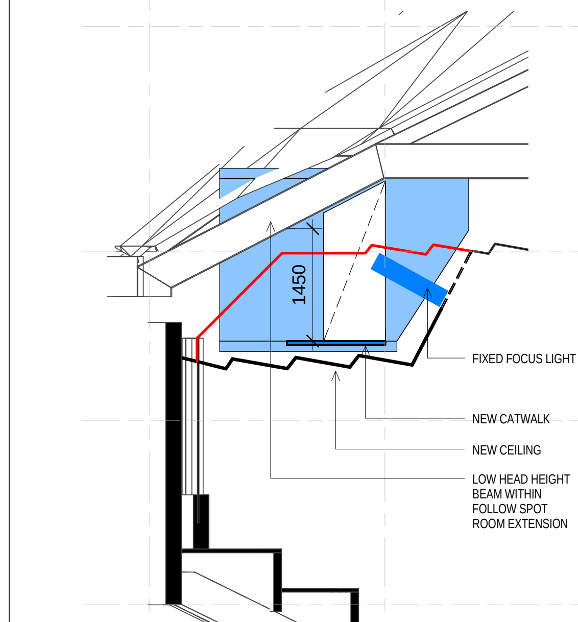
2 SECTION - FOLLOW SPOT ROOM 01 - DA 1 : 50
