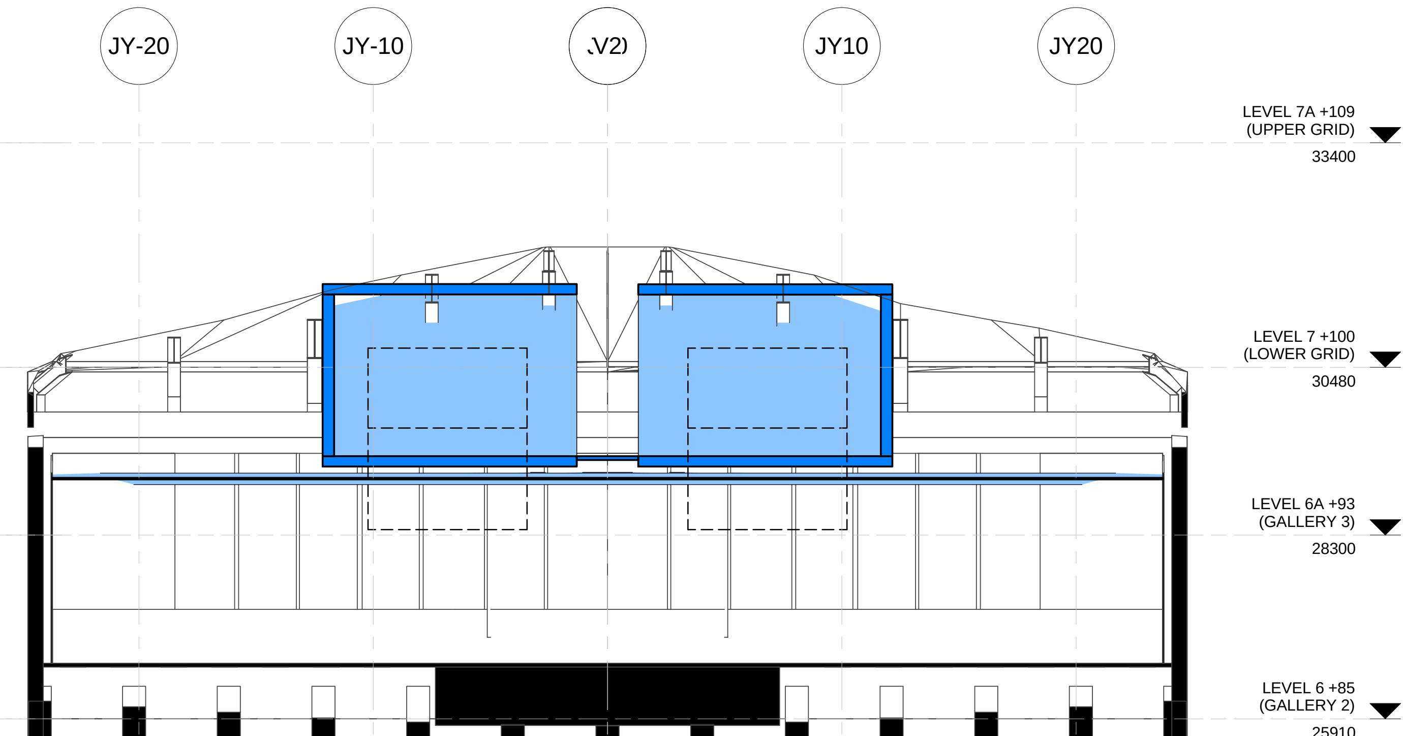
5 SECTION - FOLLOW SPOT ROOM 04 - DA 1 : 50
