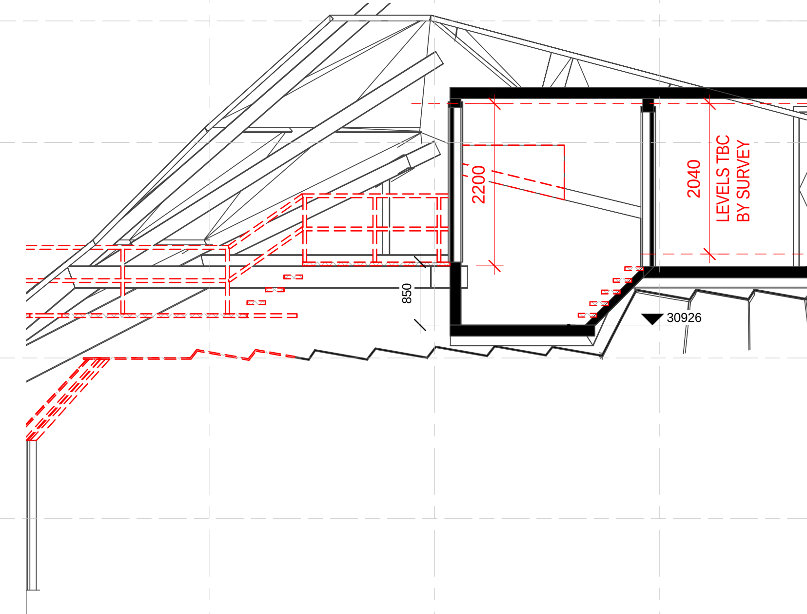
3 SECTION - EXISTING FOLLOW SPOT ROOM 02 - DEMOLITION - DA 1 : 50
