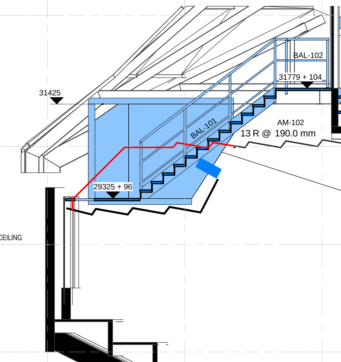
4 SECTION - FOLLOW SPOT ROOM 03 - DA 1 : 50
