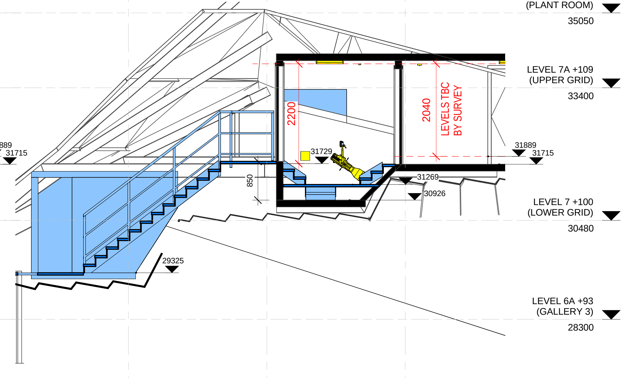
4 SECTION - EXISTING FOLLOW SPOT ROOM 02 - PROPOSED - DA 1 : 50
