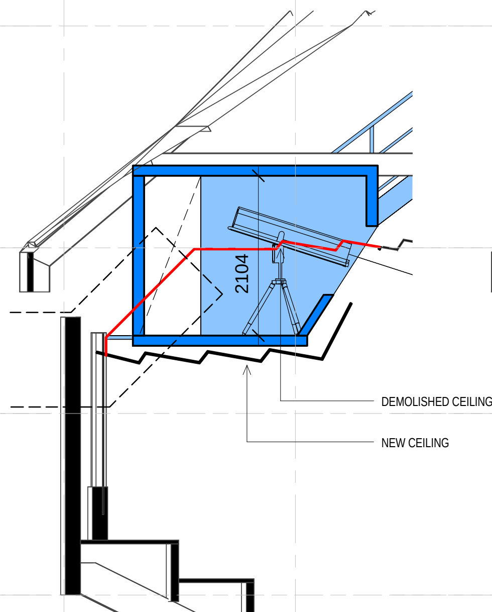
3 SECTION - FOLLOW SPOT ROOM 02 - DA 1 : 50
