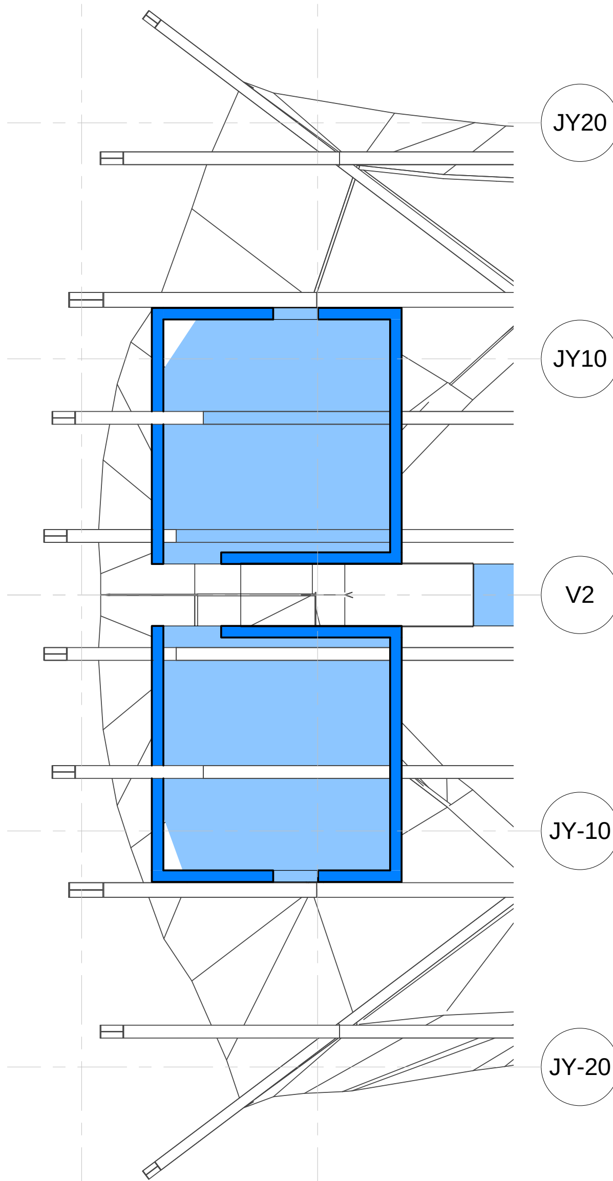
7 RCP - FOLLOW SPOT ROOM - DA 1 : 50
