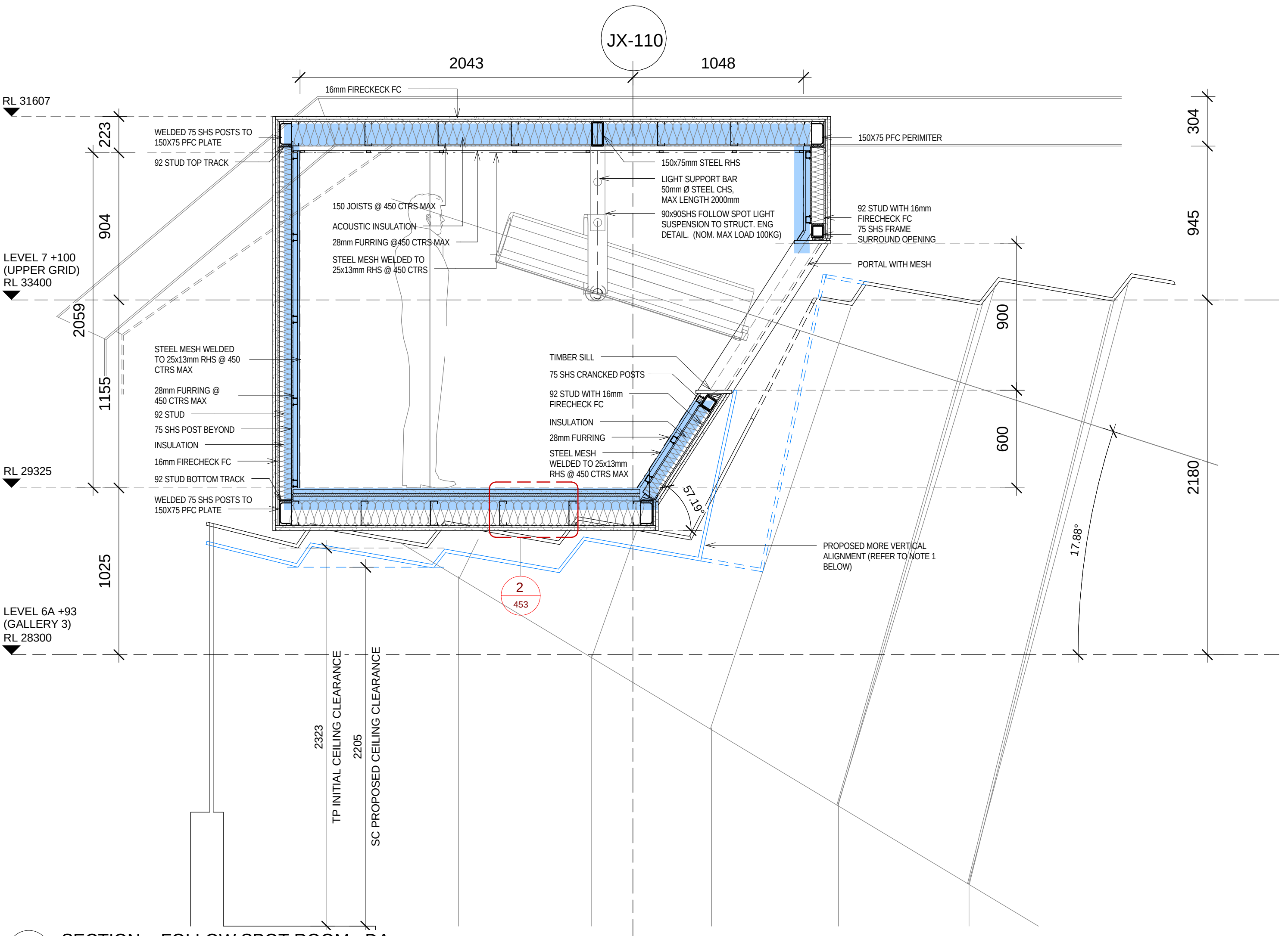
1 SECTION - FOLLOW SPOT ROOM - DA 1 : 20
