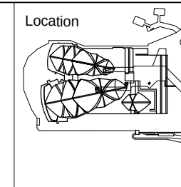
5 SECTION - FOLLOW SPOT ROOM 04 - DA 1 : 50
