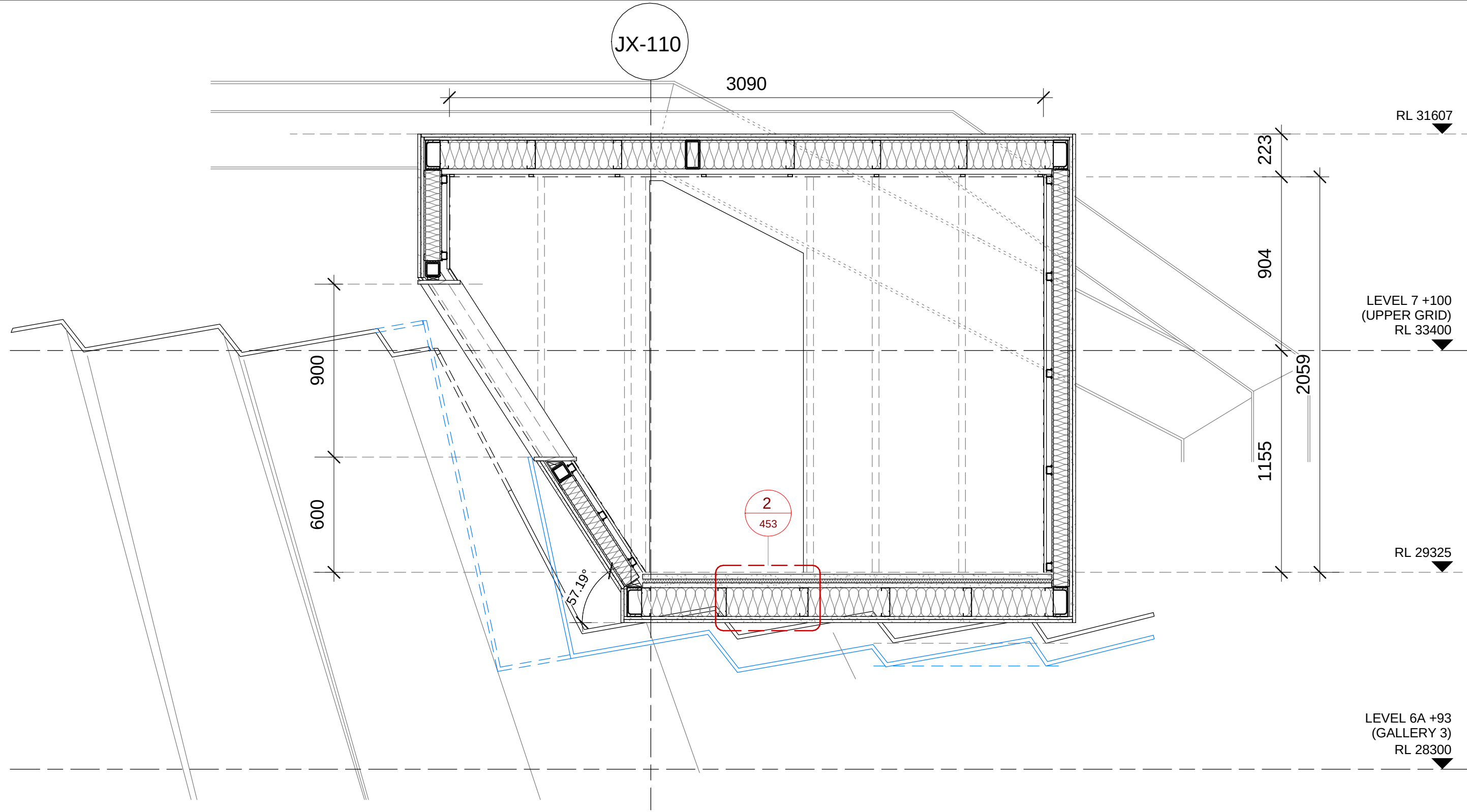
4 SECTION - FSP INTERIOR ELEVATION 1 - DA 1 : 20
