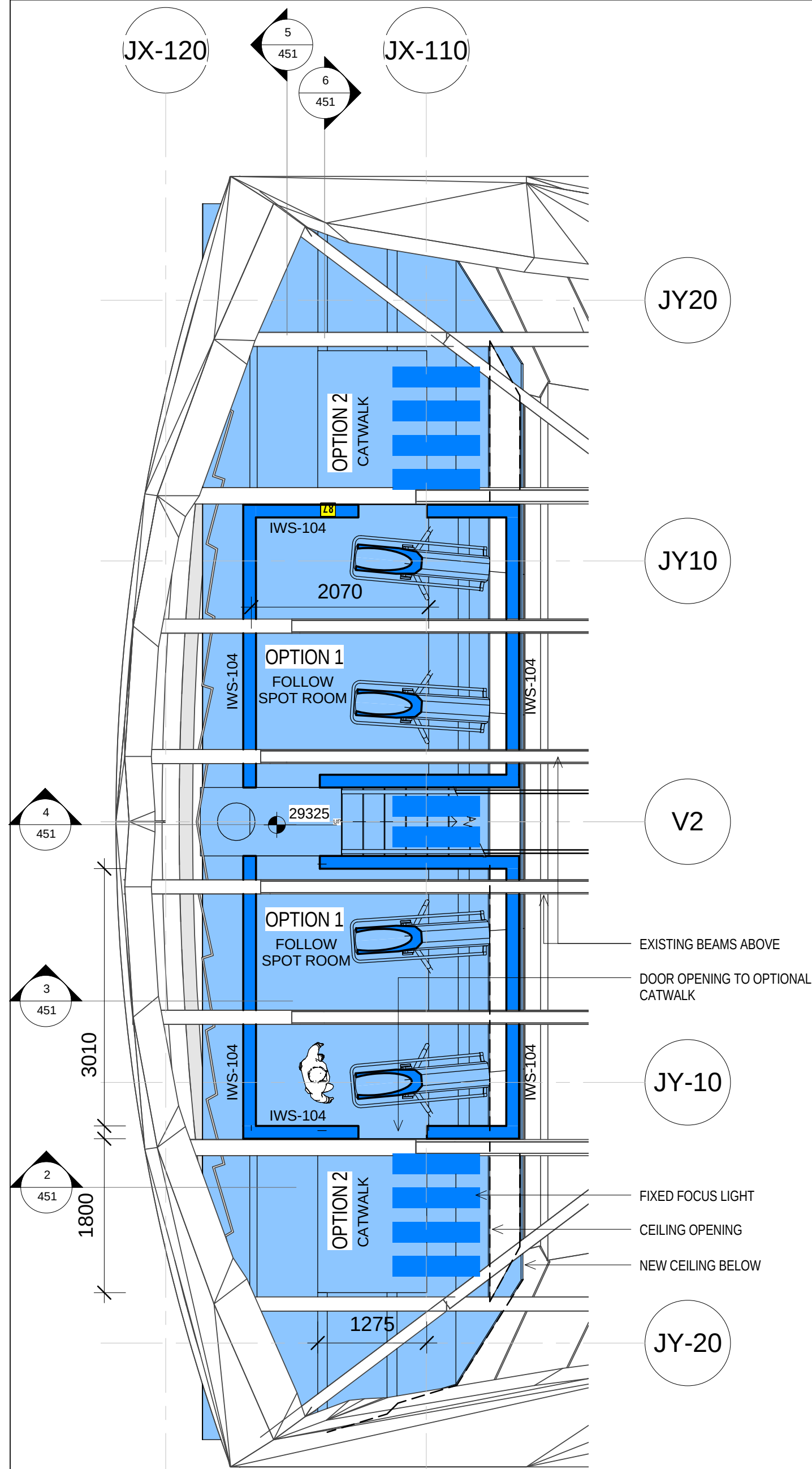
1 PLAN - FOLLOW SPOT ROOM - DA 1 : 50
