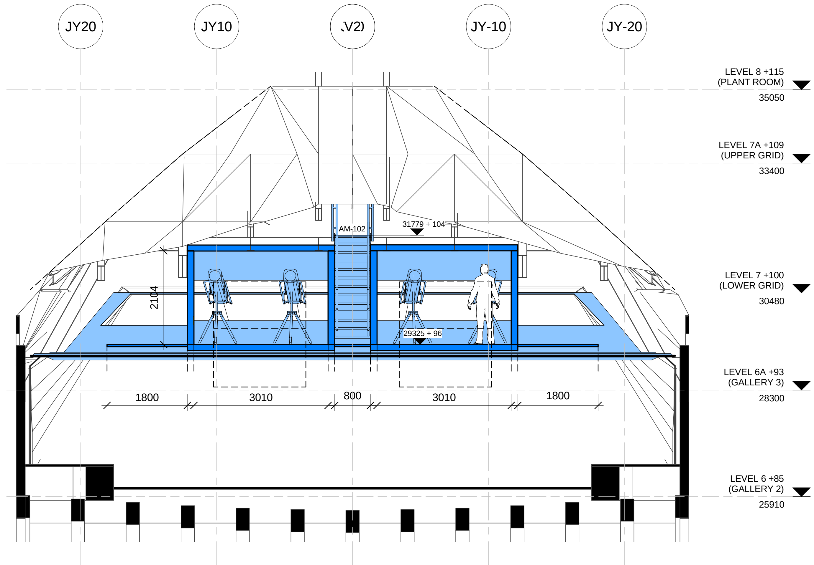
6 SECTION - FOLLOW SPOT ROOM 05 - DA 1 : 50
