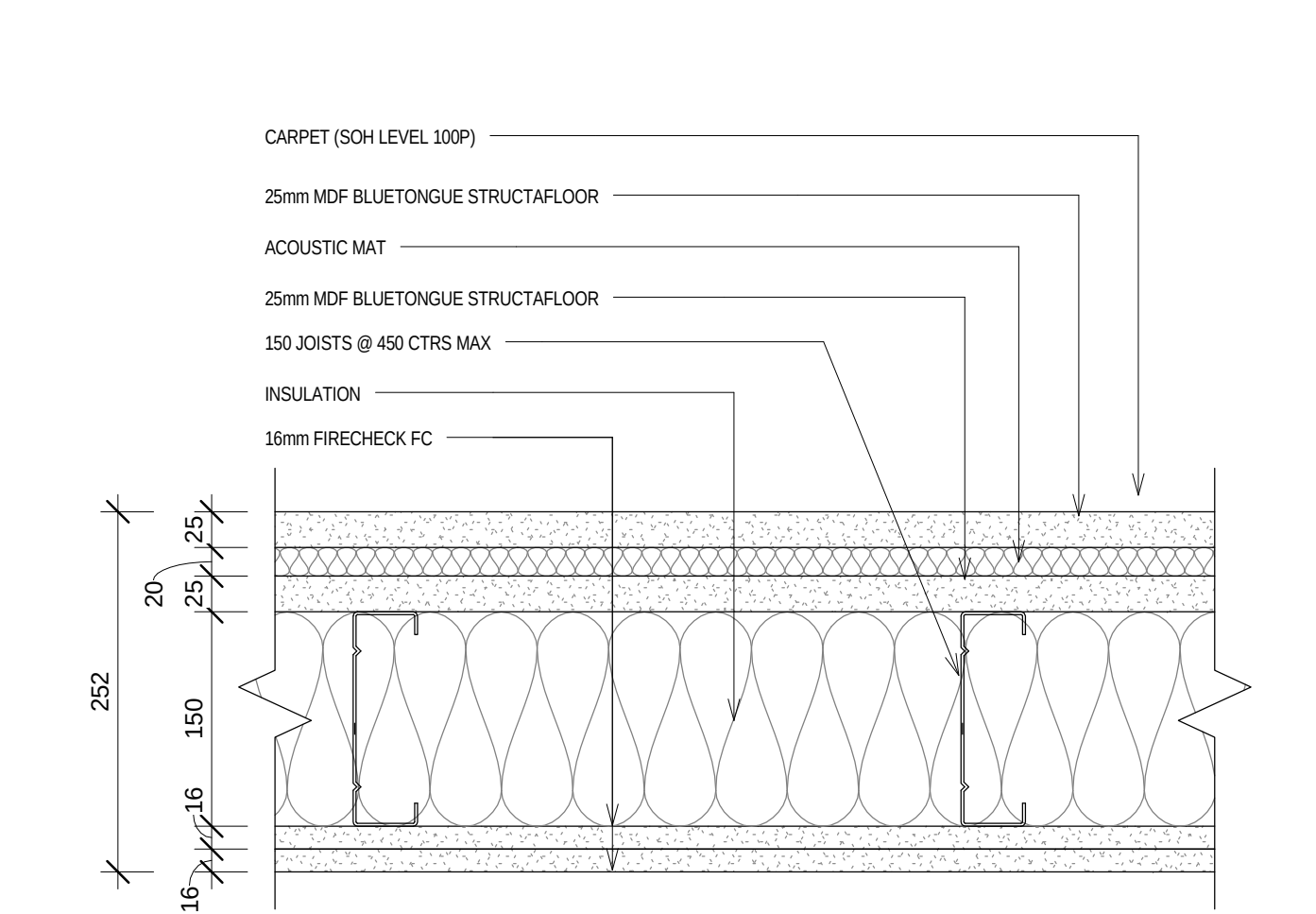
2 SECTION - PROPOSED ACOUSTIC FLOOR CONSTRUCTION - DA 1 : 5
