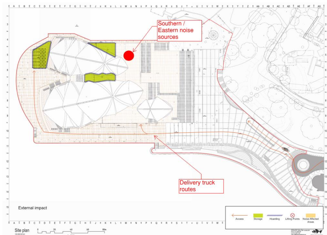
Figure 2 Indicative construction source locations, Sydney Opera House construction works
