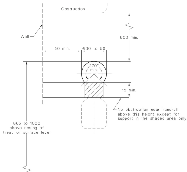
Figure 7: Handrail Details
