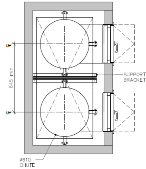
02 DUAL (610Ø) GALV. STEEL CHUTE LAYOUT
