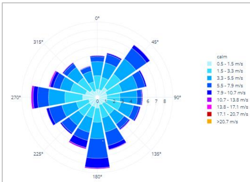
Figure 9. Wind data based on the nearest weather station.
