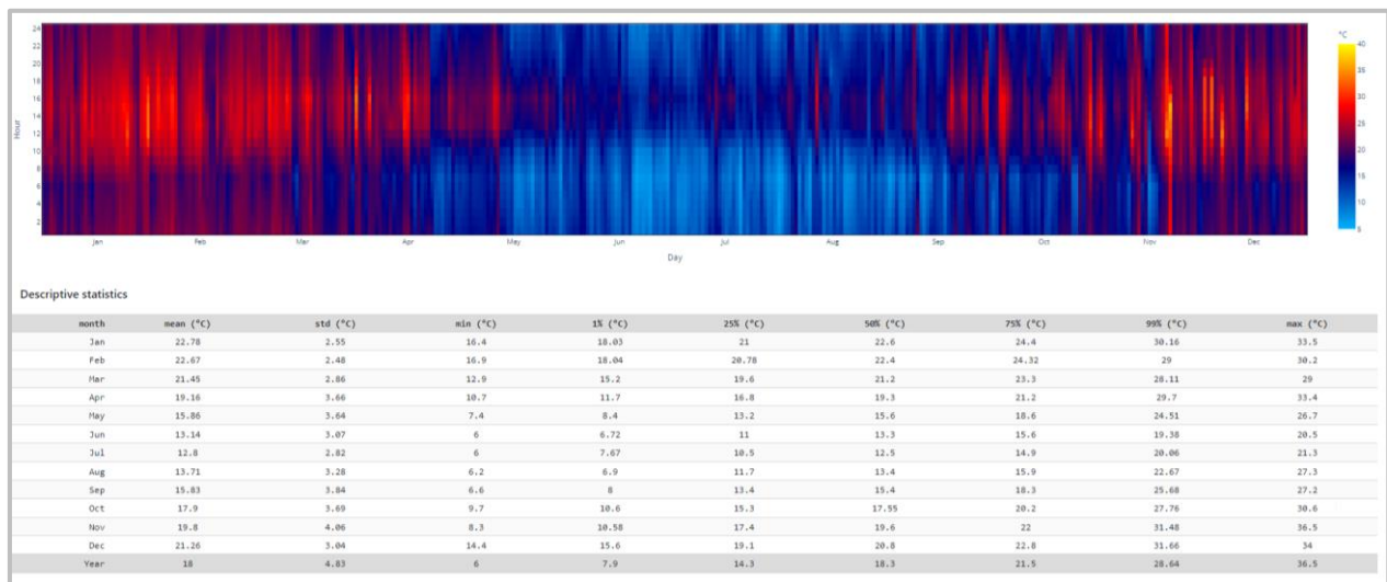
Figure 11. Heatmap Chart.
