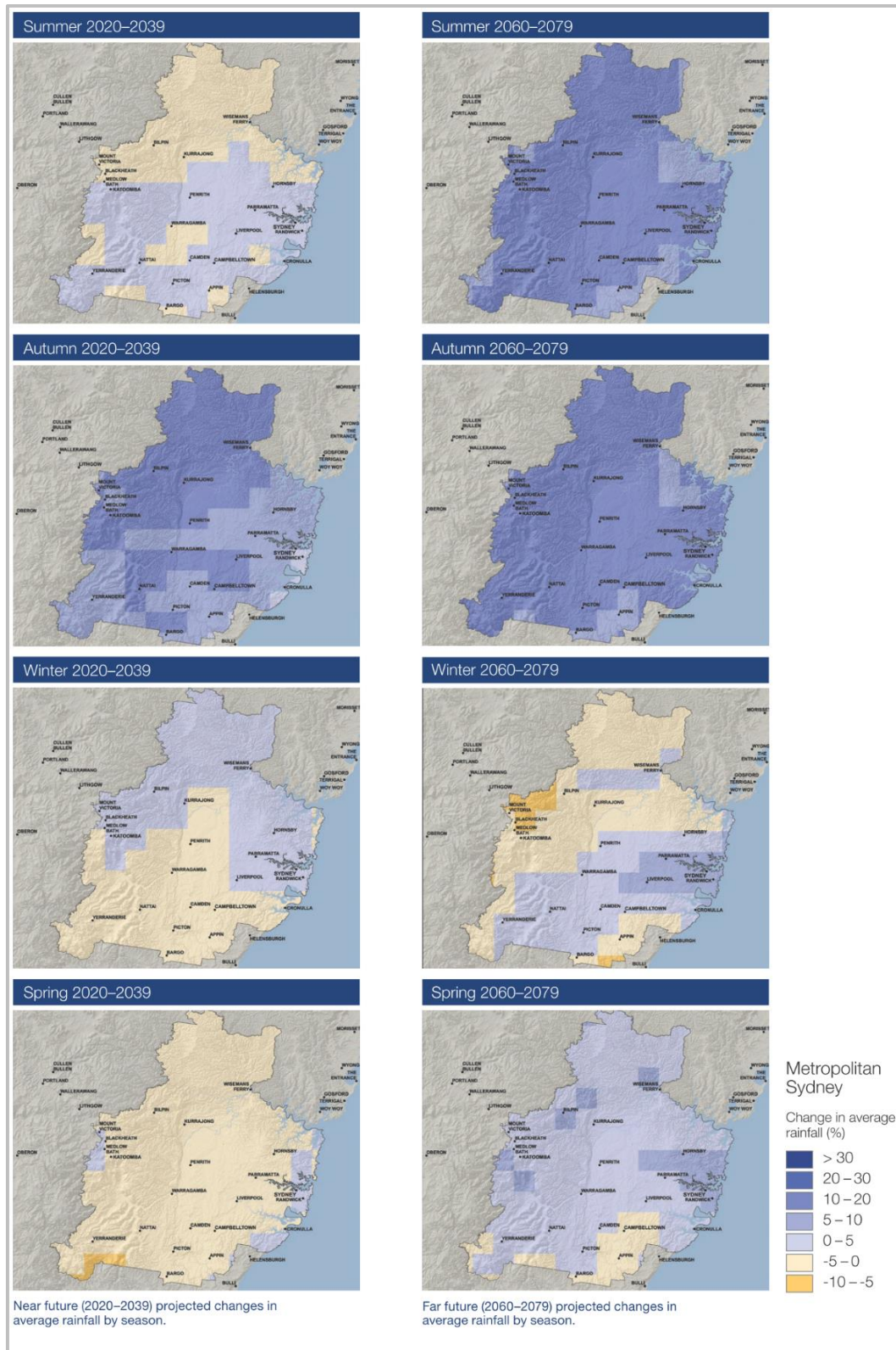
Figure 15. Change in average rainfall (%) – Sydney variation map.
