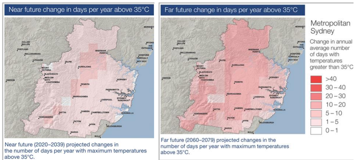
Figure 13. Change in annual average number of days with temperatures greater than 35°C – Sydney variation map.
