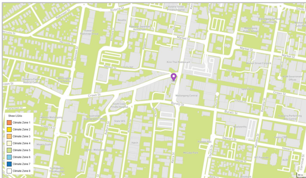
Figure 6. Climate zone map.
