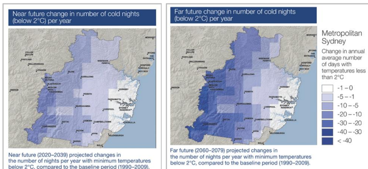
Figure 14. Change in annual average number of days with temperature less than 2°C – Sydney variation map.
