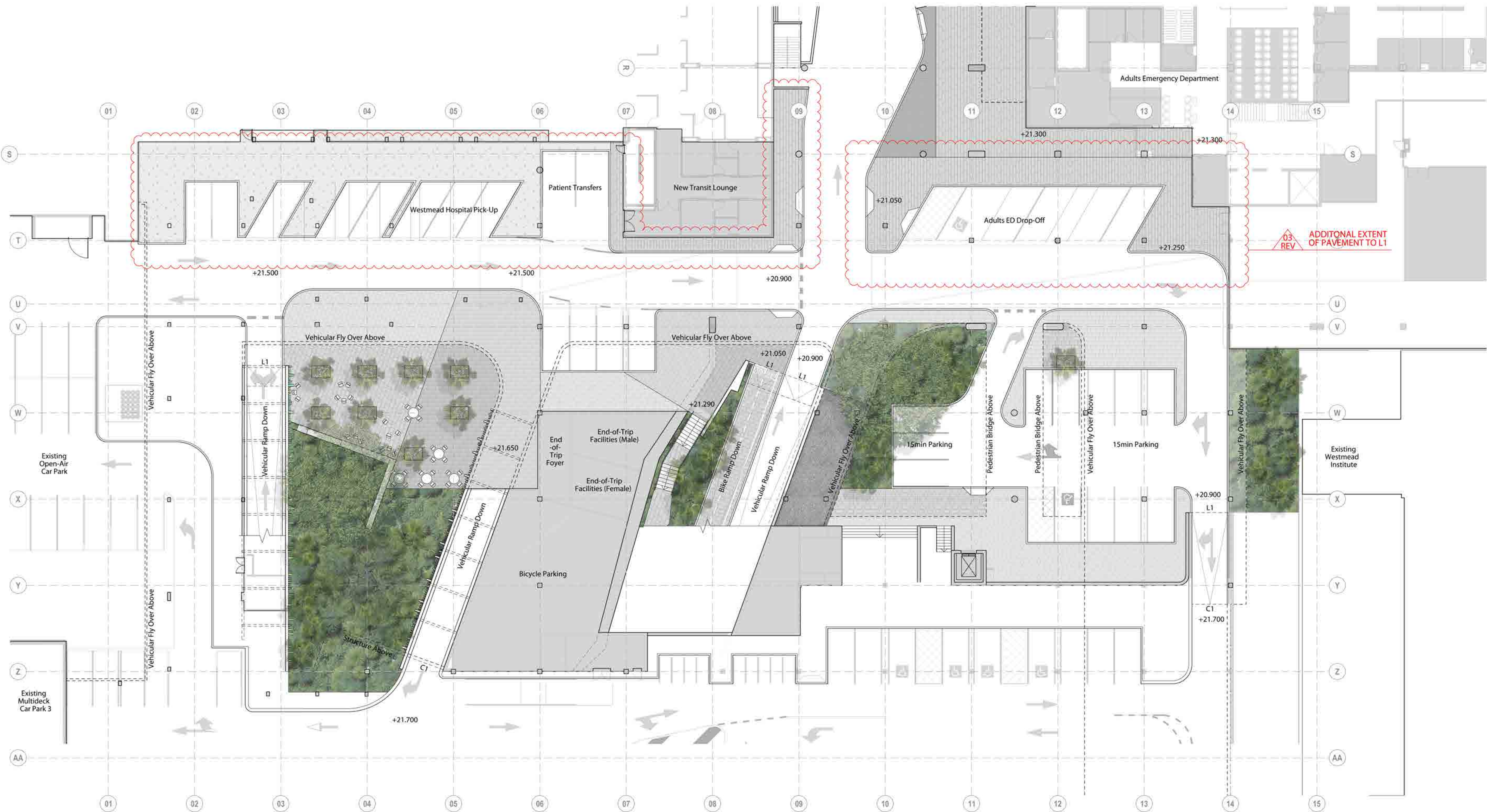
1 Landscape Plan Plaza | Level 1
