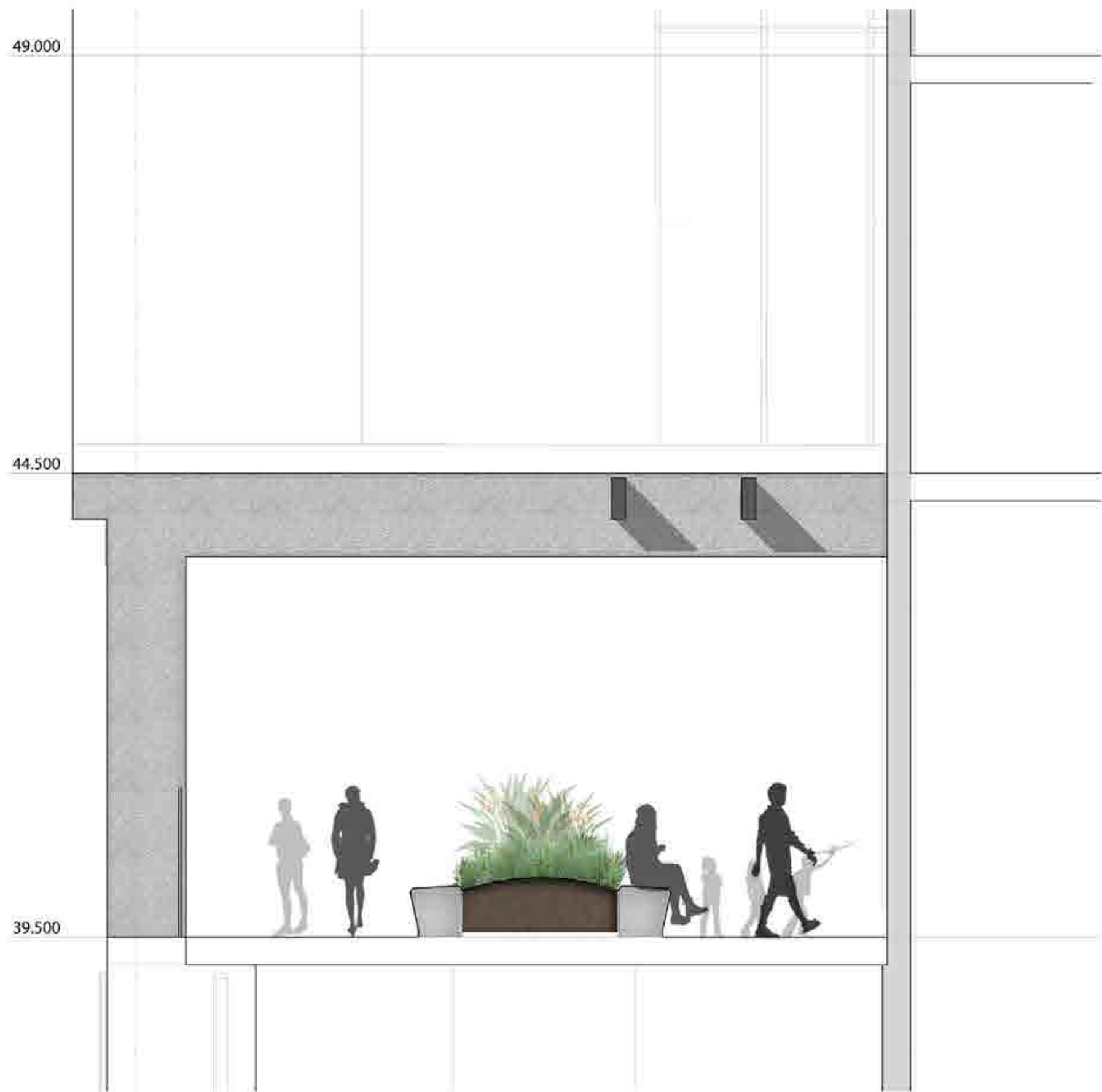
2 Level 5 Auditorium Courtyard Landscape Section
