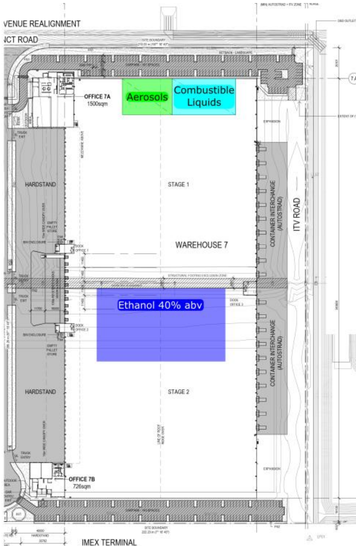
Figure 3-2: Site Layout
