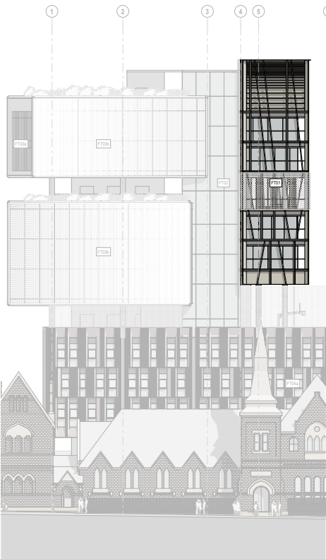
East Elevation
