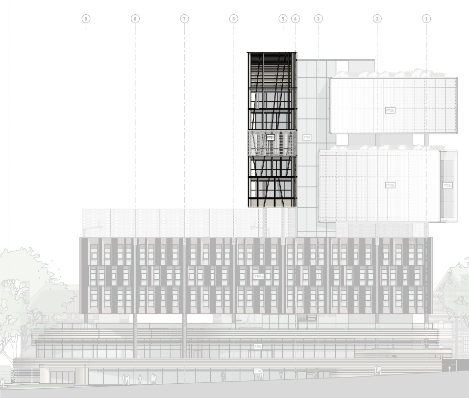
West Elevation
