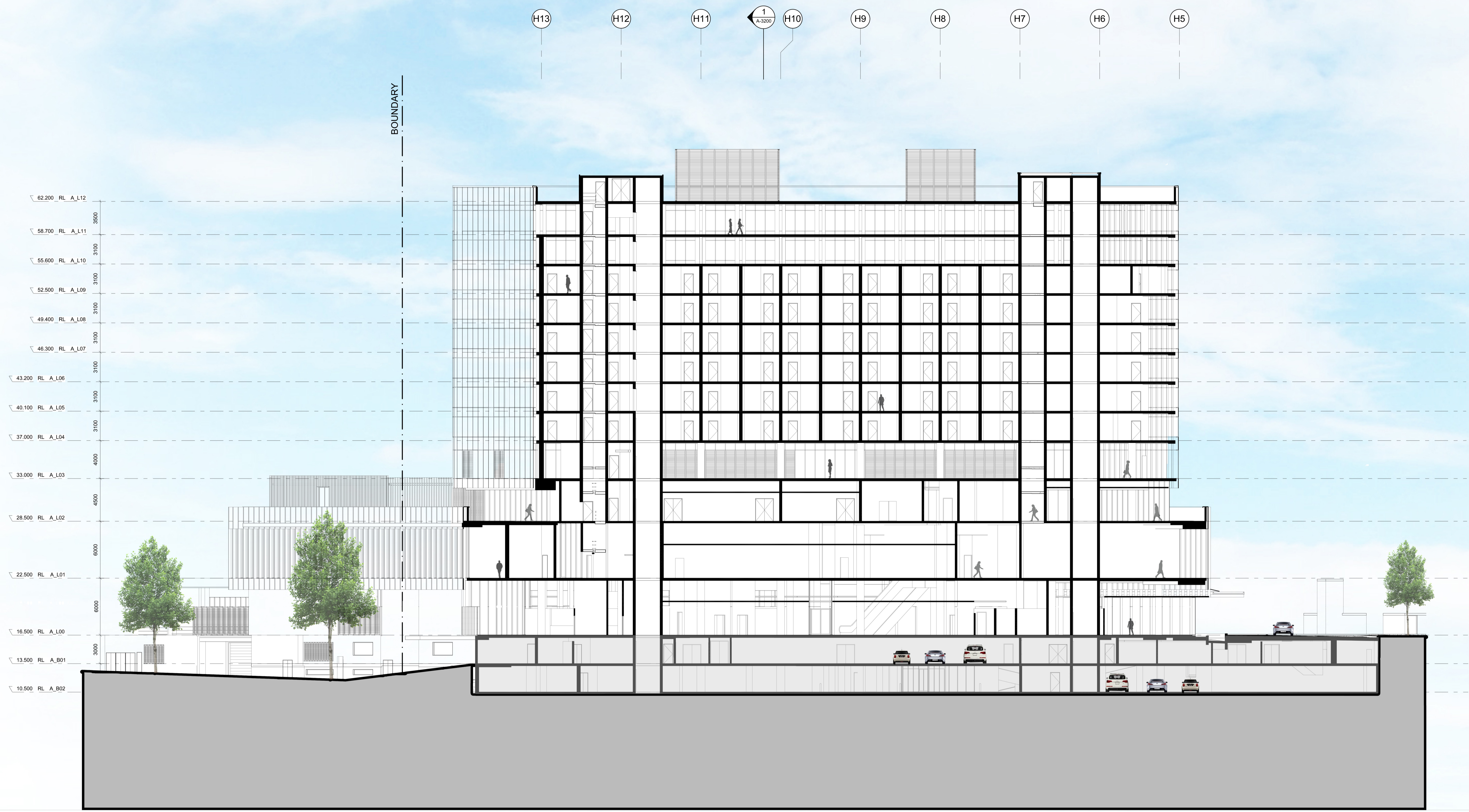
1 BUILDING CROSS SECTION 1 : 200
