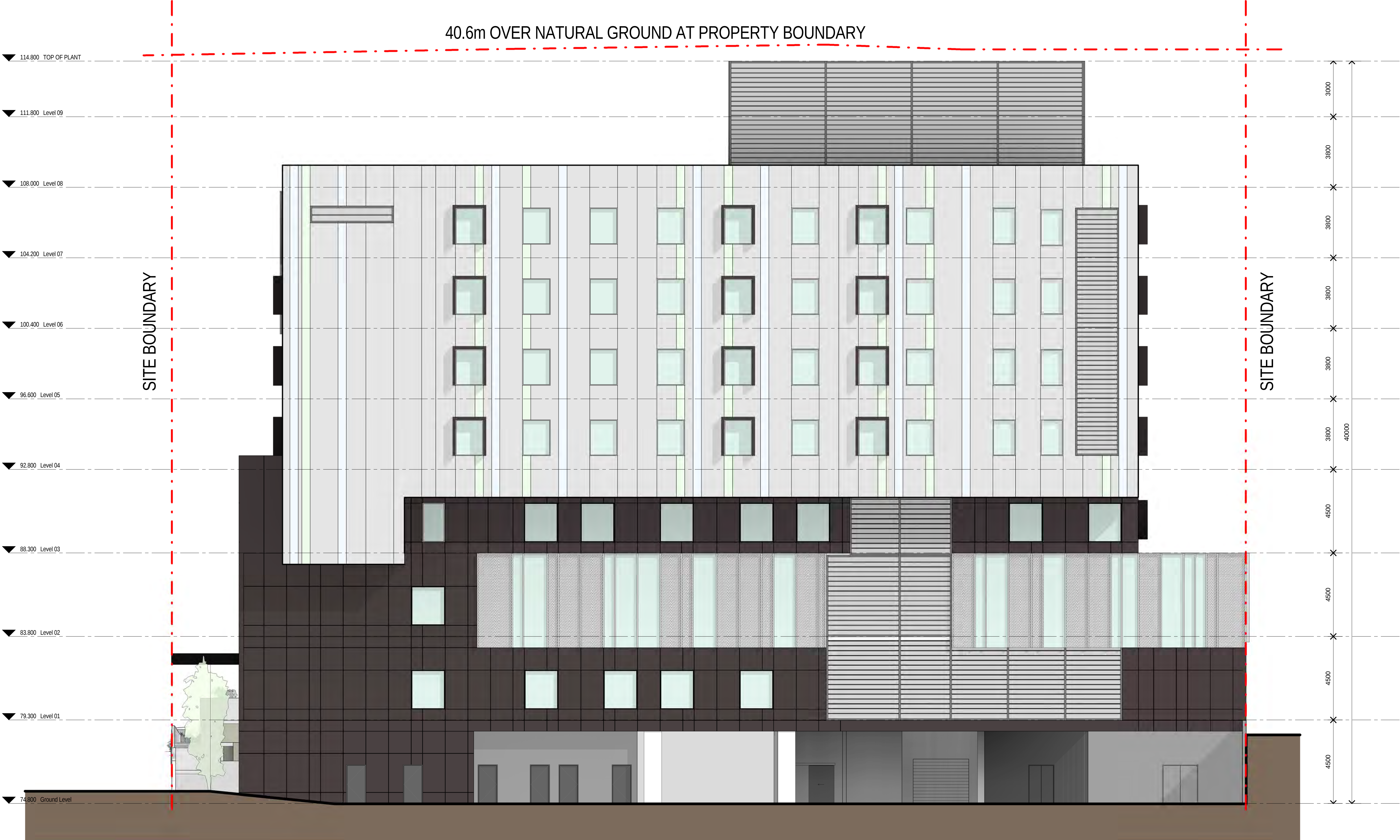
1 ELEVATION WEST 1:100
