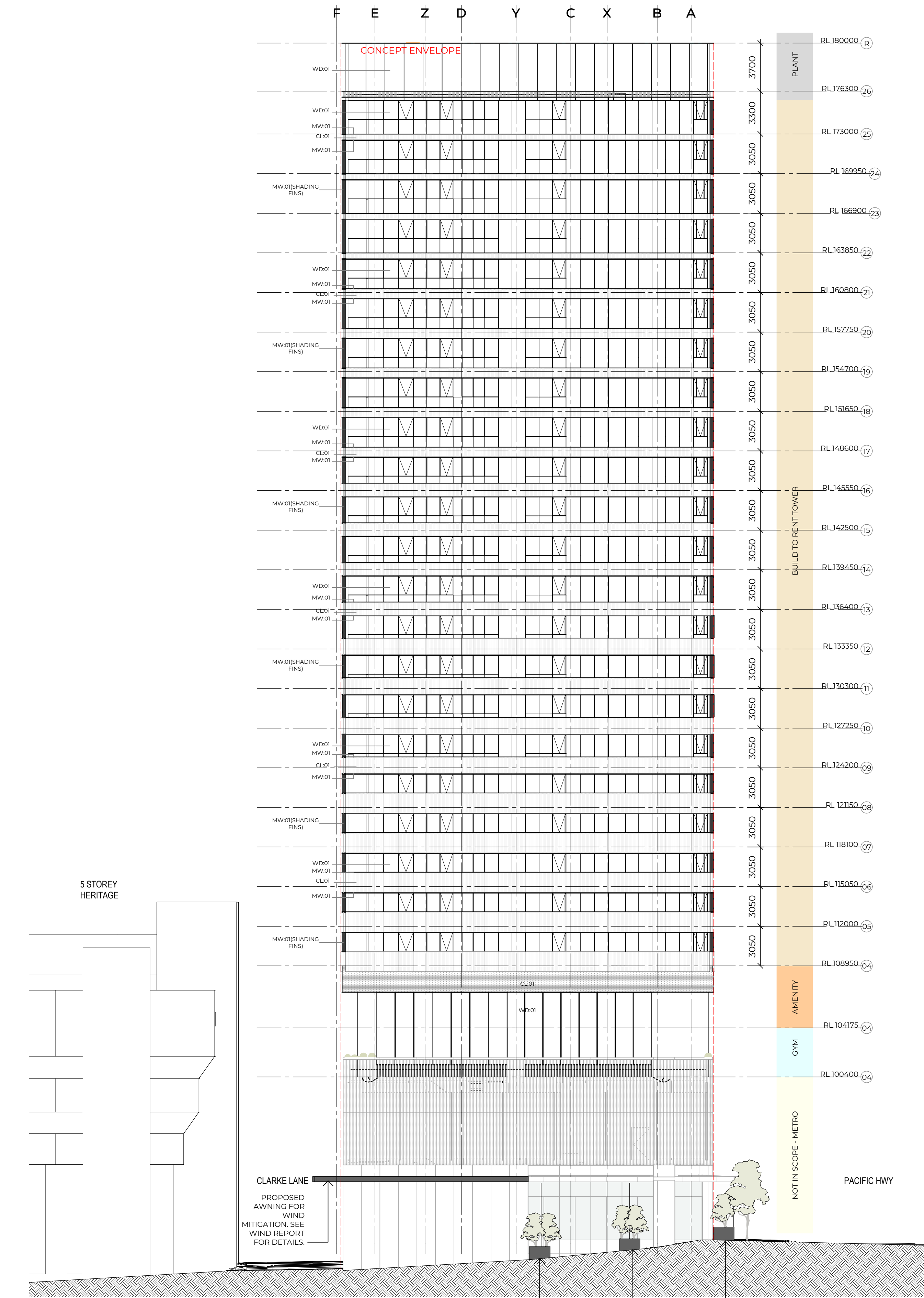
1 OXLEY STREET - PROPOSED ELEVATION SCALE 1 : 200
