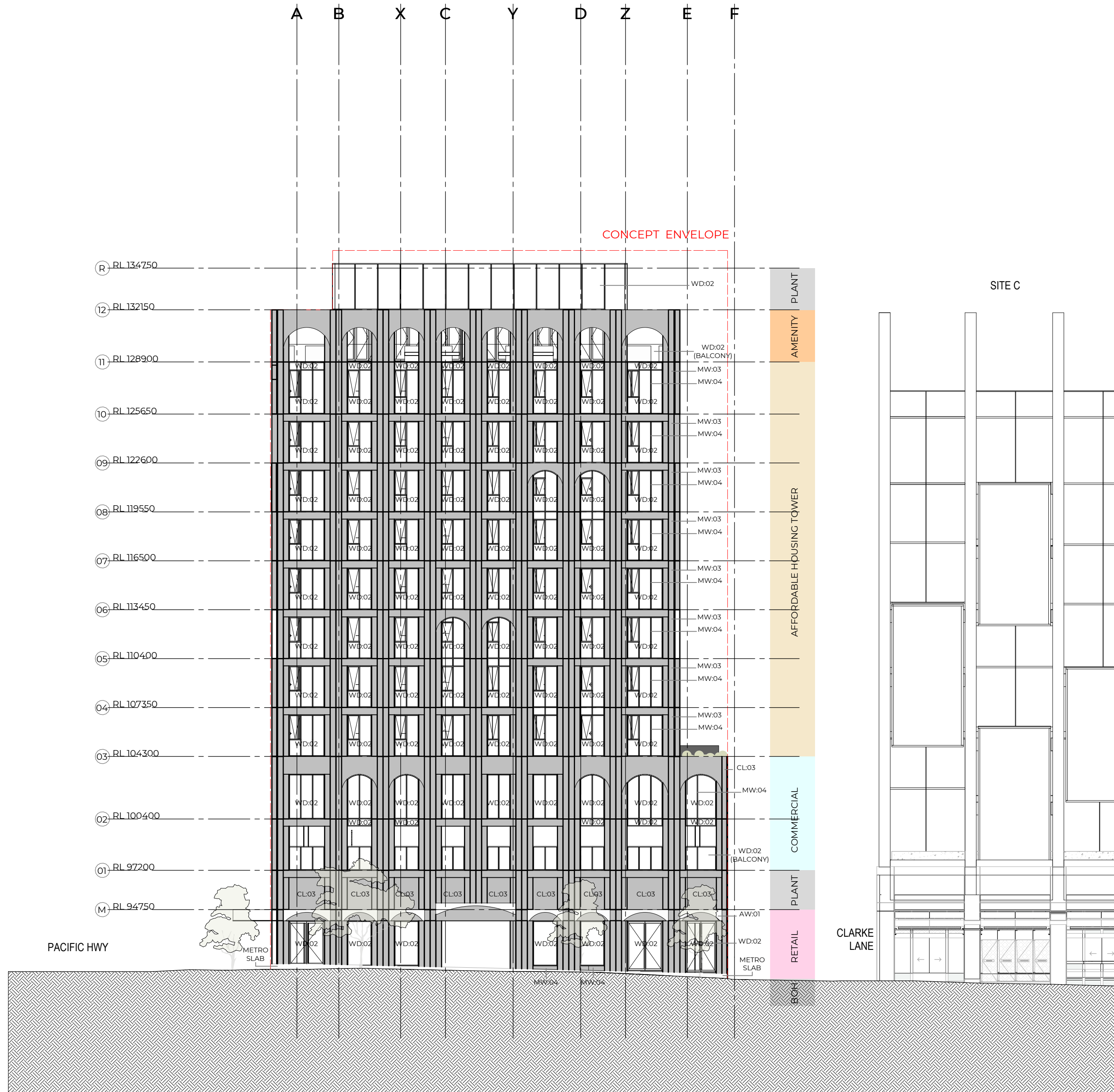
2 HUME STREET - PROPOSED ELEVATION SCALE 1 : 200
